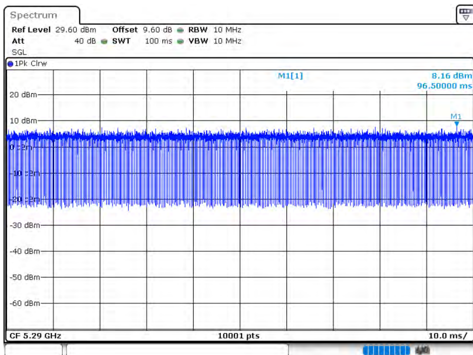
Duty Cycle NVNT 802.11ax80 5290MHz
