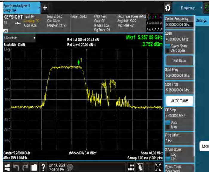
11AX20MIMO Ant2 5260 26Tone RU0
