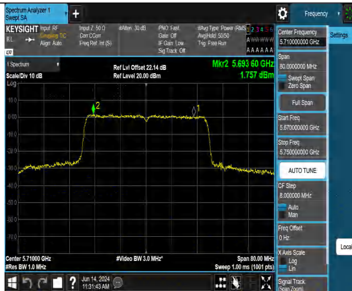
11BE40MIMO Ant3 5710 UNII-2C
