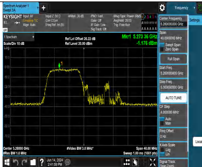
11AX20MIMO Ant3 5280 26Tone RU0
