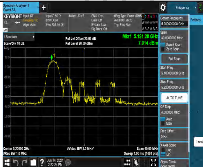
11AX20MIMO Ant2 5200 106Tone RU53
