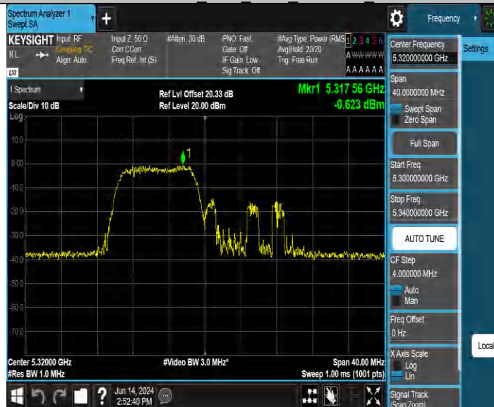
11AX20MIMO Ant3 5320 26Tone RU0
