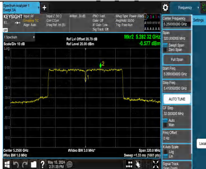
11BE160MIMO Ant2 5250 UNII-2A
