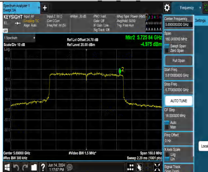
11BE80MIMO Ant2 5690 UNII-3
