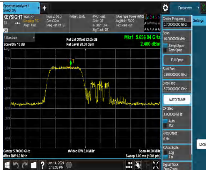
11AX20MIMO Ant2 5700 26Tone RU0
