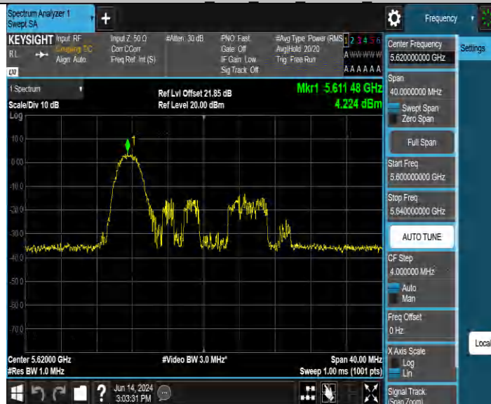
11AX20MIMO Ant2 5620 106Tone RU53
