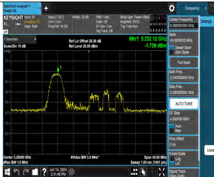
11AX20MIMO Ant2 5260 106Tone RU53
