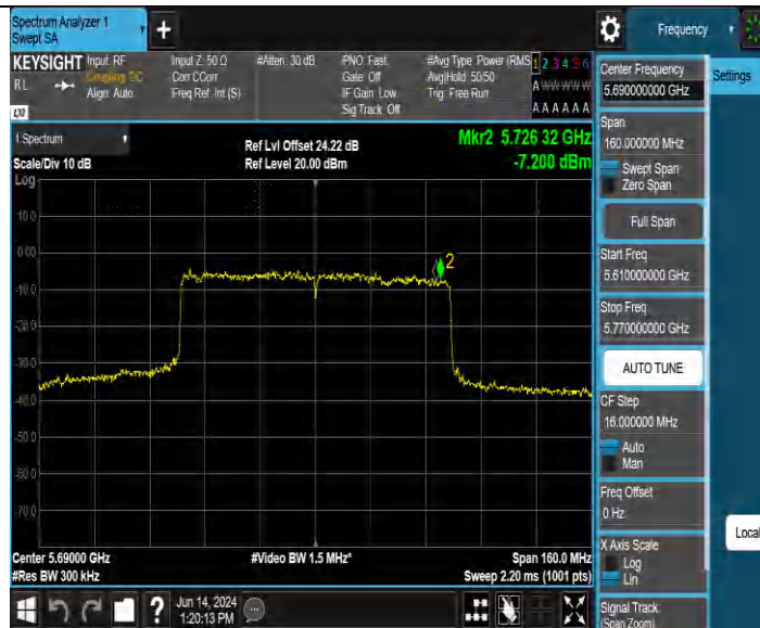
11BE80MIMO Ant3 5690 UNII-3
