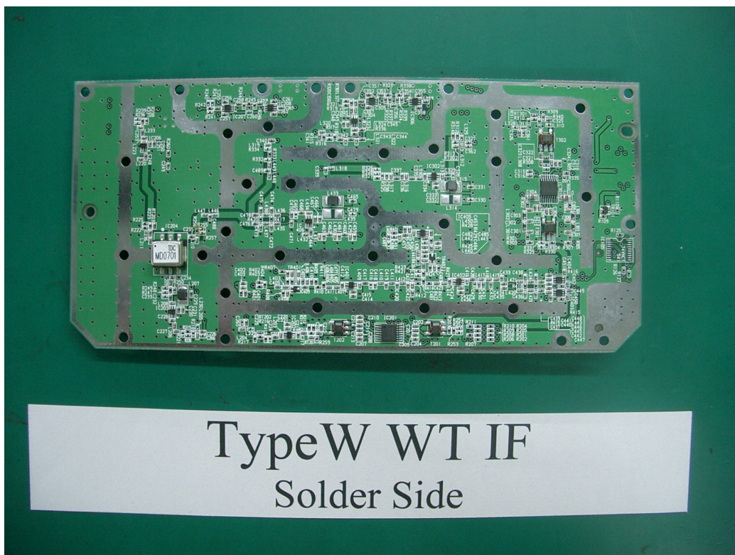
TypeW WT IF Solder Side Internal View
