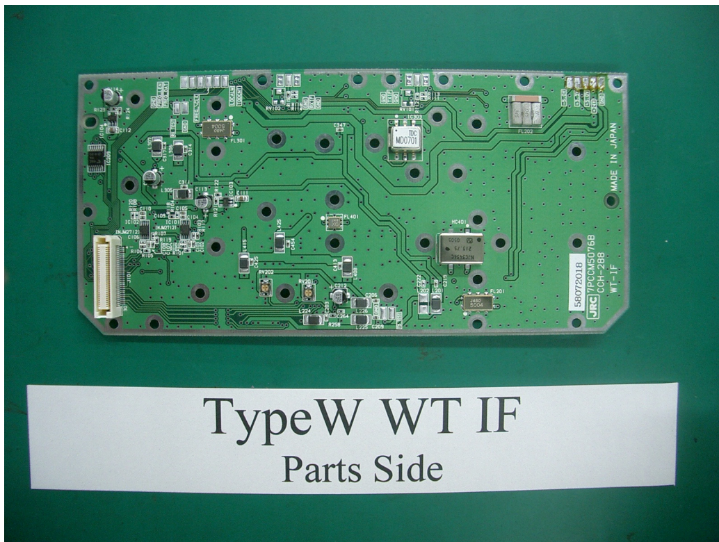
TypeW WT IF Parts Side Internal View
