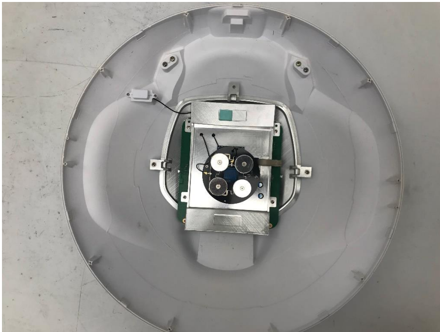
Photograph 2: Front View of DUT With Reflector Removed
