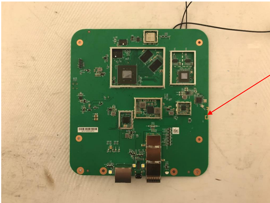
Photograph 12: Front View of the Main Printed Circuit Board – Cans Off
