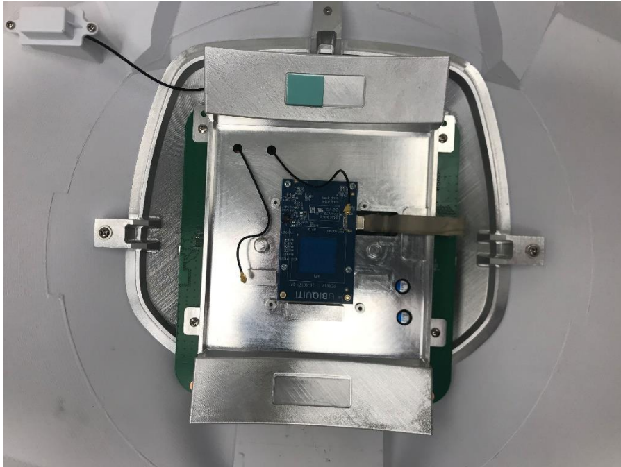
Photograph 3: Front View of DUT With 5 GHz Antenna Board Removed
