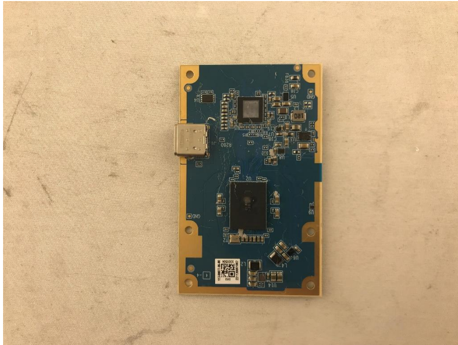
Photograph 7: Back View of 60 GHz Printed Circuit Board
