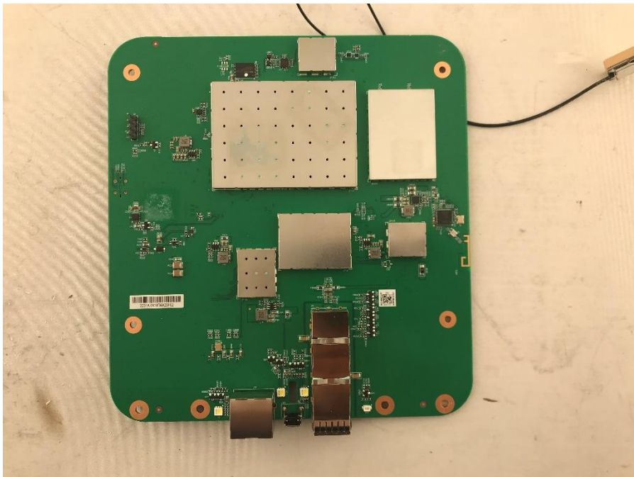
Photograph 10: Front View of the Main Printed Circuit Board – Cans On
