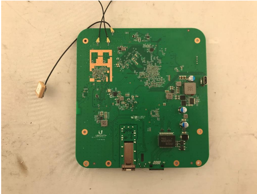
Photograph 11: Back View of the Main Printed Circuit Board
