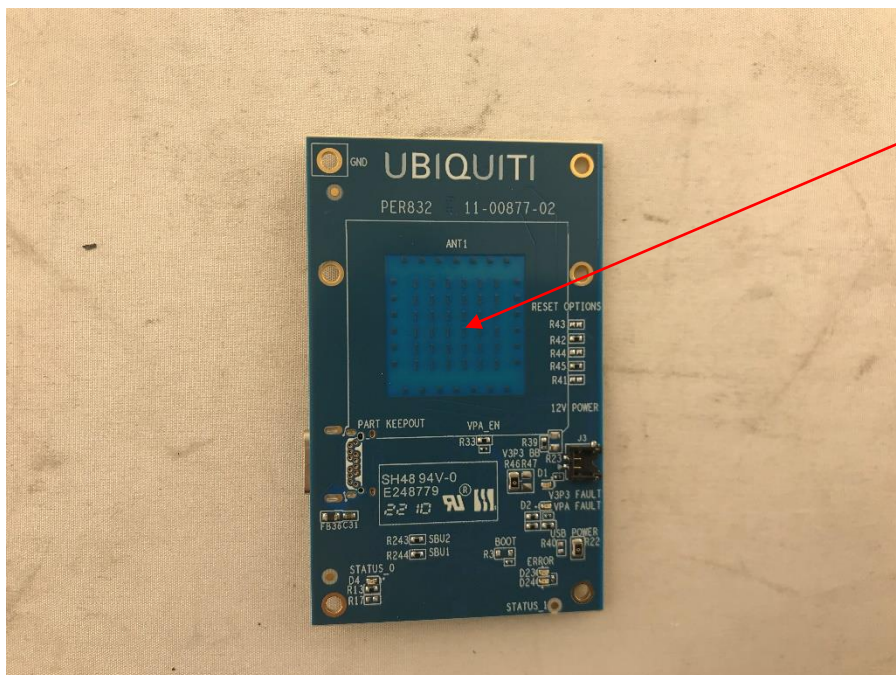
Photograph 6: Front View of 60 GHz Printed Circuit Board
