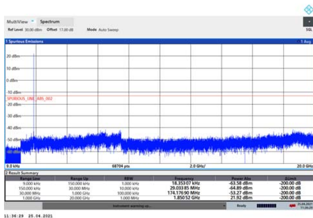
LTE eMTC Band 2 1.4MHz CH-Middle 9kHz~20GHz
