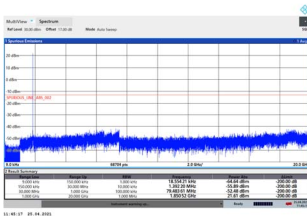
LTE eMTC Band 2 3MHz CH-Middle 9kHz~20GHz
