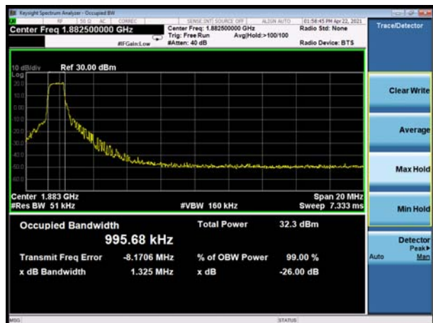
LTE eMTC Band 25 20MHz 16QAM CH-Middle
