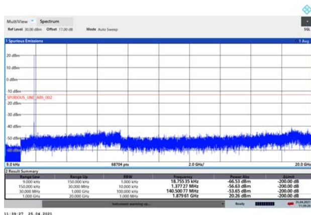
LTE eMTC Band 2 1.4MHz CH-High 9kHz~20GHz
