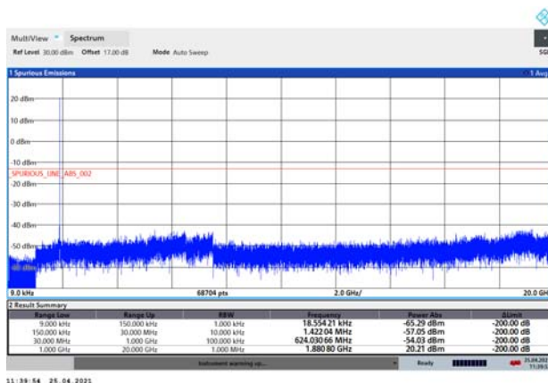
LTE eMTC Band 2 3MHz CH-High 9kHz~20GHz
