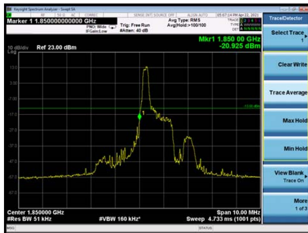
LTE eMTC Band 25 1.4MHz QPSK 100%RB CH-Low
