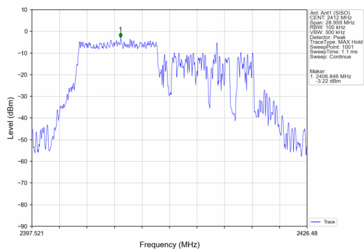
802.11ax(HEW20)_LCH_2412MHz_RU242_61_Ant1 (SISO)_NTNV
