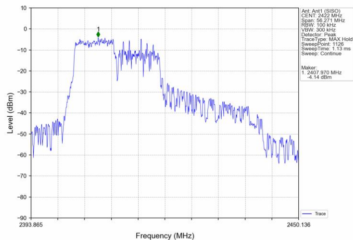
802.11ax(HEW40)_LCH_2422MHz_RU242_61_Ant1 (SISO)_NTNV
