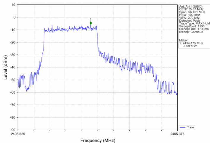
802.11ax(HEW40)_MCH_2437MHz_RU484_65_Ant1 (SISO)_NTNV
