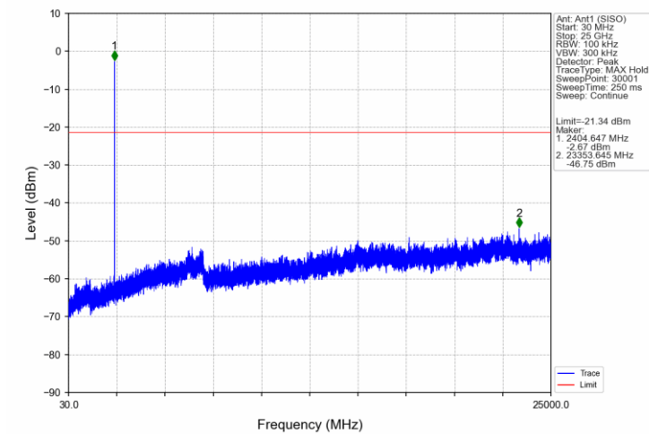
802.11ax(HEW20)_LCH_2412MHz_RU106_53_Ant1 (SISO)_NTNV
