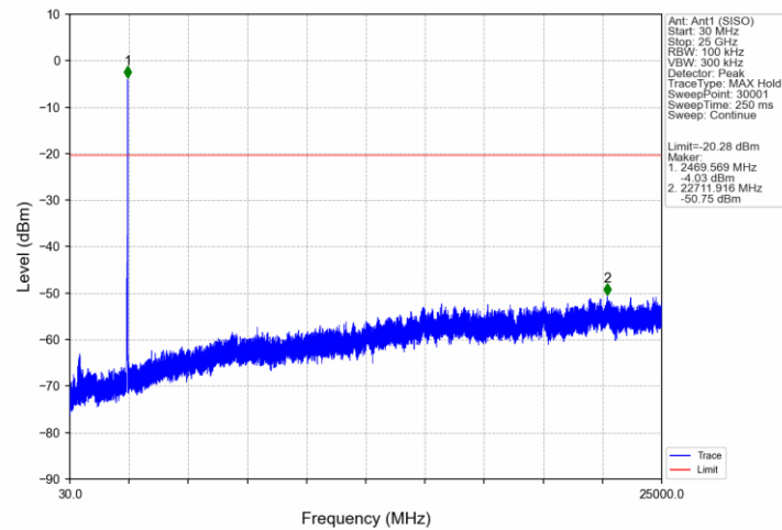
802.11ax(HEW40)_HCH_2452MHz_RU52_44_Ant1 (SISO)_NTNV
