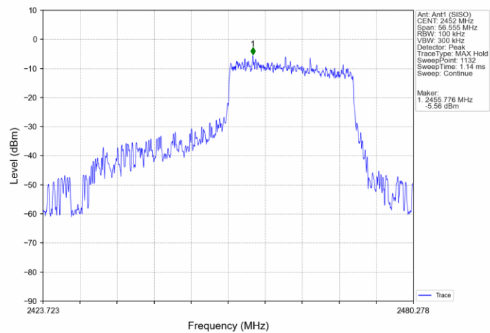
802.11ax(HEW40)_HCH_2452MHz_RU484_65_Ant1 (SISO)_NTNV
