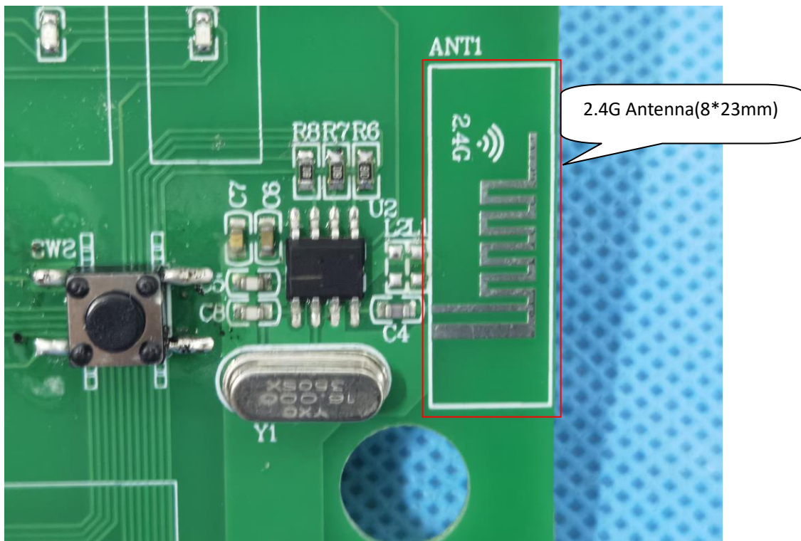
INTERNAL VIEW OF EUT (FIGURE 4)
