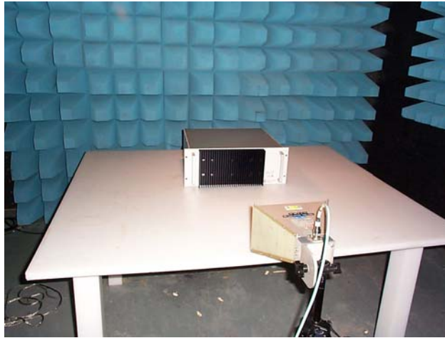
RADIATED TEST SETUP
