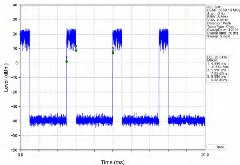
n78d_30kHz_MIMO_NTNV_10MHz_CP-OFDM_QPSK_3555MHz_Edge_1RB_Right
