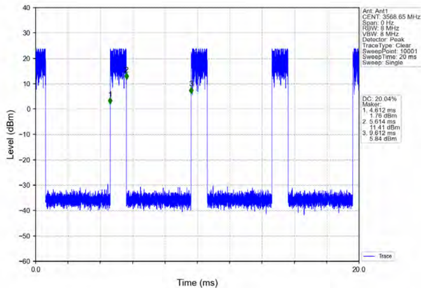
n78d_30kHz_MIMO_NTNV_20MHz_CP-OFDM_16_QAM_3560.01MHz_Inner_1RB_Right
