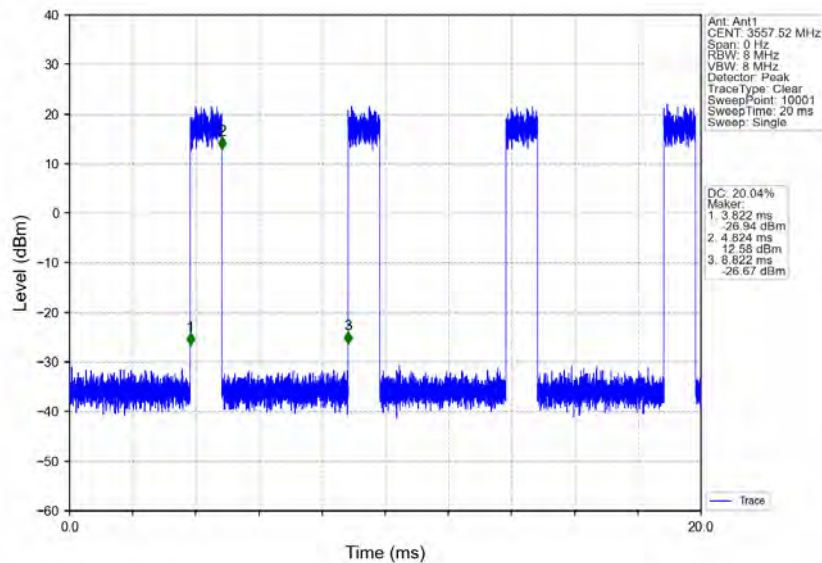
n78d_30kHz_MIMO_NTNV_15MHz_CP-OFDM_256_QAM_3557.52MHz_Inner_Full
