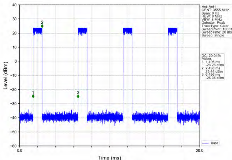
n78d_30kHz_MIMO_NTNV_10MHz_CP-OFDM_QPSK_3555MHz_Inner_Full
