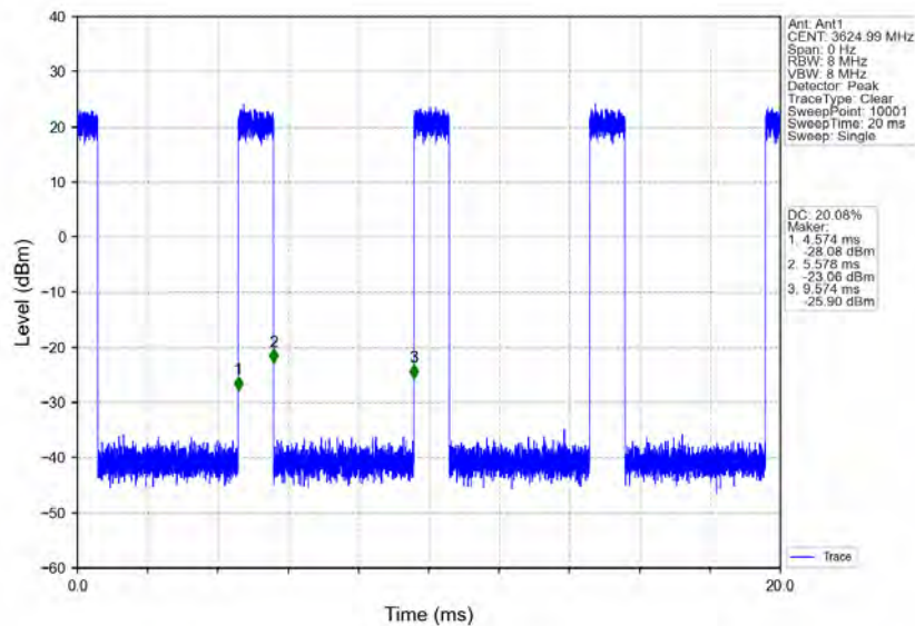
n78d_30kHz_MIMO_NTNV_15MHz_CP-OFDM_16_QAM_3624.99MHz_Inner_Full
