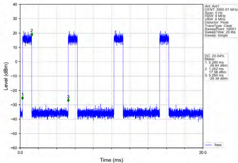
n78d_30kHz_MIMO_NTNV_20MHz_CP-OFDM_256_QAM_3560.01MHz_Inner_Full
