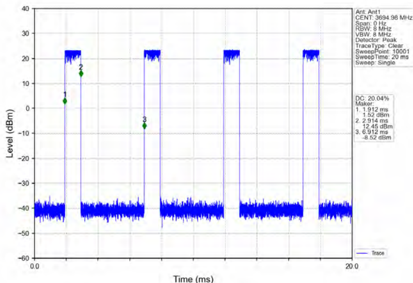
n78d_30kHz_MIMO_NTNV_10MHz_CP-OFDM_QPSK_3694.98MHz_Inner_Full
