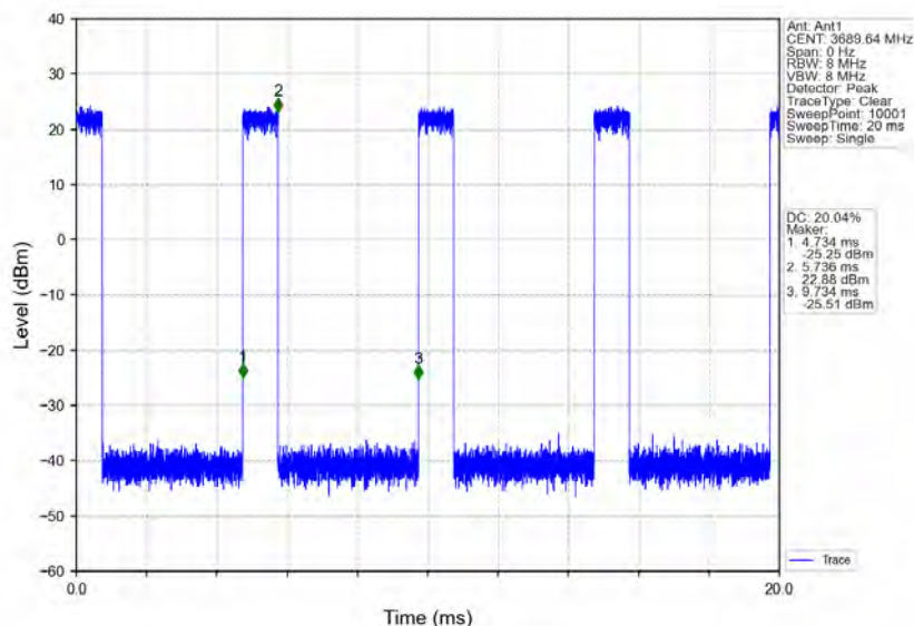
n78d_30kHz_MIMO_NTNV_20MHz_CP-OFDM_QPSK_3690MHz_Inner_Full
