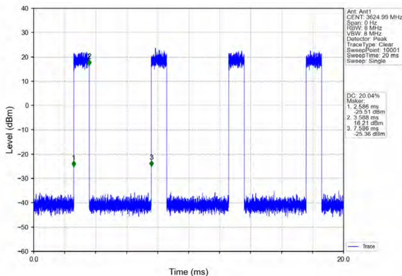
n78d_30kHz_MIMO_NTNV_20MHz_CP-OFDM_64_QAM_3624.99MHz_Inner_Full
