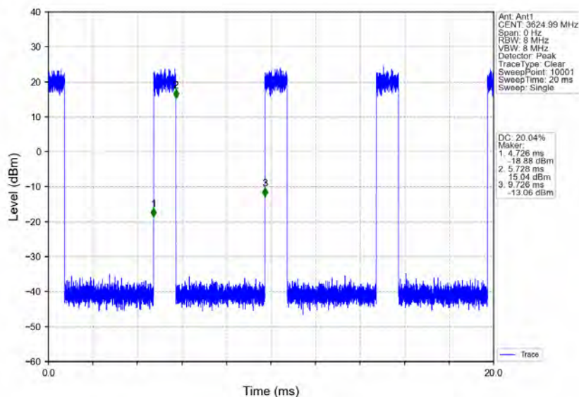
n78d_30kHz_MIMO_NTNV_15MHz_CP-OFDM_64_QAM_3624.99MHz_Inner_Full
