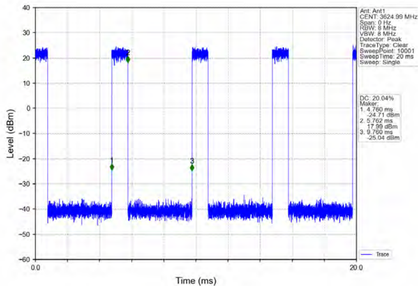
n78d_30kHz_MIMO_NTNV_10MHz_CP-OFDM_64_QAM_3624.99MHz_Inner_Full
