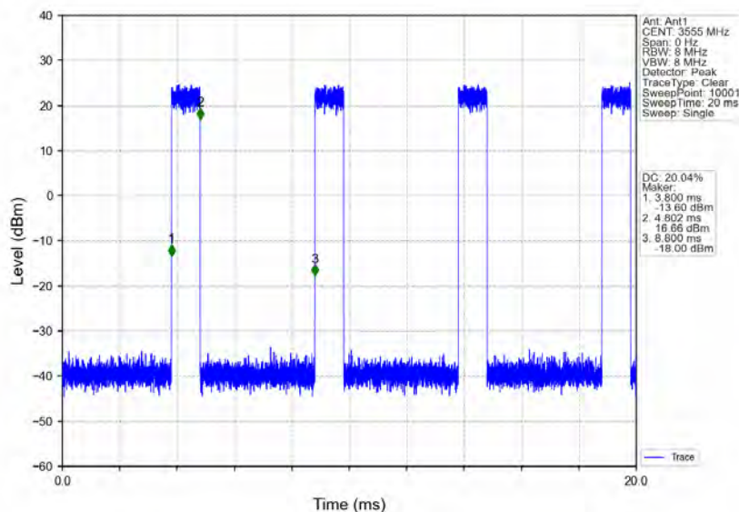
n78d_30kHz_MIMO_NTNV_10MHz_CP-OFDM_64_QAM_3555MHz_Inner_Full
