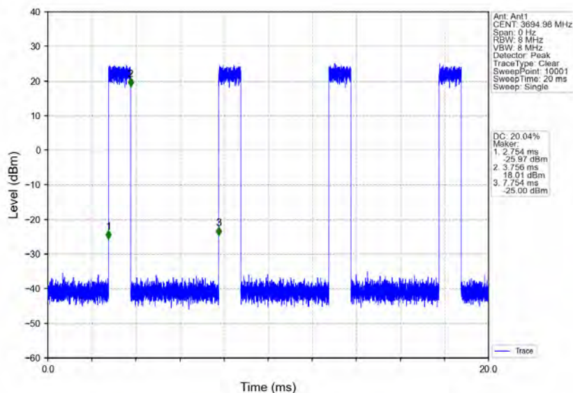
n78d_30kHz_MIMO_NTNV_10MHz_CP-OFDM_64_QAM_3694.98MHz_Inner_Full
