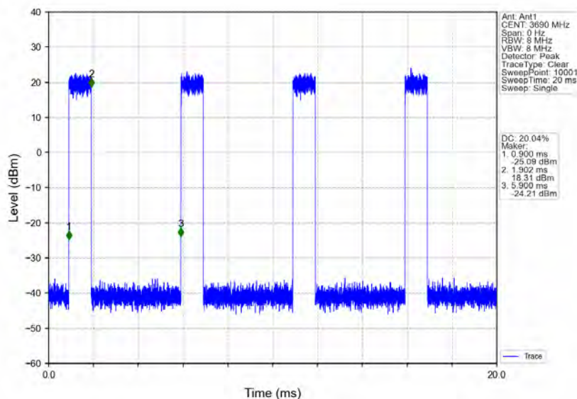
n78d_30kHz_MIMO_NTNV_20MHz_CP-OFDM_QPSK_3690MHz_Inner_Full
