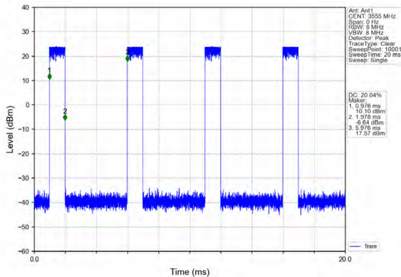
n78d_30kHz_MIMO_NTNV_10MHz_CP-OFDM_16_QAM_3555MHz_Inner_Full
