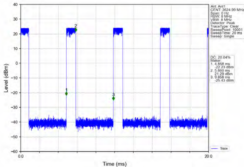
n78d_30kHz_MIMO_NTNV_10MHz_CP-OFDM_QPSK_3624.99MHz_Inner_Full
