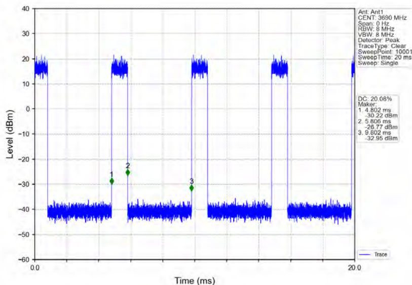
n78d_30kHz_MIMO_NTNV_20MHz_CP-OFDM_256_QAM_3690MHz_Inner_Full
