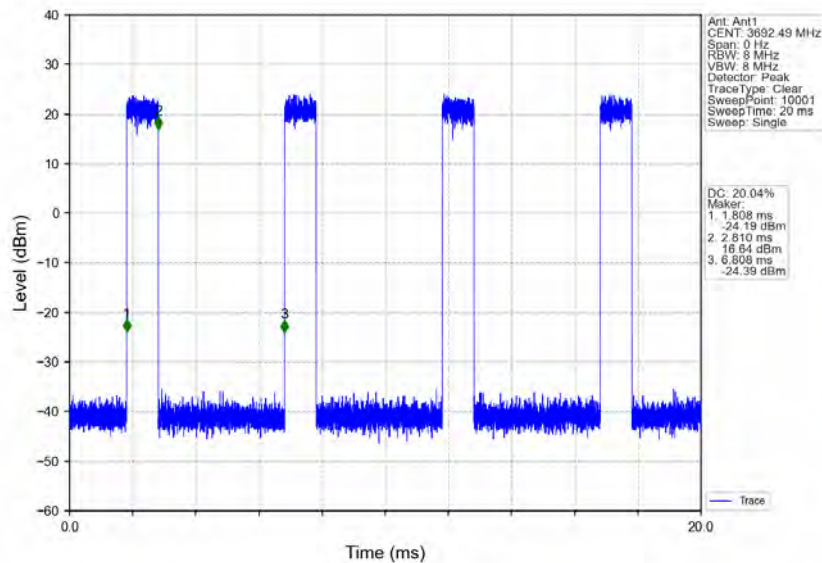
n78d_30kHz_MIMO_NTNV_15MHz_CP-OFDM_16_QAM_3692.49MHz_Inner_Full
