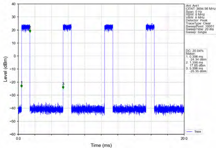
n78d_30kHz_MIMO_NTNV_10MHz_CP-OFDM_16_QAM_3694.98MHz_Inner_Full
