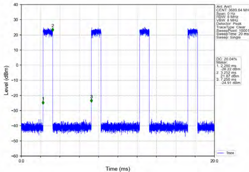
n78d_30kHz_MIMO_NTNV_20MHz_CP-OFDM_16_QAM_3690MHz_Inner_Full
