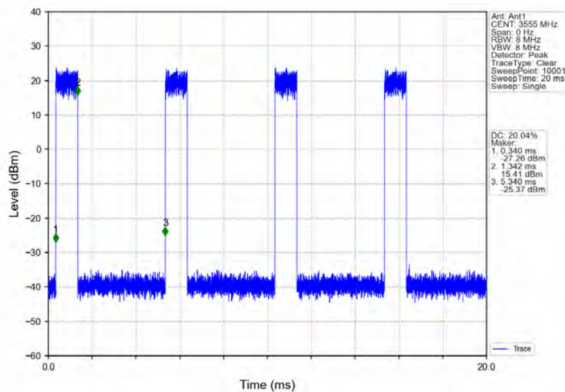
n78d_30kHz_MIMO_NTNV_10MHz_CP-OFDM_256_QAM_3555MHz_Inner_Full
