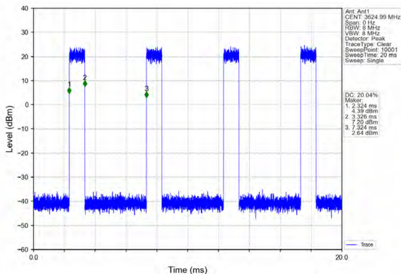
n78d_30kHz_MIMO_NTNV_15MHz_CP-OFDM_QPSK_3624.99MHz_Inner_Full
