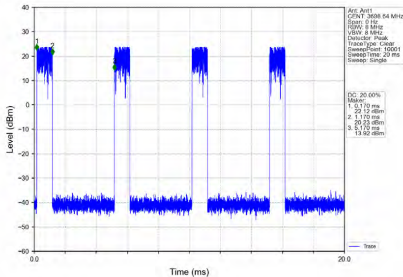
n78d_30kHz_MIMO_NTNV_20MHz_CP-OFDM QPSK_3690MHz_Inner_1RB_Right
