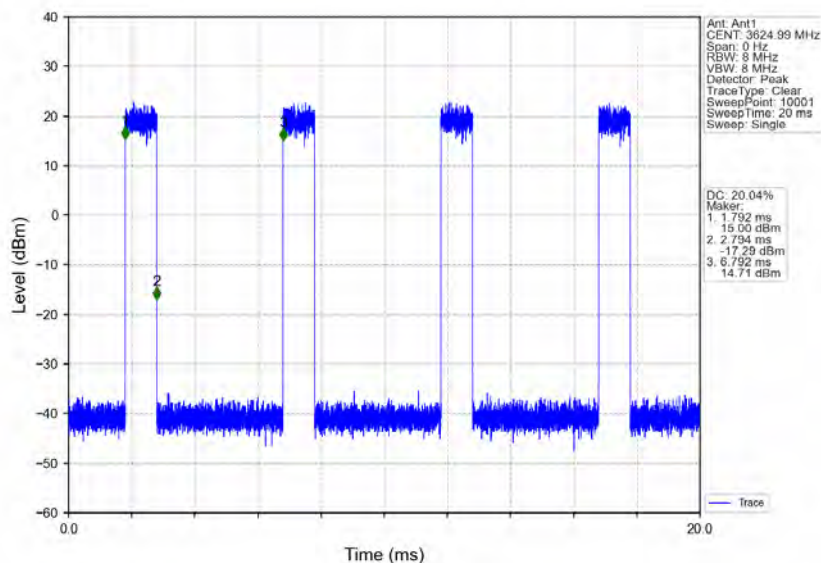
n78d_30kHz_MIMO_NTNV_20MHz_CP-OFDM_16_QAM_3624.99MHz_Inner_Full
