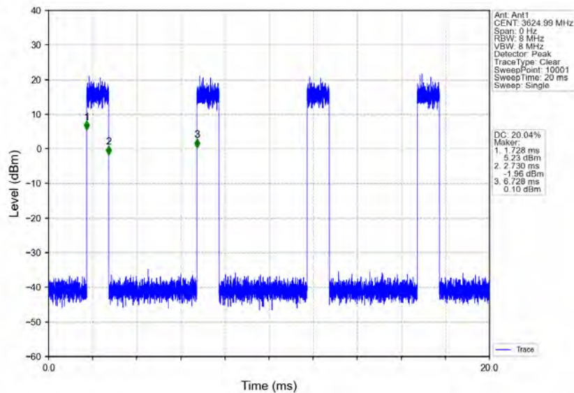
n78d_30kHz_MIMO_NTNV_20MHz_CP-OFDM_256_QAM_3624.99MHz_Inner_Full
