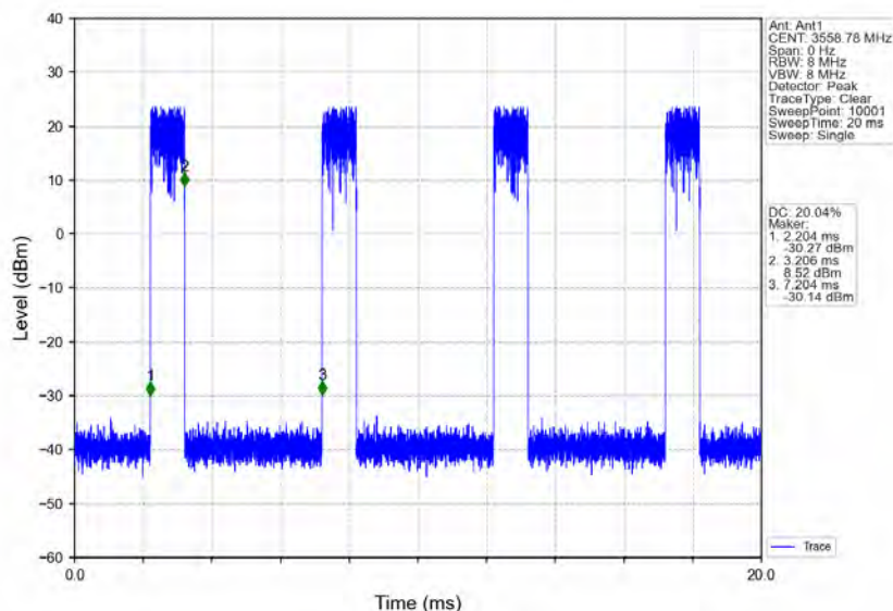
n78d_30kHz_MIMO_NTNV_10MHz_CP-OFDM 64 QAM_3555MHz_Inner_1RB_Right
