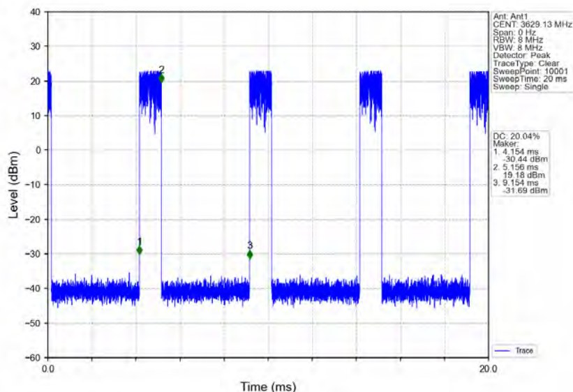
n78d_30kHz_MIMO_NTNV_10MHz_CP-OFDM_QPSK_3624.99MHz_Edge_1RB_Right
