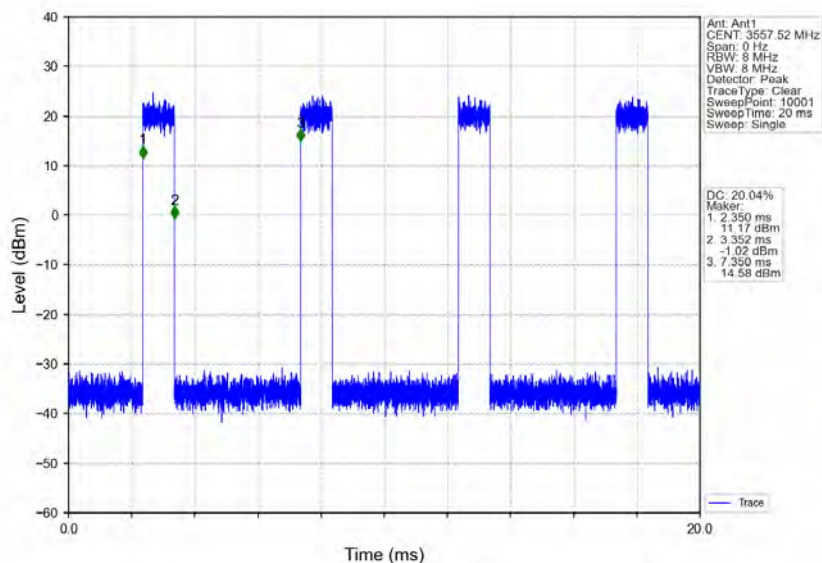
n78d_30kHz_MIMO_NTNV_15MHz_CP-OFDM_64_QAM_3557.52MHz_Inner_Full
