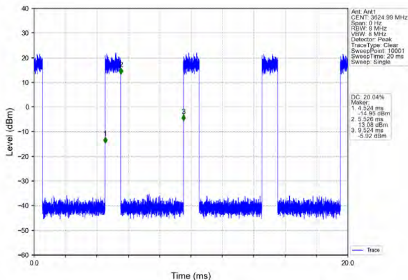
n78d_30kHz_MIMO_NTNV_15MHz_CP-OFDM_256_QAM_3624.99MHz_Inner_Full
