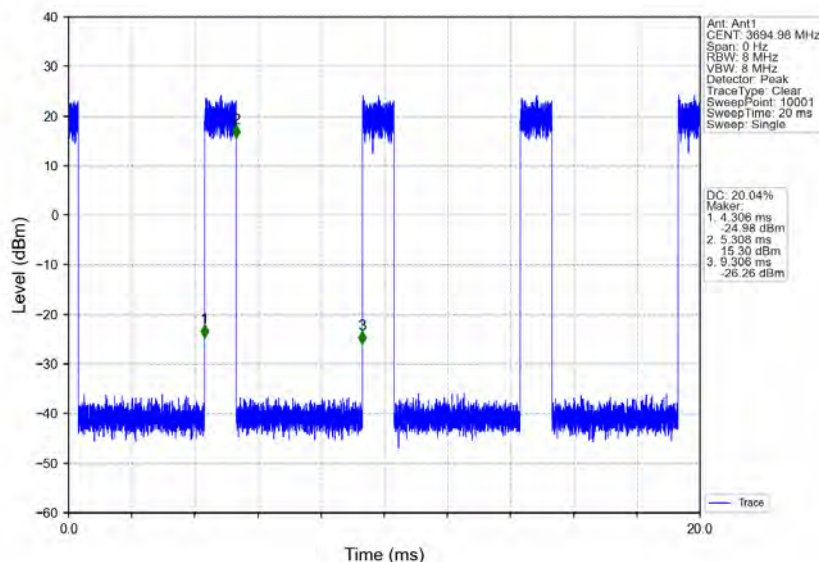
n78d_30kHz_MIMO_NTNV_10MHz_CP-OFDM_256_QAM_3694.98MHz_Inner_Full
