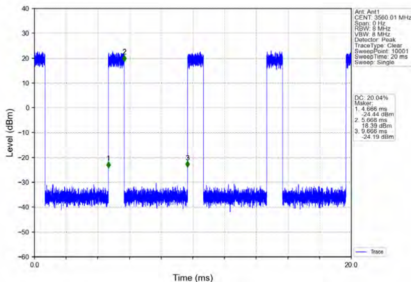
n78d_30kHz_MIMO_NTNV_20MHz_CP-OFDM_QPSK_3560.01MHz_Inner_Full
