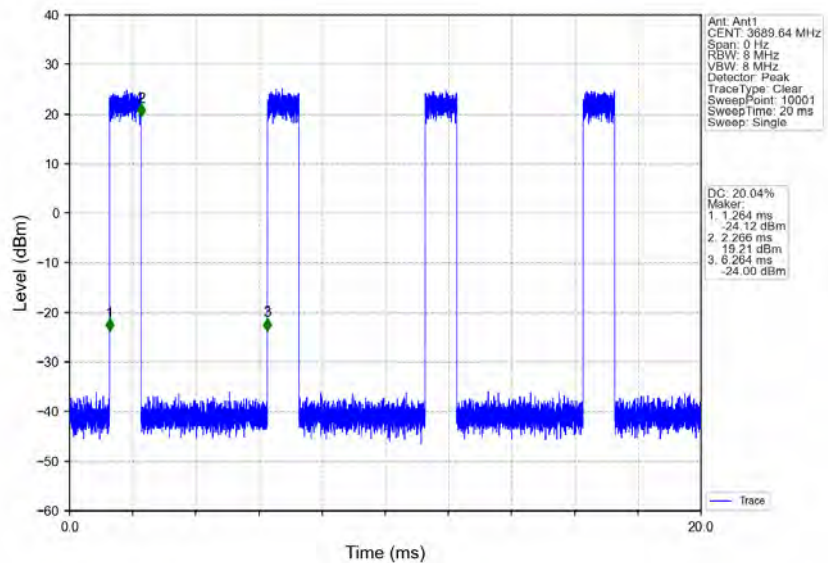
n78d_30kHz_MIMO_NTNV_20MHz_CP-OFDM_64_QAM_3690MHz_Inner_Full
