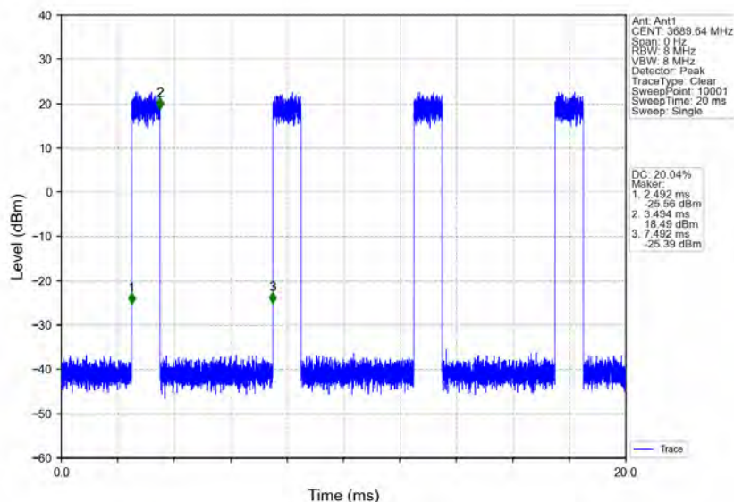
n78d_30kHz_MIMO_NTNV_20MHz_CP-OFDM_256_QAM_3690MHz_Inner_Full
