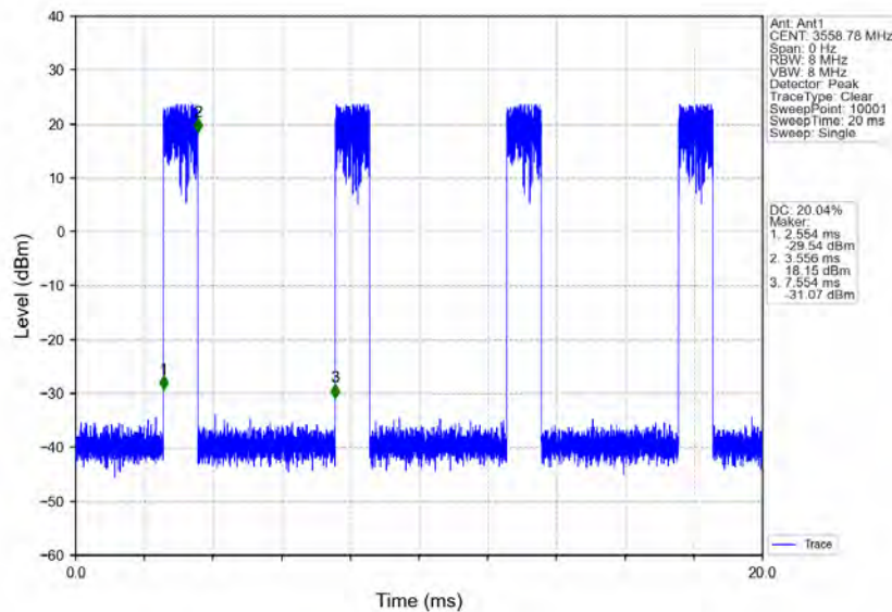
n78d_30kHz_MIMO_NTNV_10MHz_CP-OFDM_QPSK_3555MHz_Inner_1RB_Right
