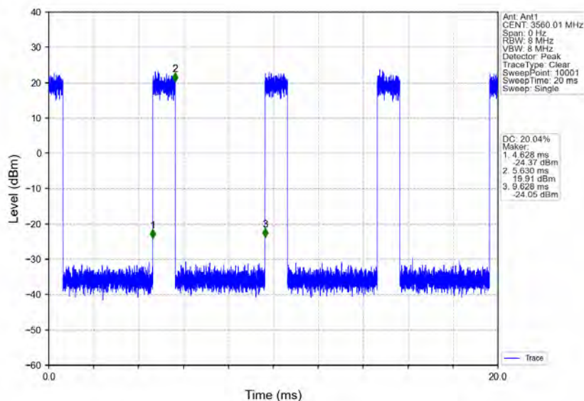
n78d_30kHz_MIMO_NTNV_20MHz_CP-OFDM_16_QAM_3560.01MHz_Inner_Full
