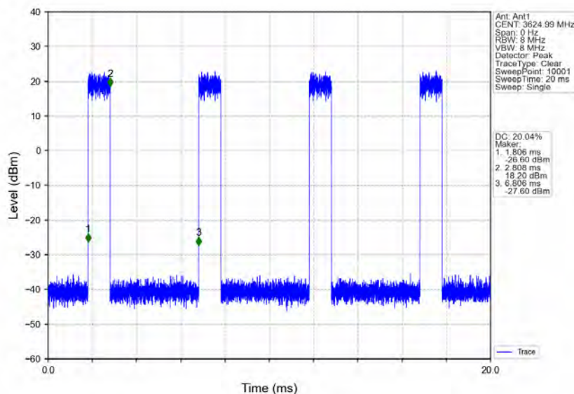
n78d_30kHz_MIMO_NTNV_10MHz_CP-OFDM_256_QAM_3624.99MHz_Inner_Full
