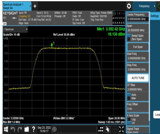
Band48-10MHz-64QAM-55290-E-TM3.1
