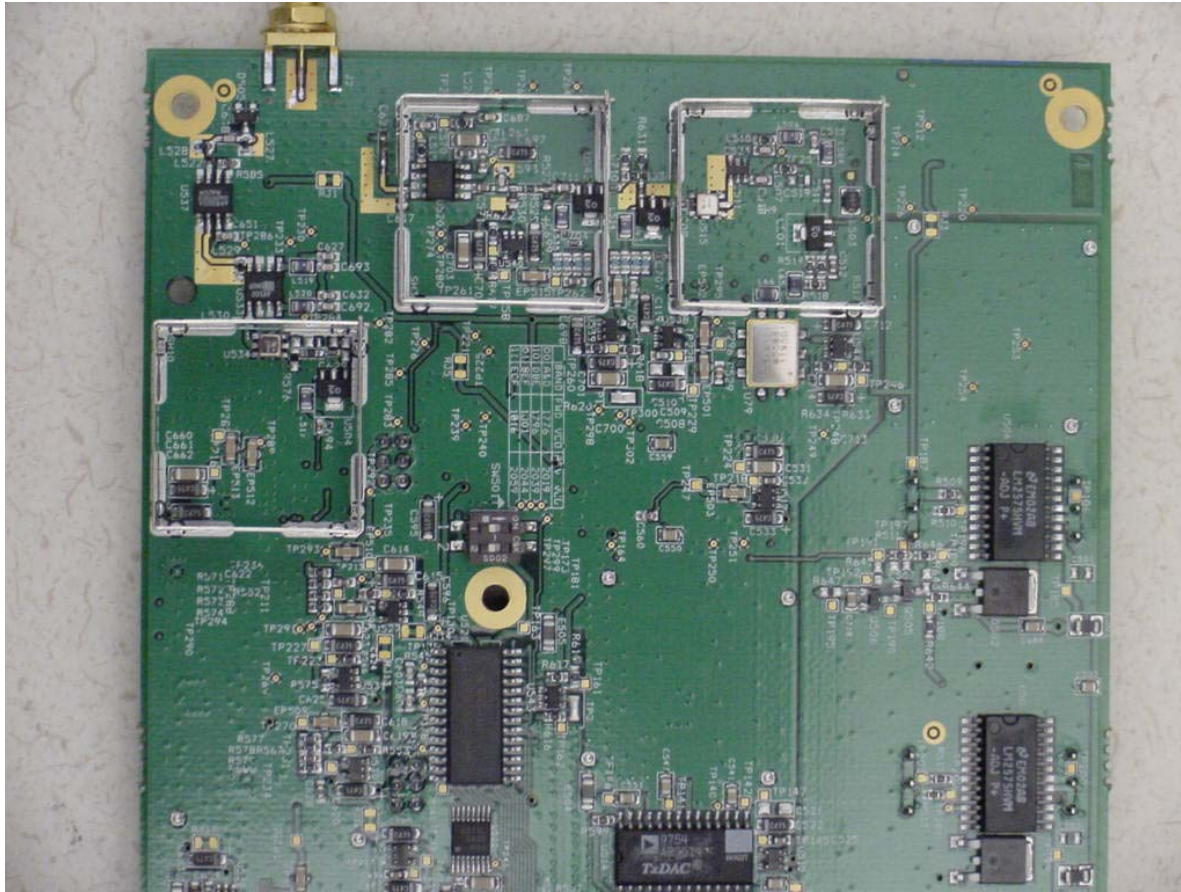
Digivance ICS 1900 MHz Digital Remote Unit PCB – Bottom View 1
