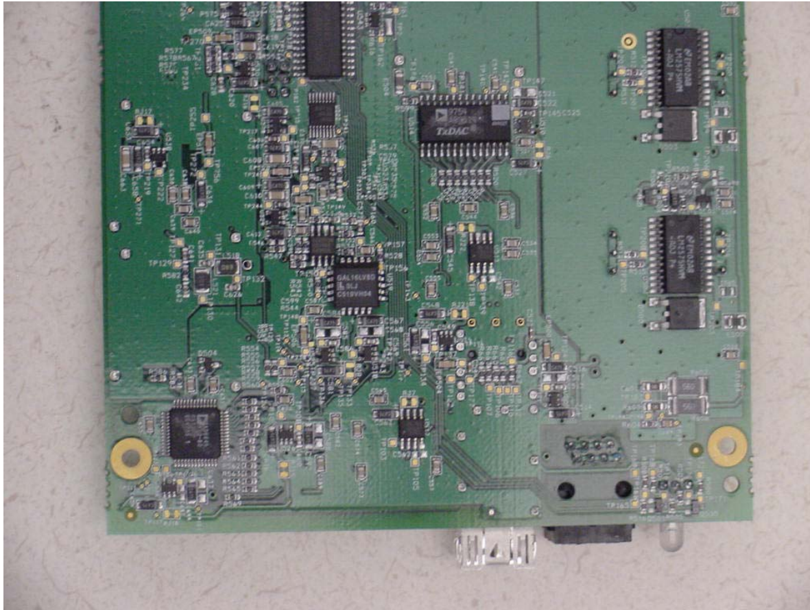
Digivance ICS 1900 MHz Digital Remote Unit PCB – Bottom View 2
