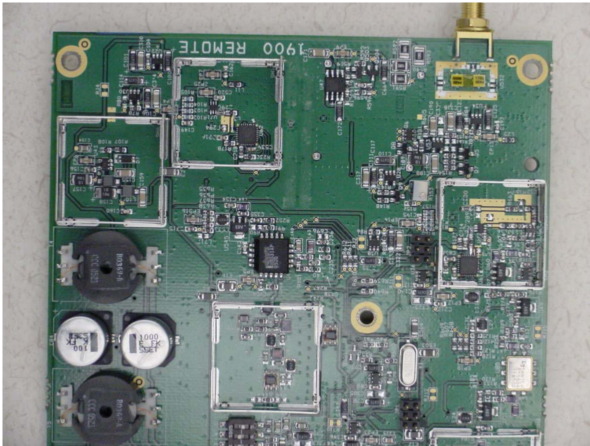
Digivance ICS 1900 MHz Digital Remote Unit PCB – Top View 1
