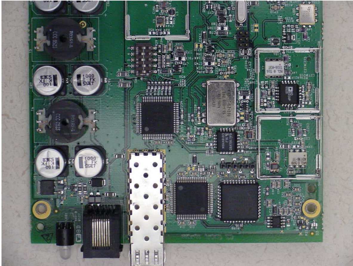
Digivance ICS 1900 MHz Digital Remote Unit PCB – Top View 2
