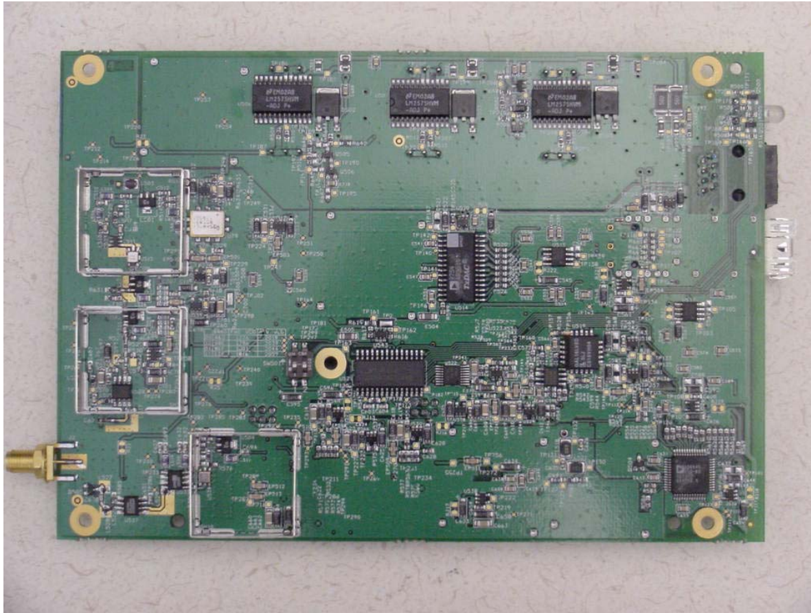
Digivance ICS 1900 MHz Digital Remote Unit PCB – Bottom View
