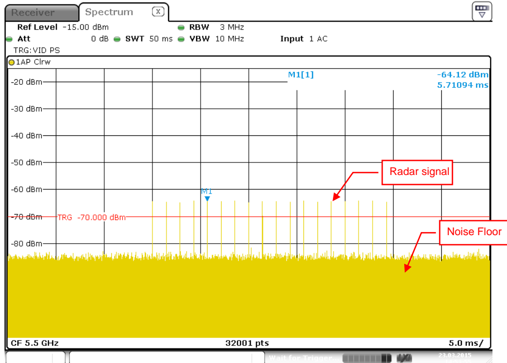
Radar Signal 0
