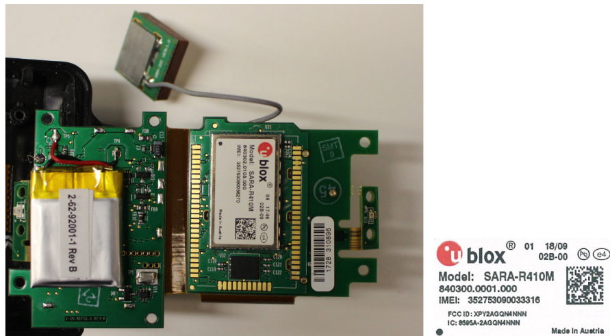
Pic 2 – BI LOC8 LTE Nested Board, back side (Left), UBIOX Label from FCC website (Right)
