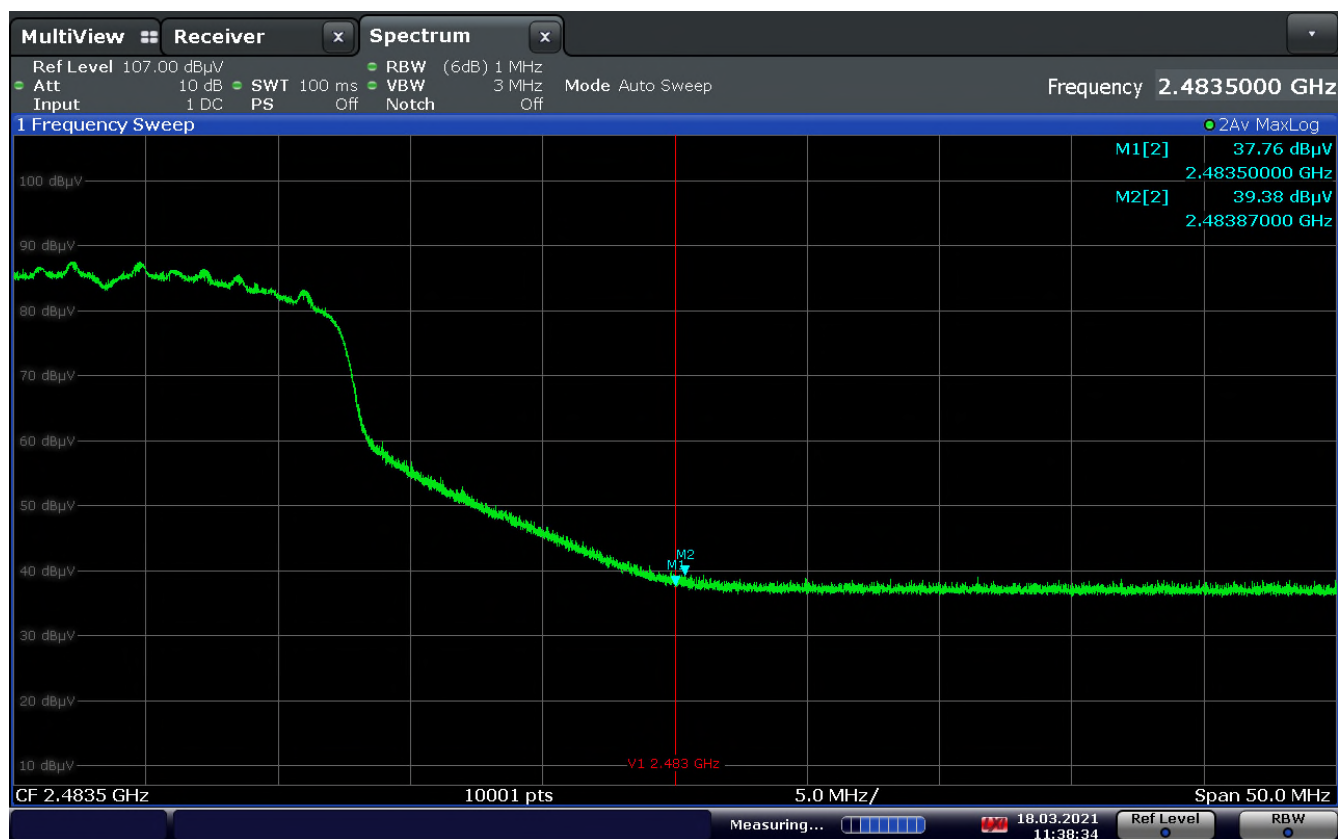
Figure 2-27 – Band-edge, 802.11n HT20 High Channel – Average
