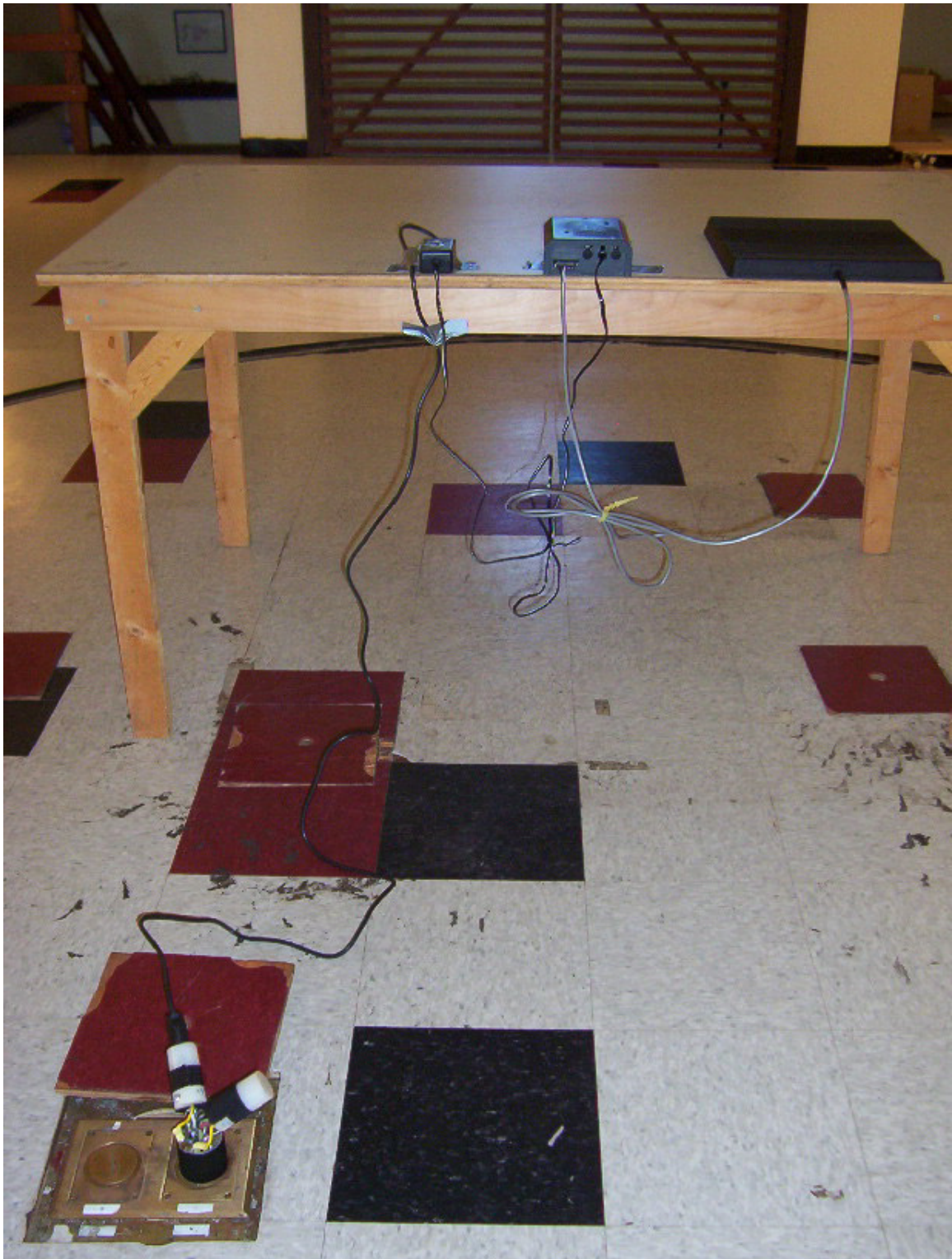
Checkpoint Systems, Inc.: CP9-2 EMI Test Setup Photo (Rear View)
