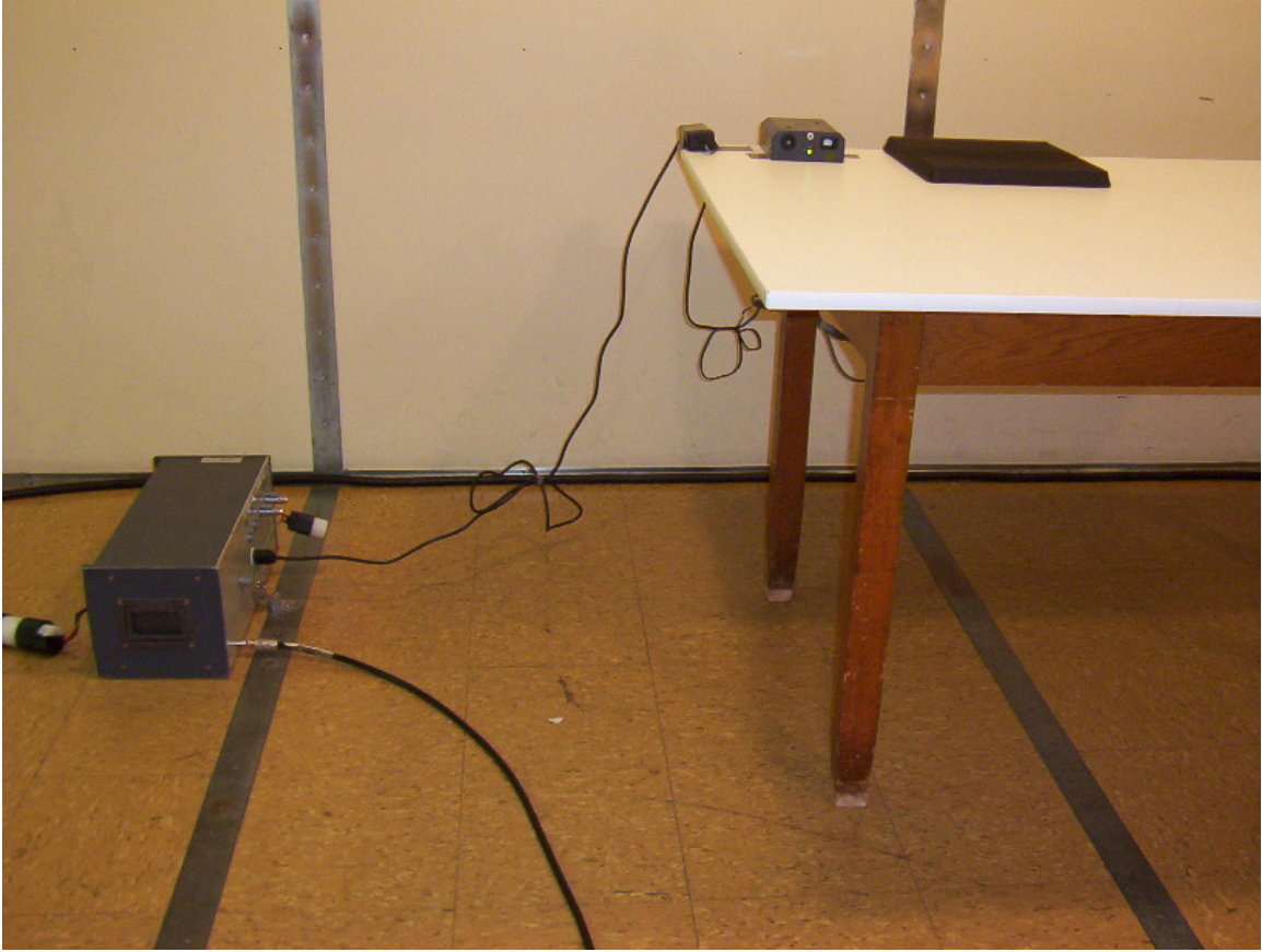
Checkpoint Systems, Inc.: CP9-2 Conducted Emissions Test Setup Photo
