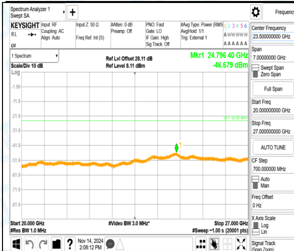
Band41_10MHz_16QAM_41190_1RB#0_0.15~30_0.15~30
