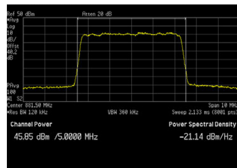
LTE5_Middle Channel_64QAM_Average
