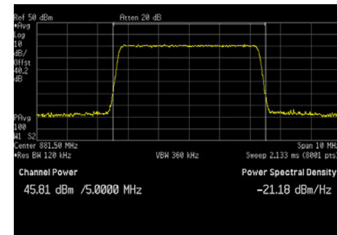
LTE5_Middle Channel_16QAM_Average
