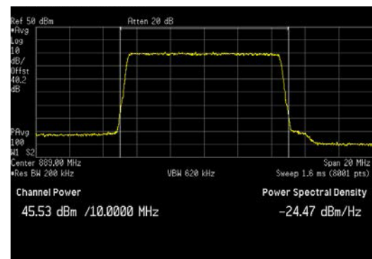
LTE10_Top Channel_Average
