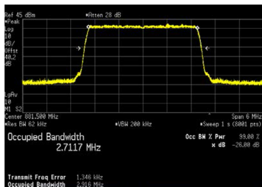
LTE3_64QAM
