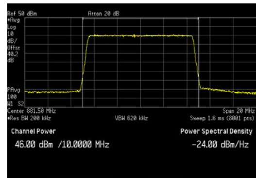
LTE10_Middle Channel_Average
