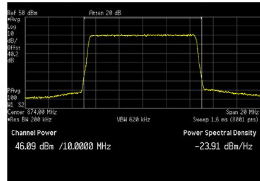
LTE10_Bottom Channel_Average
