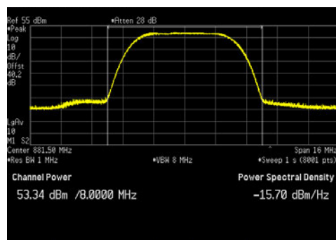
LTE5_Middle Channel_256QAM_Peak
