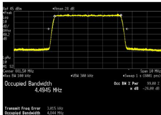
LTE5_64QAM
