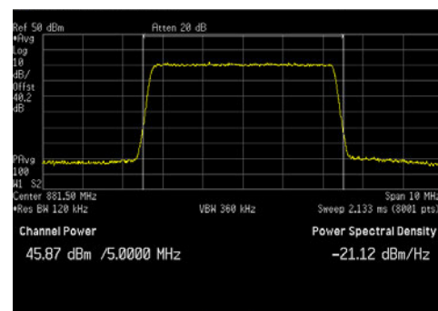
LTE5_Middle Channel_256QAM_Average
