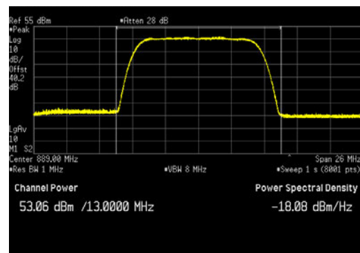
LTE10_Top Channel_Peak
