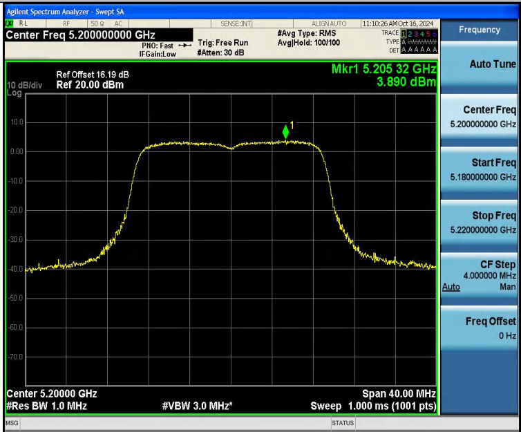
11AC20SISO-Ant1-5200-PASS
