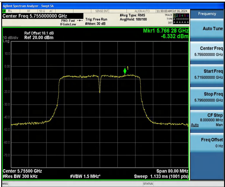
11AC40SISO-Ant1-5755-PASS
