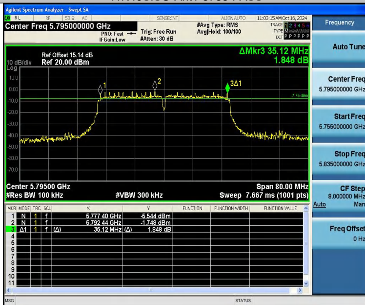
11N40SISO-Ant1-5795-PASS
