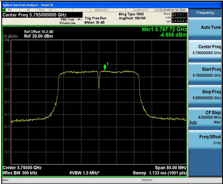
11AC40SISO-Ant1-5795-PASS
