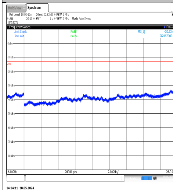
NTNV-N77-3700-3980-PC3-30-20-M-DFT-QPSK- Edge_1RB_Left-6000-26000-Ant1-PASS
