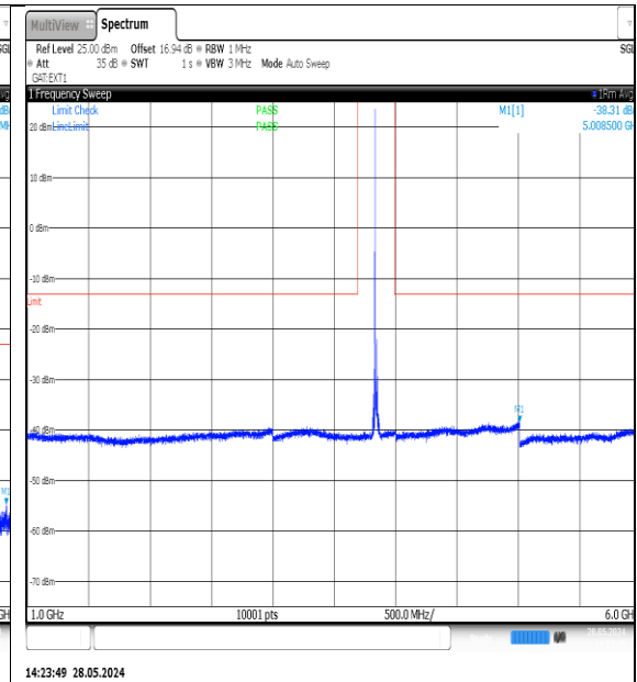
NTNV-N77-3700-3980-PC3-30-20-M-DFT-QPSK- Edge_1RB_Left-1000-6000-Ant1-PASS
