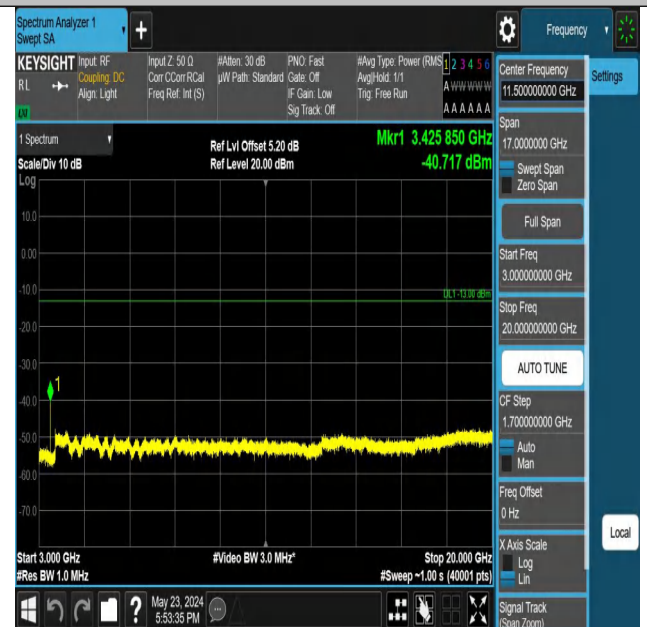
Band4_3MHz_QPSK_19965_1RB#14_3000~20000_3000~20000
