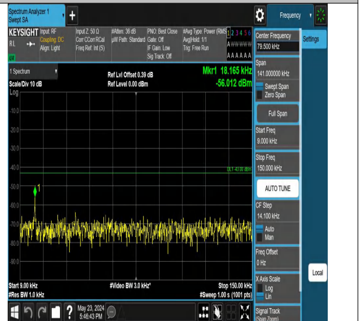
Band4_1.4MHz_QPSK_20175_1RB#5_0.009~0.15_0.009~0.15
