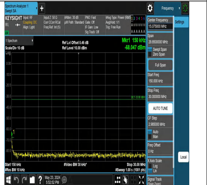
Band4_3MHz_QPSK_19965_1RB#0_0.15~30_0.15~30
