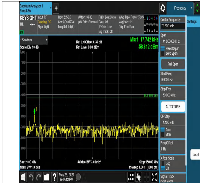
Band4_1.4MHz_QPSK_20393_1RB#0_0.009~0.15_0.009~0.15
