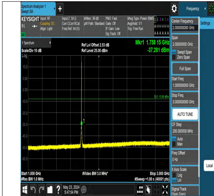
Band4_1.4MHz_QPSK_20393_1RB#5_1000~3000_1000~3000
