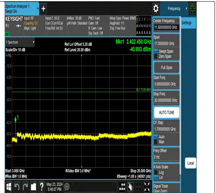
Band4_1.4MHz_QPSK_19957_1RB#5_3000~20000_3000~20000
