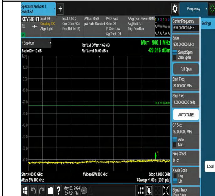
Band4_1.4MHz_QPSK_20393_1RB#0_30~1000_30~1000
