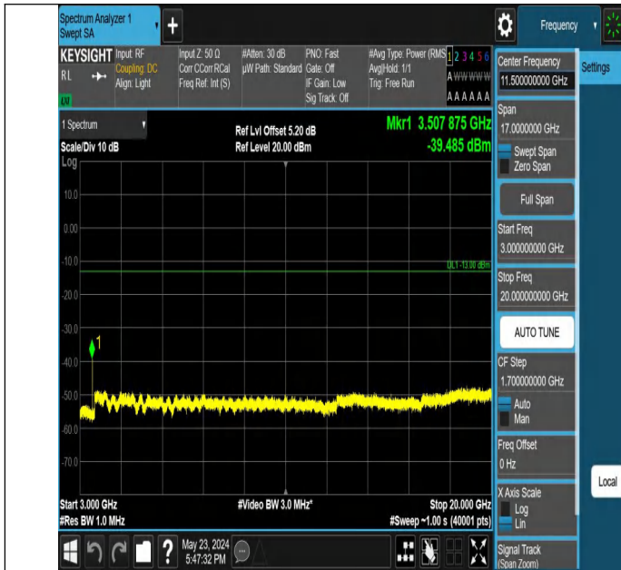
Band4_1.4MHz_QPSK_20393_1RB#0_3000~20000_3000~20000
