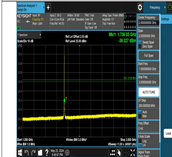
Band4_1.4MHz_QPSK_20175_1RB#5_1000~3000_1000~3000
