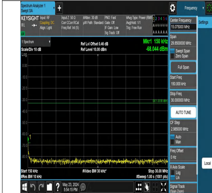
Band4_3MHz_QPSK_20175_1RB#14_0.15~30_0.15~30
