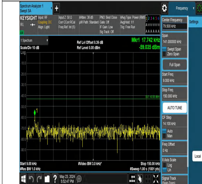
Band4_3MHz_QPSK_19965_1RB#0_0.009~0.15_0.009~0.15
