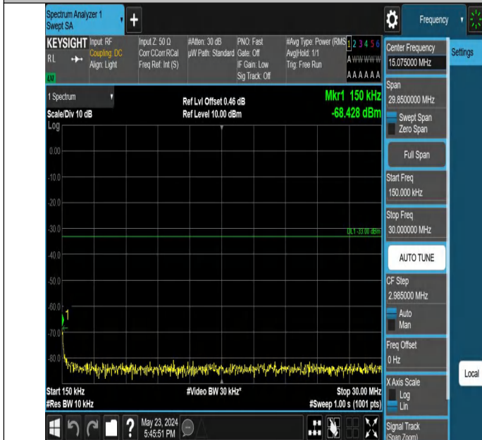
Band4_1.4MHz_QPSK_19957_1RB#5_0.15~30_0.15~30
