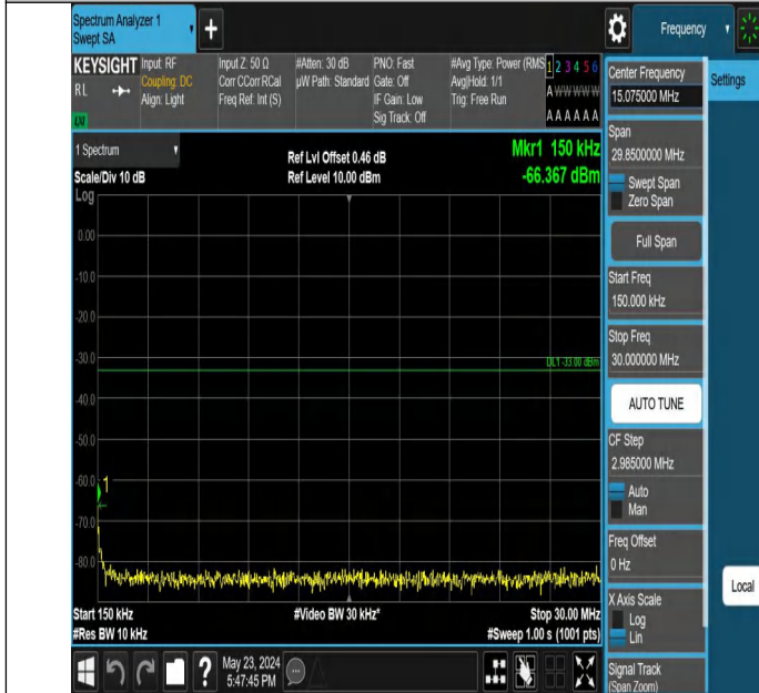
Band4_1.4MHz_QPSK_20393_1RB#5_0.15~30_0.15~30
