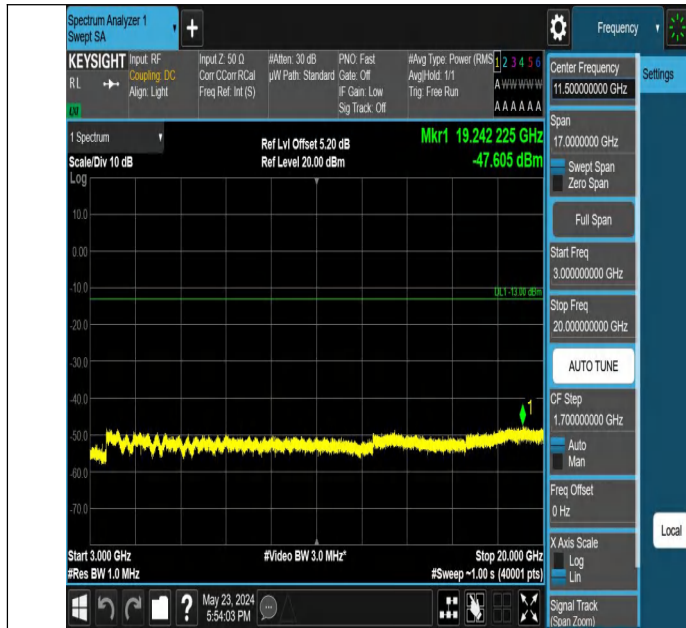
Band3_3MHz_QPSK_20175_1RB#0_3000~20000_3000~20000
