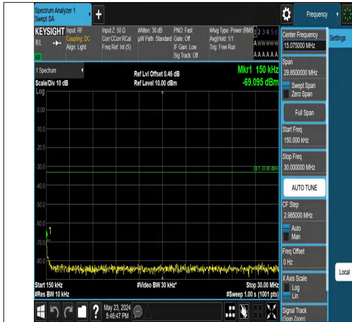
Band4_1.4MHz_QPSK_20175_1RB#5_0.15~30_0.15~30
