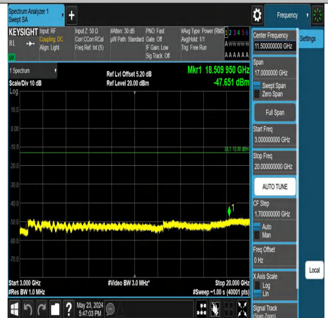
Band4_1.4MHz_QPSK_20175_1RB#5_3000~20000_3000~20000
