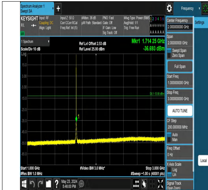
Band4_1.4MHz_QPSK_19957_1RB#5_1000~3000_1000~3000
