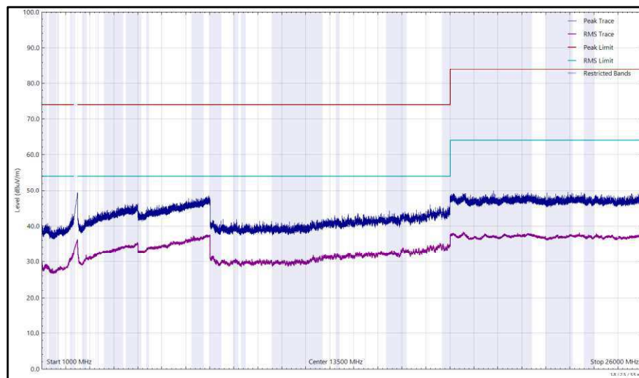
Figure 126 - 2437 MHz (CH6), HT20, CDD, Core 0 + Core 1, 1 GHz to 26 GHz, Horizontal
