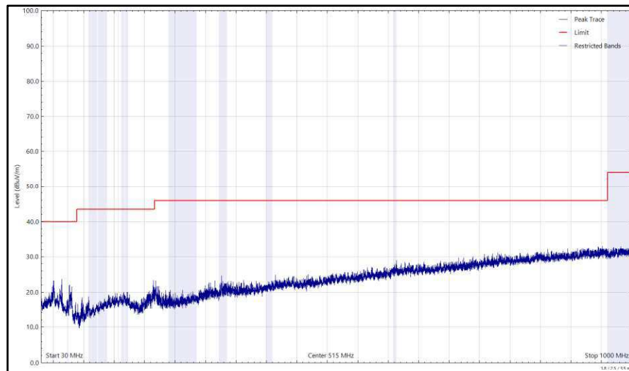
Figure 135 - 2437 MHz (CH6), HE20, RU26-0, CDD, Core 0 + Core 1, 30 MHz to 1 GHz, Vertical (Peak)
