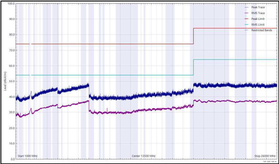
Figure 120 - 2437 MHz (CH6), 802.11g, Core 1, 1 GHz to 26 GHz, Vertical
