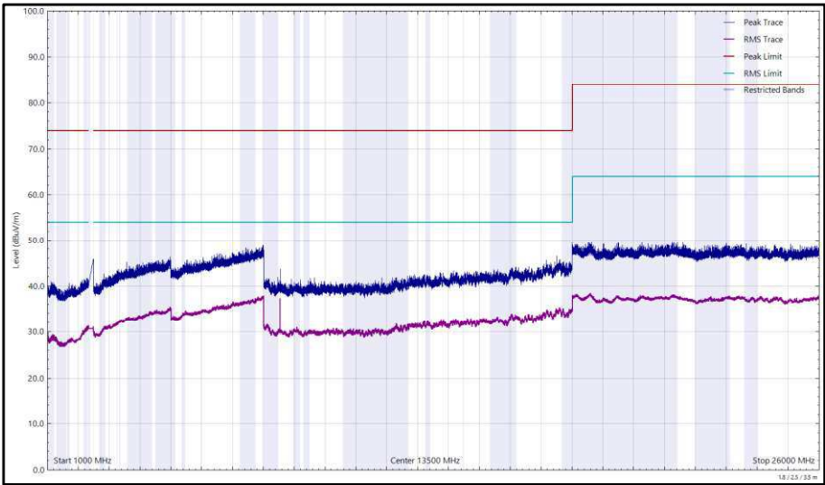
Figure 94 - 2437 MHz (CH6), 802.11b, Core 0, 1 GHz to 26 GHz, Horizontal
