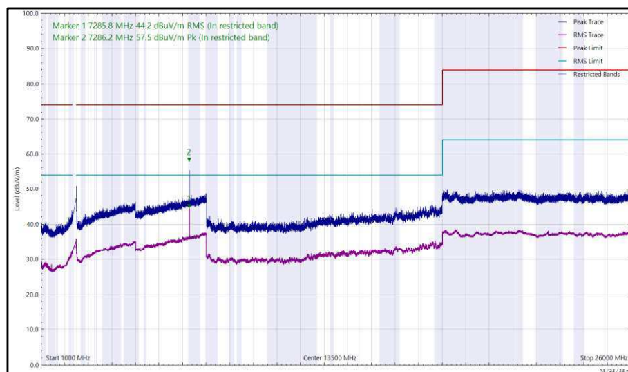
Figure 134 - 2437 MHz (CH6), HE20, RU26-0, CDD, Core 0 + Core 1, 1 GHz to 26 GHz, Horizontal
