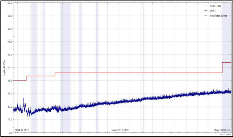
Figure 119 - 2437 MHz (CH6), 802.11g, Core 1, 30 MHz to 1 GHz, Vertical (Peak)
