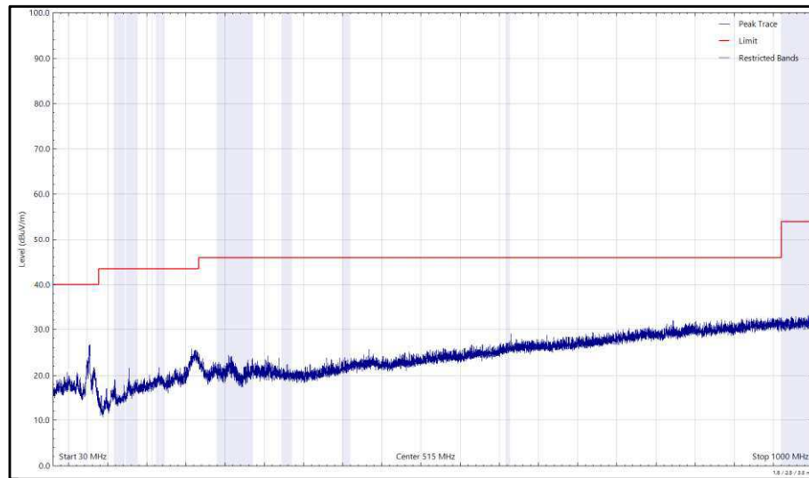
Figure 117 - 2437 MHz (CH6), 802.11g, Core 1, 30 MHz to 1 GHz, Horizontal (Peak)
