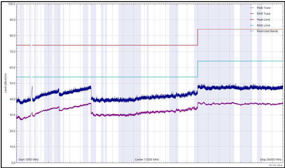
Figure 102 - 2437 MHz (CH6), 802.11b, Core 1, 1 GHz to 26 GHz, Horizontal
