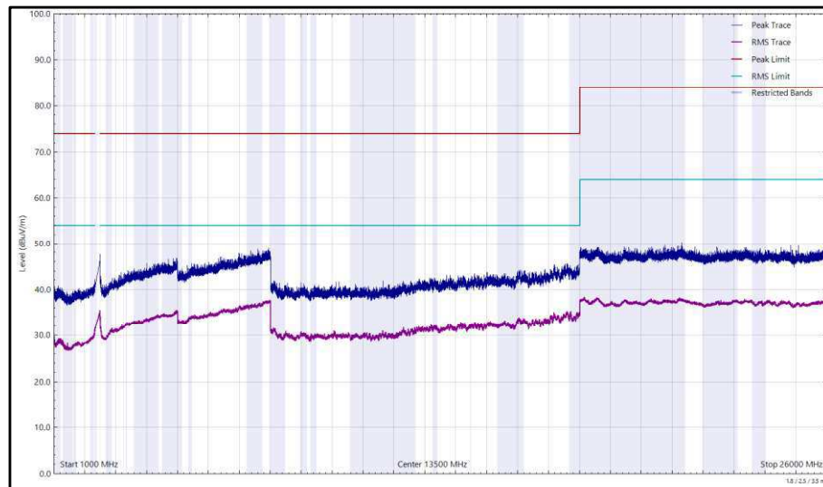
Figure 118 - 2437 MHz (CH6), 802.11g, Core 1, 1 GHz to 26 GHz, Horizontal
