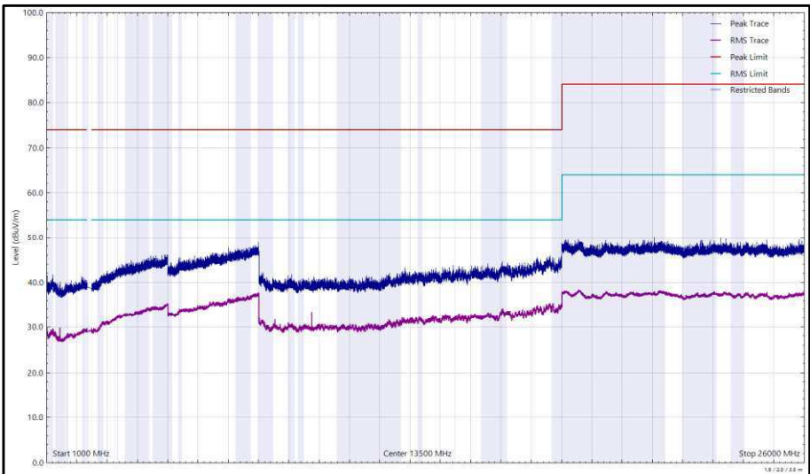
Figure 96 - 2437 MHz (CH6), 802.11b, Core 0, 1 GHz to 26 GHz, Vertical
