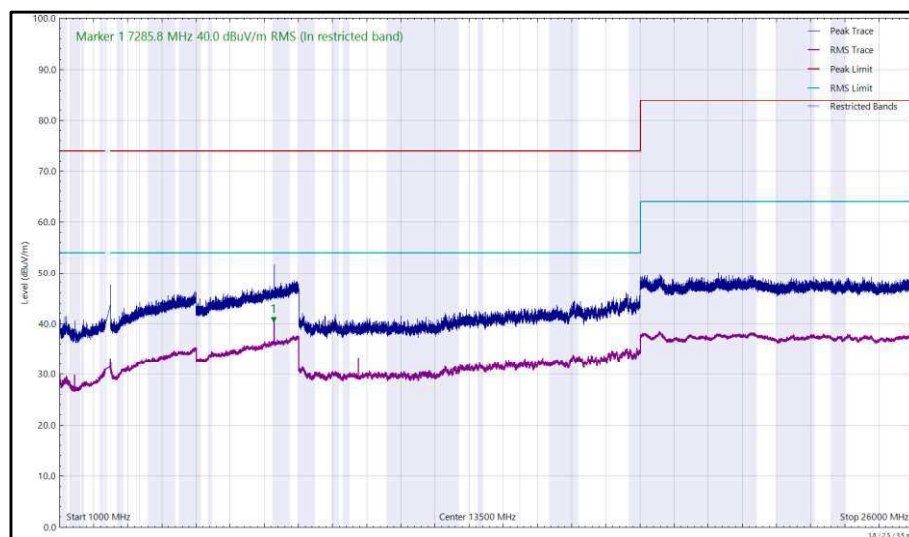
Figure 136 - 2437 MHz (CH6), HE20, RU26-0, CDD, Core 0 + Core 1, 1 GHz to 26 GHz, Vertical
