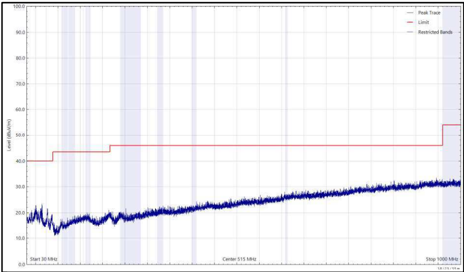
Figure 103 - 2437 MHz (CH6), 802.11b, Core 1, 30 MHz to 1 GHz, Vertical (Peak)
