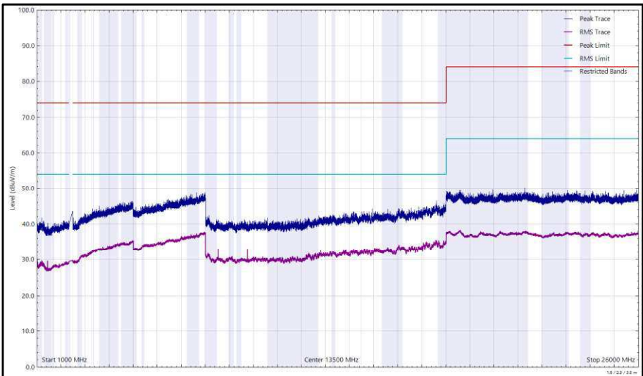
Figure 104 - 2437 MHz (CH6), 802.11b, Core 1, 1 GHz to 26 GHz, Vertical
