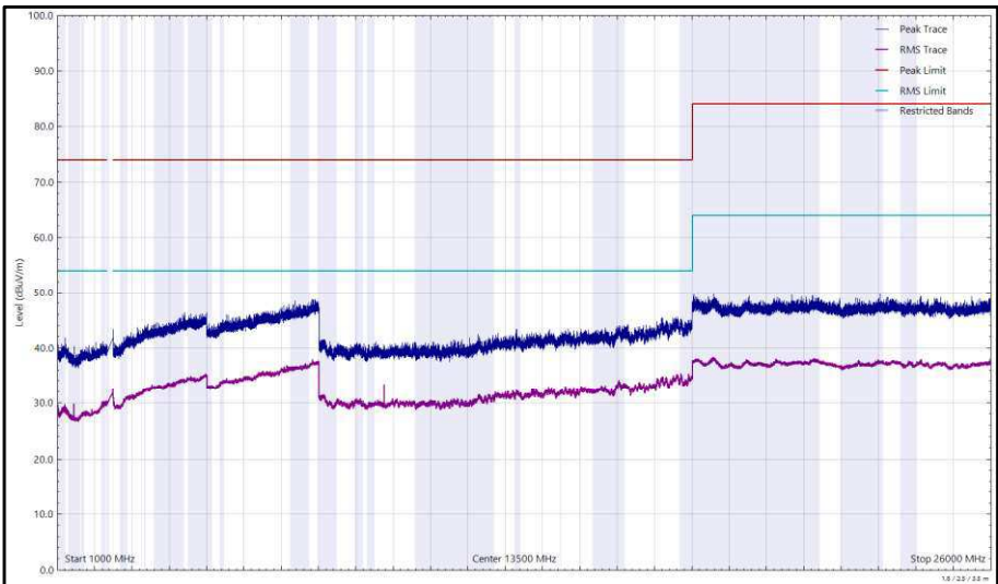
Figure 112 - 2437 MHz (CH6), 802.11g, Core 0, 1 GHz to 26 GHz, Vertical
