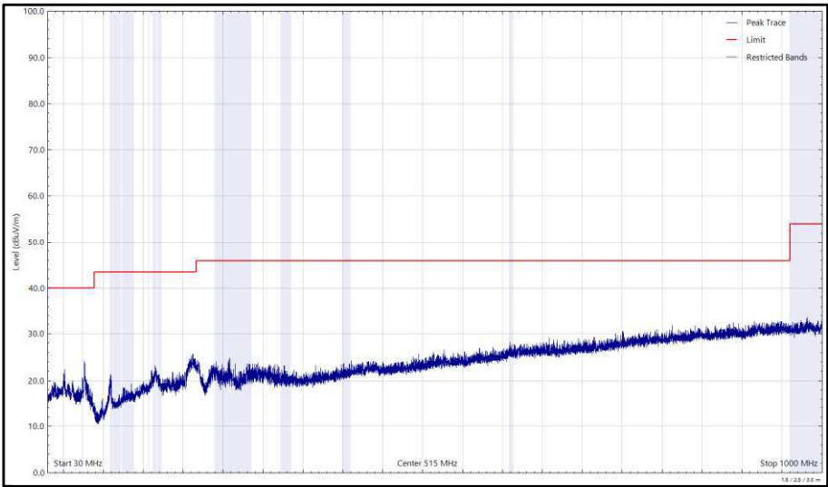
Figure 93 - 2437 MHz (CH6), 802.11b, Core 0, 30 MHz to 1 GHz, Horizontal (Peak)
