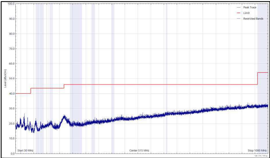
Figure 95 - 2437 MHz (CH6), 802.11b, Core 0, 30 MHz to 1 GHz, Vertical (Peak)
