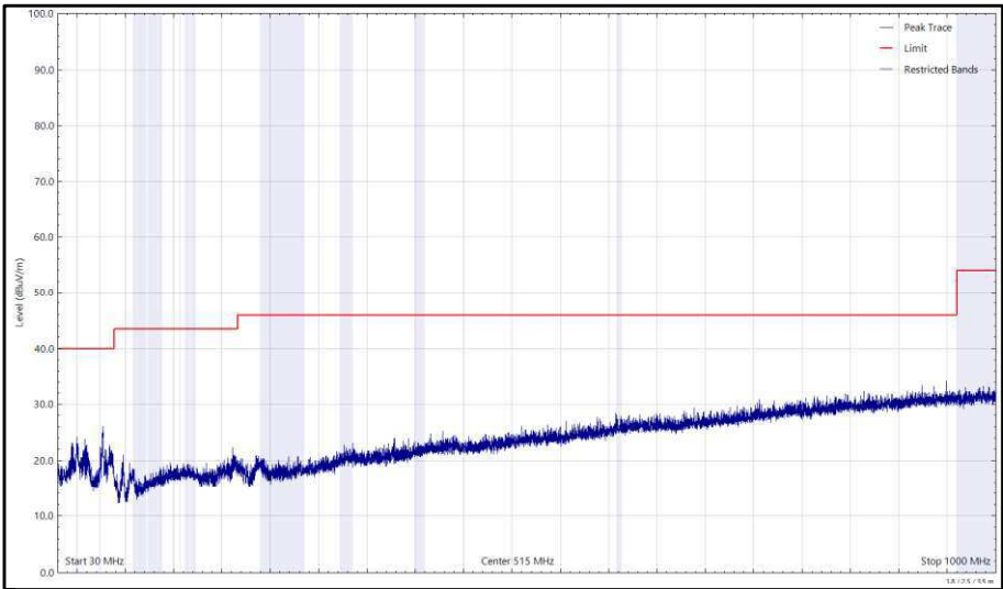
Figure 111 - 2437 MHz (CH6), 802.11g, Core 0, 30 MHz to 1 GHz, Vertical (Peak)
