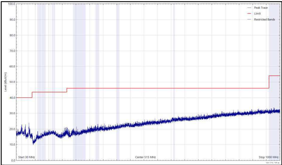
Figure 127 - 2437 MHz (CH6), HT20, CDD, Core 0 + Core 1, 30 MHz to 1 GHz, Vertical (Peak)
