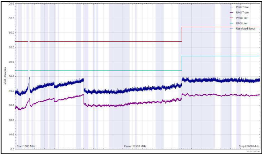
Figure 110 - 2437 MHz (CH6), 802.11g, Core 0, 1 GHz to 26 GHz, Horizontal
