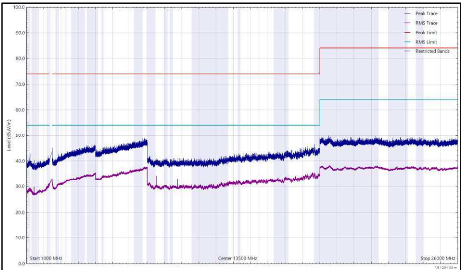
Figure 128 - 2437 MHz (CH6), HT20, CDD, Core 0 + Core 1, 1 GHz to 26 GHz, Vertical
