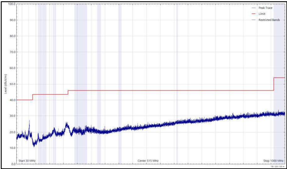
Figure 101 - 2437 MHz (CH6), 802.11b, Core 1, 30 MHz to 1 GHz, Horizontal (Peak)
