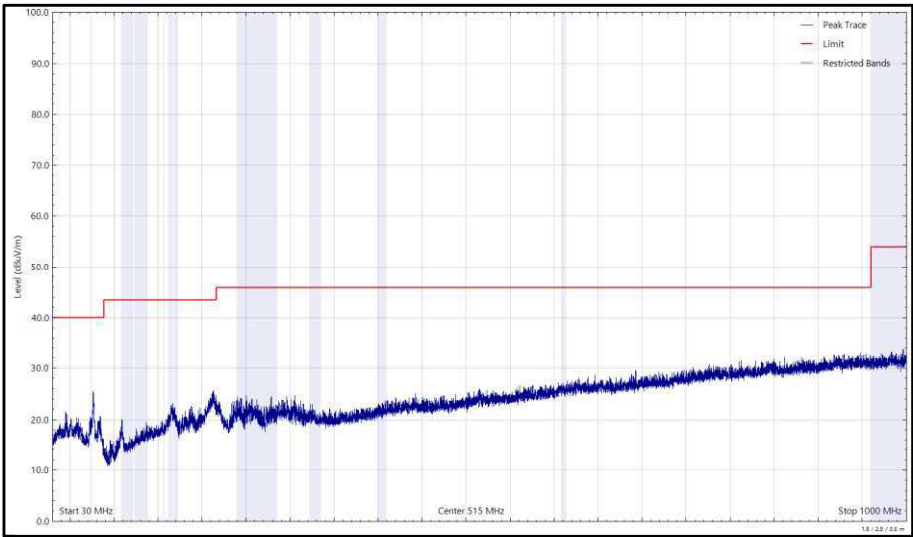
Figure 109 - 2437 MHz (CH6), 802.11g, Core 0, 30 MHz to 1 GHz, Horizontal (Peak)
