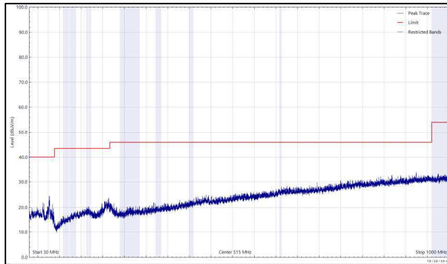
Figure 125 - 2437 MHz (CH6), HT20, CDD, Core 0 + Core 1, 30 MHz to 1 GHz, Horizontal (Peak)
