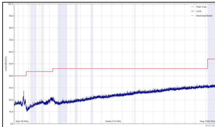
Figure 133 - 2437 MHz (CH6), HE20, RU26-0, CDD, Core 0 + Core 1, 30 MHz to 1 GHz, Horizontal (Peak)
