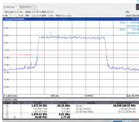
1-N25-15-20-M-9-CP-256QAM-Outer_Full-106@0-Ant1 1-18.949-20.080-≤20-PASS
