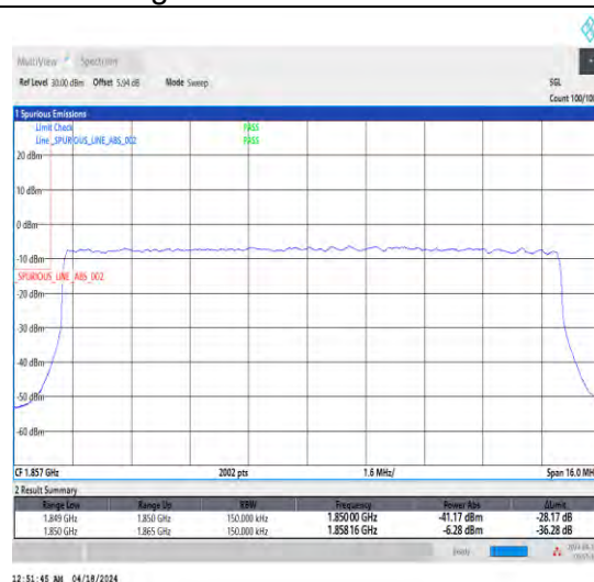
1-N25-15-15-L-3-DFT-PI2BPSK-Outer_Full-75@0-Ant1-1-seegraph-PASS-see graph
