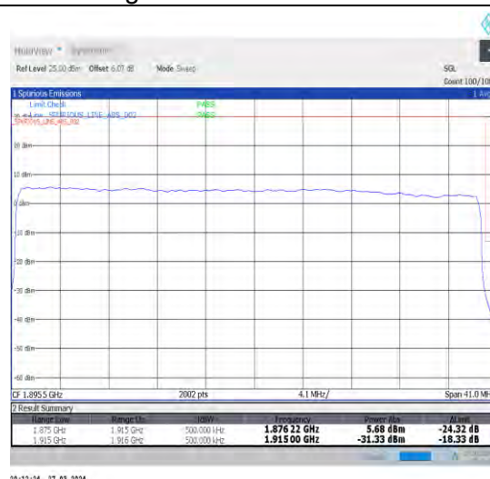
1-N25-15-40-H-3-DFT-PI2BPSK-Outer_Full-216@0-Ant1-1-seegraph-PASS-see graph
