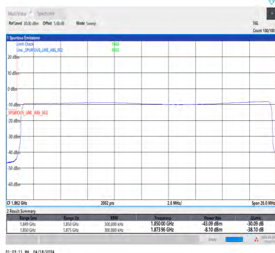
1-N25-15-25-L-6-CP-QPSK-Outer_Full-133@0-Ant1-1-seegraph-PASS-see graph
