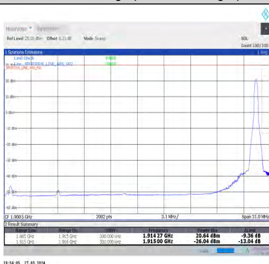
1-N25-15-30-H-5-CP-QPSK-Edge_1RB_Right-1@159-Ant1-1-seegraph-PASS-see graph
