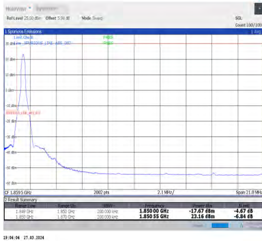
1-N25-15-20-L-1-DFT-PI2BPSK-Edge_1RB_Left-1@0-Ant1-1-seegraph-PASS-see graph
