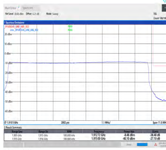
1-N25-15-10-H-6-CP-QPSK-Outer_Full-52@0-Ant1-1-seegraph-PASS-see graph
