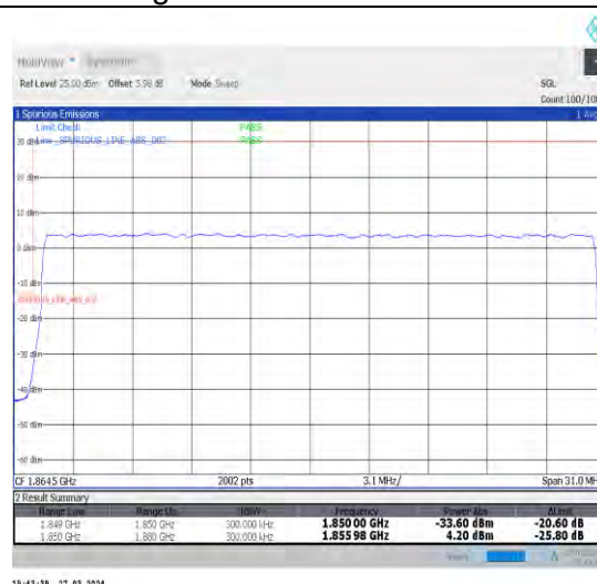
1-N25-15-30-L-3-DFT-PI2BPSK-Outer_Full-160@0-Ant1-1-seegraph-PASS-see graph
