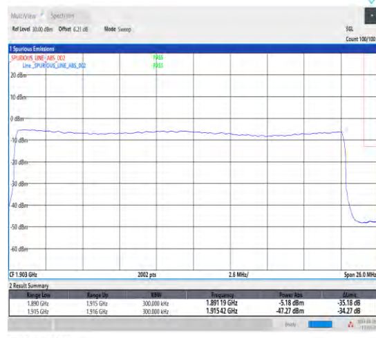
1-N25-15-25-H-3-DFT-PI2BPSK-Outer_Full-128@0-Ant1-1-seegraph-PASS-see graph
