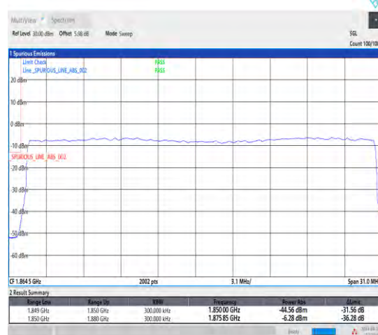
1-N25-15-30-L-3-DFT-PI2BPSK-Outer_Full-160@0-Ant1-1-seegraph-PASS-see graph
