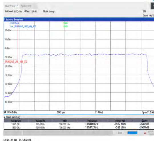
1-N25-15-10-L-3-DFT-PI2BPSK-Outer_Full-50@0- Ant1-1-seegraph-PASS-see graph
