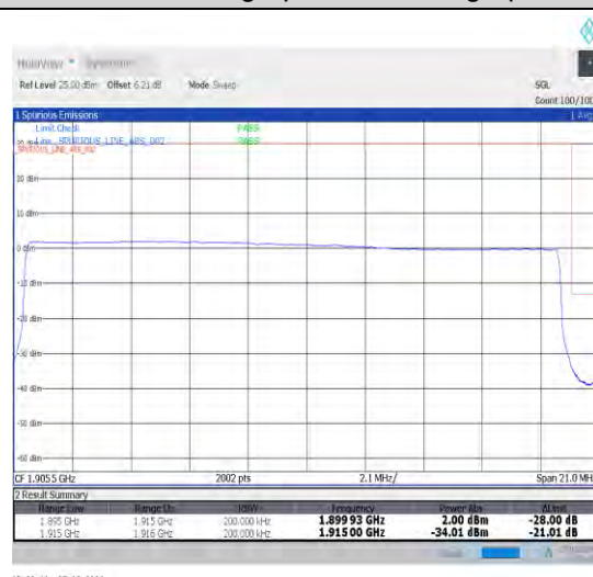
1-N25-15-20-H-6-CP-QPSK-Outer_Full-106@0-Ant1-1-seegraph-PASS-see graph
