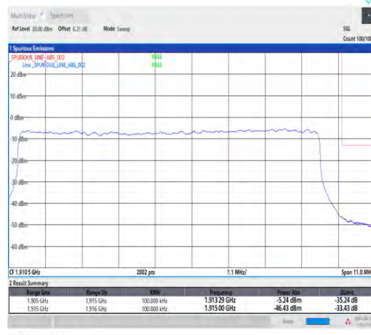
1-N25-15-10-H-3-DFT-PI2BPSK-Outer_Full-50@0-Ant1-1-seegraph-PASS-see graph
