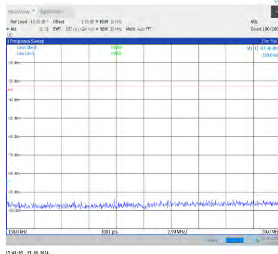
1-N25-15-40-L-1-DFT-PI2BPSK-Inner_1RB_Left-1@ 1-0.15-30-Ant1-0.15--87.46--33-PASS
