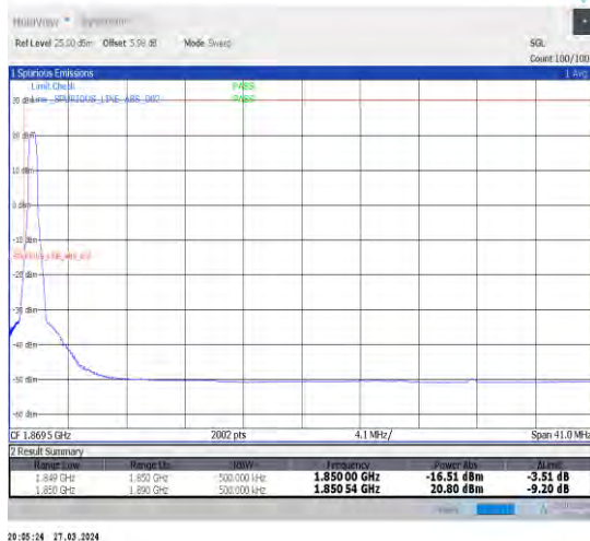
1-N25-15-40-L-4-CP-QPSK-Edge_1RB_Left-1@0-Ant1-1-seegraph-PASS-see graph
