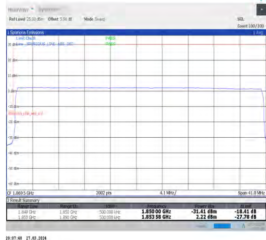
1-N25-15-40-L-6-CP-QPSK-Outer_Full-216@0-Ant1-1-seegraph-PASS-see graph
