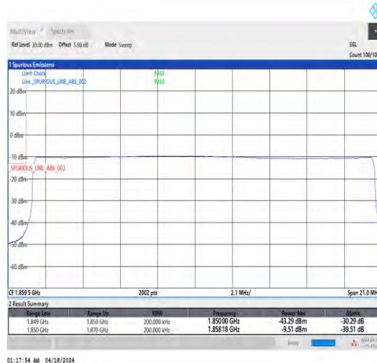
1-N25-15-20-L-6-CP-QPSK-Outer_Full-106@0-Ant1-1-seegraph-PASS-see graph
