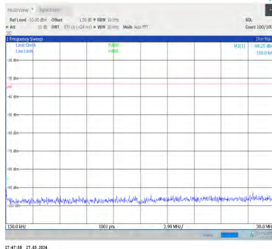
1-N25-15-40-H-1-DFT-PI2BPSK-Inner_1RB_Left-1@ 1-0.15-30-Ant1-0.15--88.25--33-PASS
