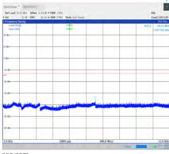
1-N25-15-40-M-1-DFT-PI2BPSK-Inner_1RB_Left-1 @1-3000-12000-Ant1-7997.70--36.59--13-PASS
