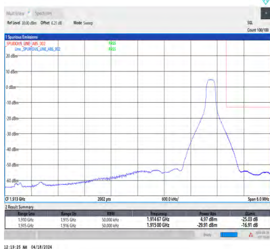
1-N25-15-5-H-5-CP-QPSK-Edge_1RB_Right-1@24-Ant1-1-seegraph-PASS-see graph
