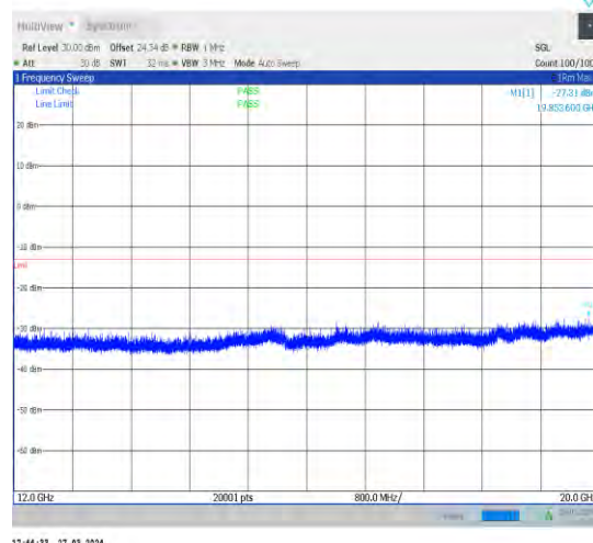
1-N25-15-40-L-1-DFT-PI2BPSK-Inner_1RB_Left-1@ 1-12000-20000-Ant1-19853.60--27.31--13-PASS
