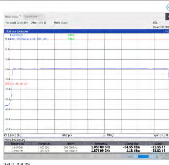
1-N25-15-30-L-6-CP-QPSK-Outer_Full-160@0-Ant1-1-seegraph-PASS-see graph
