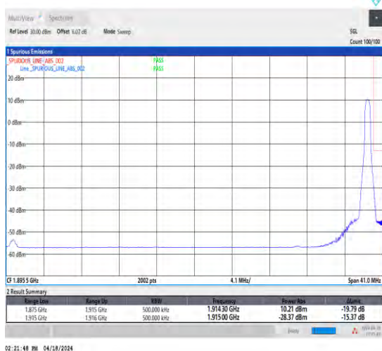
1-N25-15-40-H-5-CP-QPSK-Edge_1RB_Right-1@215-Ant1-1-seegraph-PASS-see graph
