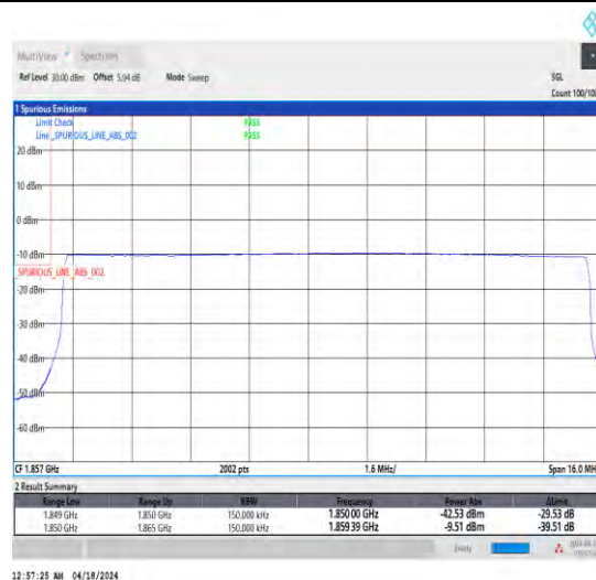
1-N25-15-15-L-6-CP-QPSK-Outer_Full-79@0-Ant1-1-seegraph-PASS-see graph
