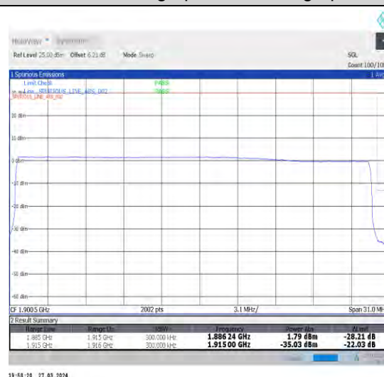
1-N25-15-30-H-6-CP-QPSK-Outer_Full-160@0-Ant1-1-seegraph-PASS-see graph
