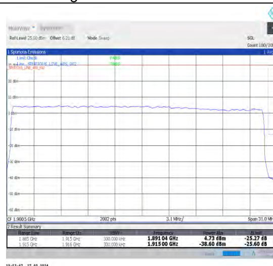
1-N25-15-30-H-3-DFT-PI2BPSK-Outer_Full-160@0-Ant1-1-seegraph-PASS-see graph
