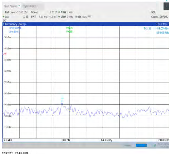
1-N25-15-40-H-1-DFT-PI2BPSK-Inner_1RB_Left-1 @1-0.009-0.15-Ant1-0.06--88.05--43-PASS
