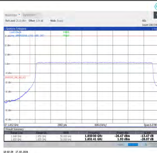
1-N25-15-5-L-6-CP-QPSK-Outer_Full-25@0-Ant1-1 1-seegraph-PASS-see graph
