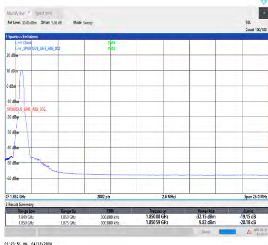
1-N25-15-25-L-4-CP-QPSK-Edge_1RB_Left-1@0-Ant1-1-seegraph-PASS-see graph
