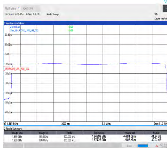
1-N25-15-30-L-6-CP-QPSK-Outer_Full-160@0-Ant1-1-seegraph-PASS-see graph
