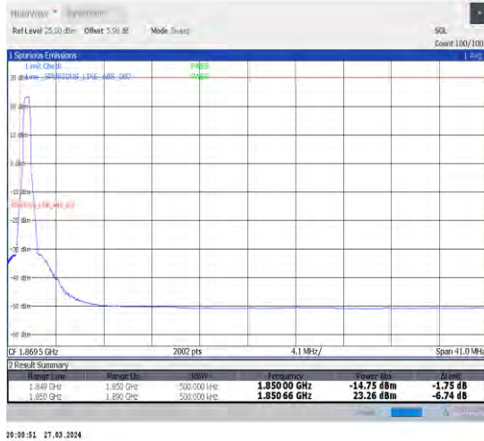
1-N25-15-40-L-1-DFT-PI2BPSK-Edge_1RB_Left-1@0-Ant1-1-seegraph-PASS-see graph
