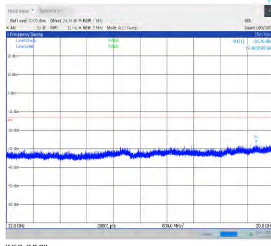
1-N25-15-40-M-1-DFT-PI2BPSK-Inner_1RB_Left-1@ 1-12000-20000-Ant1-19465.60--26.76--13-PASS
