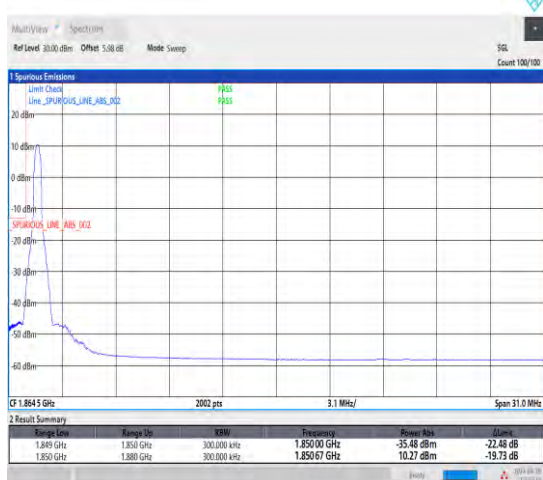
1-N25-15-30-L-1-DFT-PI2BPSK-Edge_1RB_Left-1@0-Ant1-1-seegraph-PASS-see graph
