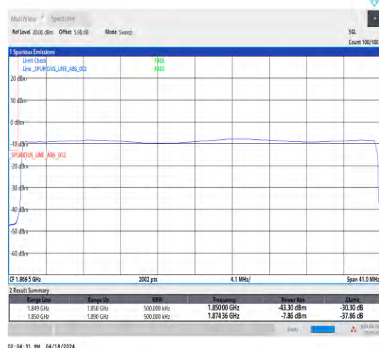
1-N25-15-40-L-6-CP-QPSK-Outer_Full-216@0-Ant1-1-seegraph-PASS-see graph
