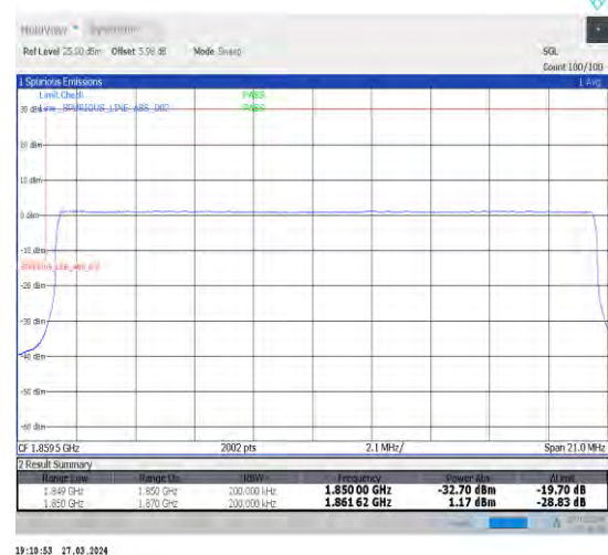
1-N25-15-20-L-6-CP-QPSK-Outer_Full-106@0-Ant1-1-seegraph-PASS-see graph
