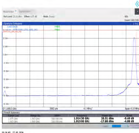
1-N25-15-40-H-5-CP-QPSK-Edge_1RB_Right-1@215-Ant1-1-seegraph-PASS-see graph
