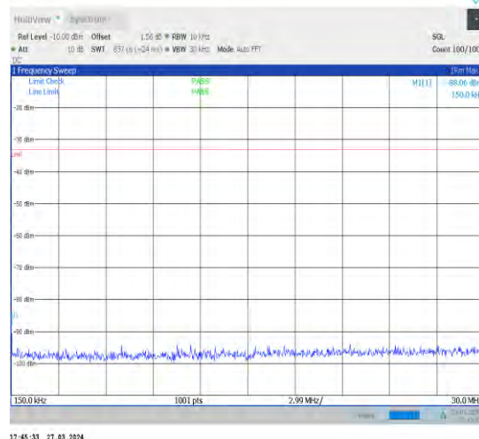
1-N25-15-40-M-1-DFT-PI2BPSK-Inner_1RB_Left-1@ 1-0.15-30-Ant1-0.15--88.06--33-PASS
