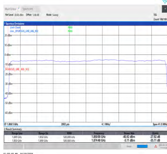
1-N25-15-40-L-3-DFT-PI2BPSK-Outer_Full-216@0-Ant1-1-seegraph-PASS-see graph
