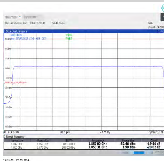
1-N25-15-25-L-6-CP-QPSK-Outer_Full-133@0-Ant1-1-seegraph-PASS-see graph
