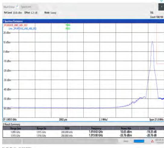
1-N25-15-20-H-2-DFT-PI2BPSK-Edge_1RB_Right-1@105-Ant1-1-seegraph-PASS-see graph
