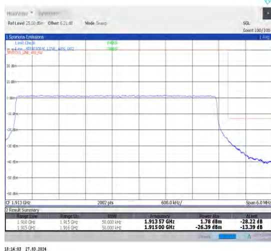
1-N25-15-5-H-6-CP-QPSK-Outer_Full-25@0-Ant1-1-seegraph-PASS-see graph
