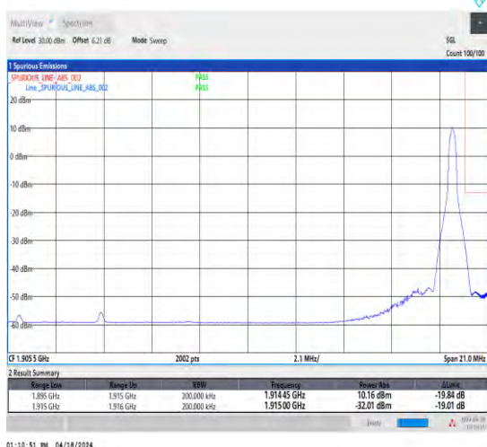
1-N25-15-20-H-5-CP-QPSK-Edge_1RB_Right-1@105-Ant1-1-seegraph-PASS-see graph
