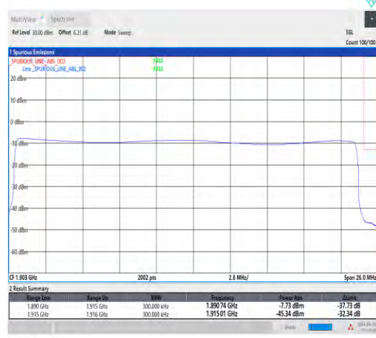
1-N25-15-25-H-6-CP-QPSK-Outer_Full-133@0-Ant1-1-seegraph-PASS-see graph
