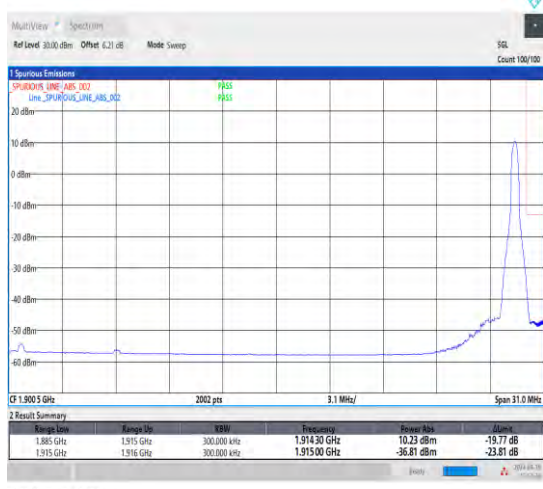
1-N25-15-30-H-5-CP-QPSK-Edge_1RB_Right-1@159-Ant1-1-seegraph-PASS-see graph
