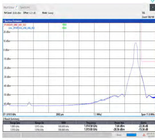
1-N25-15-10-H-5-CP-QPSK-Edge_1RB_Right-1@51-Ant1-1-seegraph-PASS-see graph
