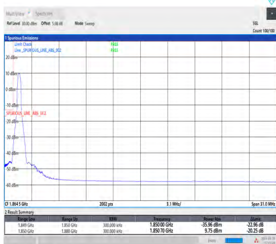
1-N25-15-30-L-4-CP-QPSK-Edge_1RB_Left-1@0-Ant1-1-seegraph-PASS-see graph
