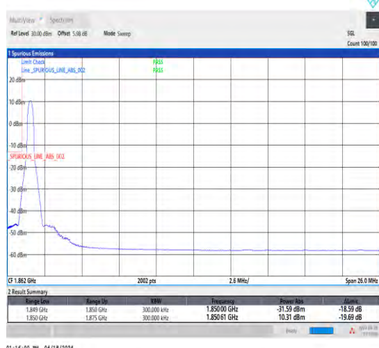
1-N25-15-25-L-1-DFT-PI2BPSK-Edge_1RB_Left-1@0-Ant1-1-seegraph-PASS-see graph
