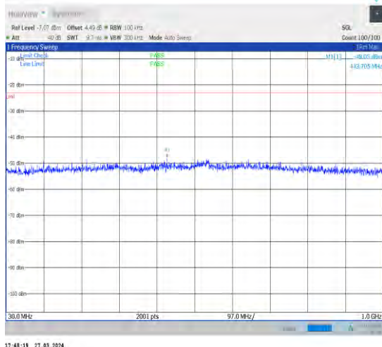
1-N25-15-40-H-1-DFT-PI2BPSK-Inner_1RB_Left-1 @1-30-1000-Ant1-443.71--48.05--23-PASS
