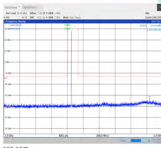
1-N25-15-40-L-1-DFT-PI2BPSK-Inner_1RB_Left-1@ 1-1000-3000-Ant1-2835.00--34.34--13-PASS
