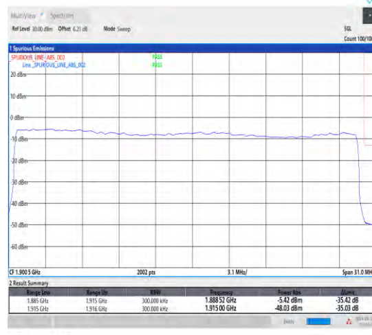
1-N25-15-30-H-3-DFT-PI2BPSK-Outer_Full-160@0-Ant1-1-seegraph-PASS-see graph
