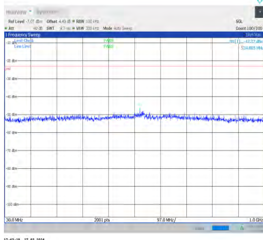
1-N25-15-40-L-1-DFT-PI2BPSK-Inner_1RB_Left-1 @1-30-1000-Ant1-534.89--47.32--23-PASS
