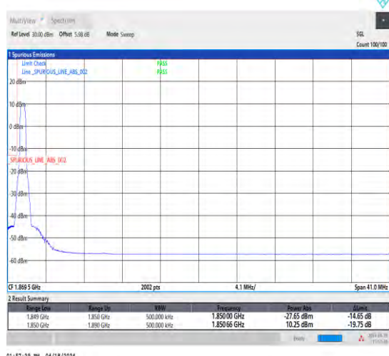
1-N25-15-40-L-1-DFT-PI2BPSK-Edge_1RB_Left-1@0-Ant1-1-seegraph-PASS-see graph
