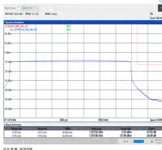
1-N25-15-5-H-6-CP-QPSK-Outer_Full-25@0-Ant1-1-seegraph-PASS-see graph
