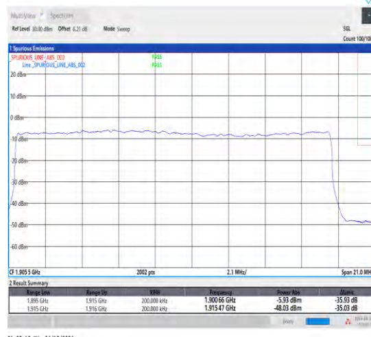
1-N25-15-20-H-3-DFT-PI2BPSK-Outer_Full-100@0-Ant1-1-seegraph-PASS-see graph
