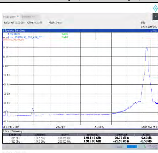
1-N25-15-20-H-5-CP-QPSK-Edge_1RB_Right-1@105-Ant1-1-seegraph-PASS-see graph
