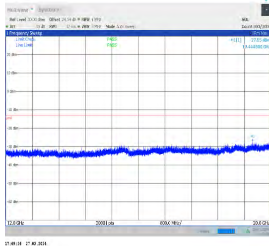
1-N25-15-40-H-1-DFT-PI2BPSK-Inner_1RB_Left-1@ 1-12000-20000-Ant1-19444.80--27.55--13-PASS
