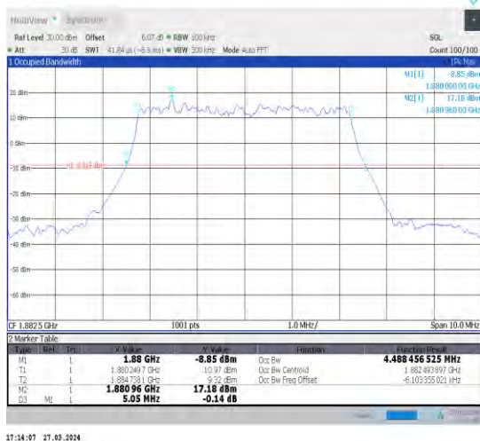
1-N25-15-5-M-1-DFT-QPSK-Outer_Full-25@0-Ant1- 4.488-5.050-≤5-PASS
