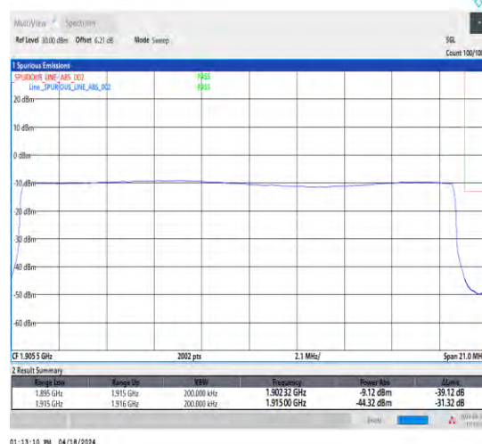
1-N25-15-20-H-6-CP-QPSK-Outer_Full-106@0-Ant1-1-seegraph-PASS-see graph
