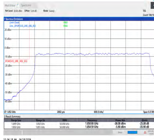
1-N25-15-5-L-3-DFT-PI2BPSK-Outer_Full-25@0- Ant1-1-seegraph-PASS-see graph
