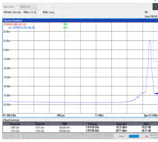
1-N25-15-30-H-2-DFT-PI2BPSK-Edge_1RB_Right-1@159-Ant1-1-seegraph-PASS-see graph
