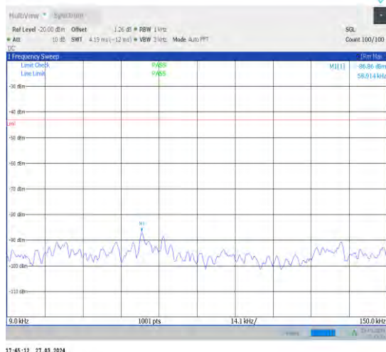
1-N25-15-40-M-1-DFT-PI2BPSK-Inner_1RB_Left-1 @ 1-0.009-0.15-Ant1-0.06--86.86--43-PASS
