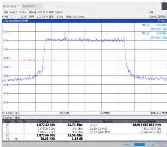
1-N25-15-20-M-6-CP-QPSK-Outer_Full-106@0-Ant1 -18.917-20.080-≤20-PASS
