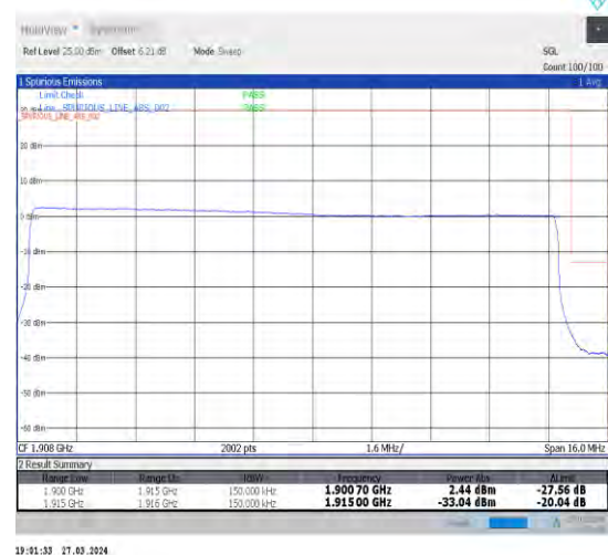
1-N25-15-15-H-6-CP-QPSK-Outer_Full-79@0-Ant1-1-seegraph-PASS-see graph
