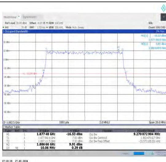
1-N25-15-10-M-8-CP-64QAM-Outer_Full-52@0-Ant1 -9.27-10.060-≤10-PASS
