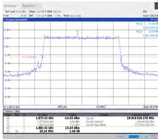
1-N25-15-20-M-7-CP-16QAM-Outer_Full-106@0-Ant1 1-18.916-20.160-≤20-PASS
