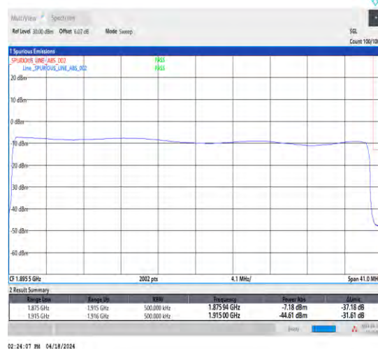
1-N25-15-40-H-6-CP-QPSK-Outer_Full-216@0-Ant1-1-seegraph-PASS-see graph
