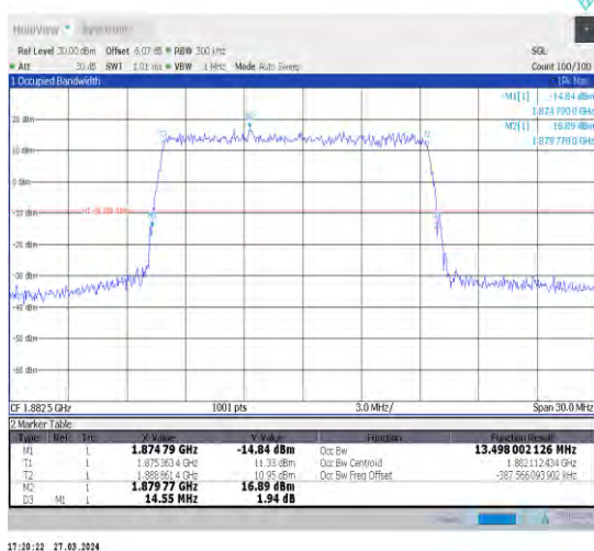
1-N25-15-15-M-1-DFT-QPSK-Outer_Full-75@0-Ant1 -13.498-14.550-≤15-PASS
