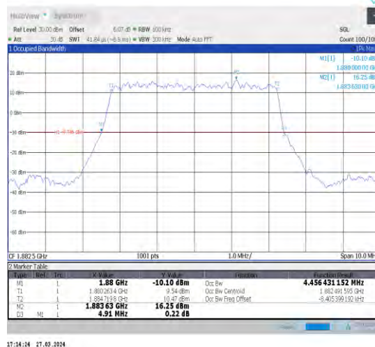
1-N25-15-5-M-2-DFT-PI2BPSK-Outer_Full-25@0-An t1-4.456-4.910-≤5-PASS
