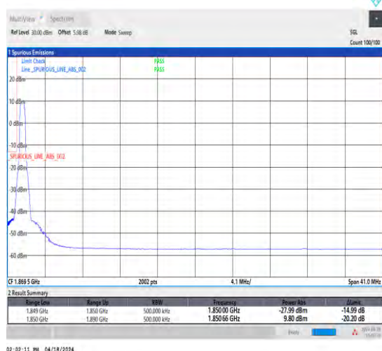
1-N25-15-40-L-4-CP-QPSK-Edge_1RB_Left-1@0-Ant1-1-seegraph-PASS-see graph
