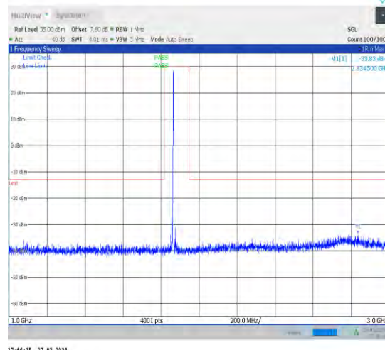
1-N25-15-40-M-1-DFT-PI2BPSK-Inner_1RB_Left-1@ 1-1000-3000-Ant1-2834.50--33.83--13-PASS
