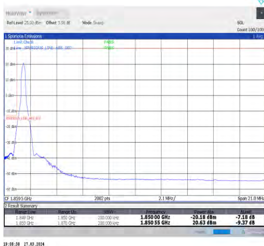
1-N25-15-20-L-4-CP-QPSK-Edge_1RB_Left-1@0-Ant1-1-seegraph-PASS-see graph
