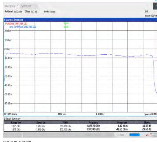
1-N25-15-40-H-3-DFT-PI2BPSK-Outer_Full-216@0-Ant1-1-seegraph-PASS-see graph
