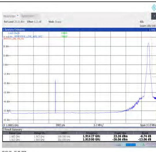
1-N25-15-30-H-2-DFT-PI2BPSK-Edge_1RB_Right-1@159-Ant1-1-seegraph-PASS-see graph
