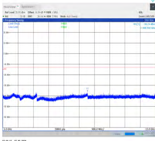
1-N25-15-40-L-1-DFT-PI2BPSK-Inner_1RB_Left-1 @ 1-3000-12000-Ant1-7988.70--36.24--13-PASS
