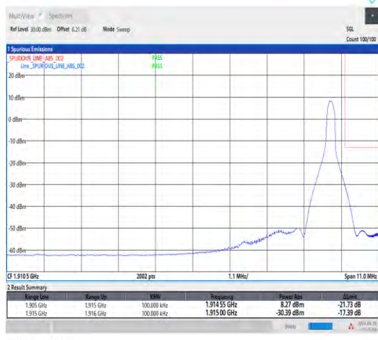
1-N25-15-10-H-2-DFT-PI2BPSK-Edge_1RB_Right-1@51-Ant1-1-seegraph-PASS-see graph
