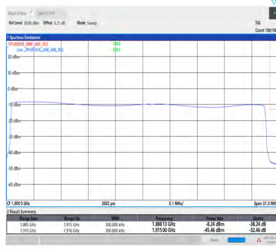
1-N25-15-30-H-6-CP-QPSK-Outer_Full-160@0-Ant1-1-seegraph-PASS-see graph
