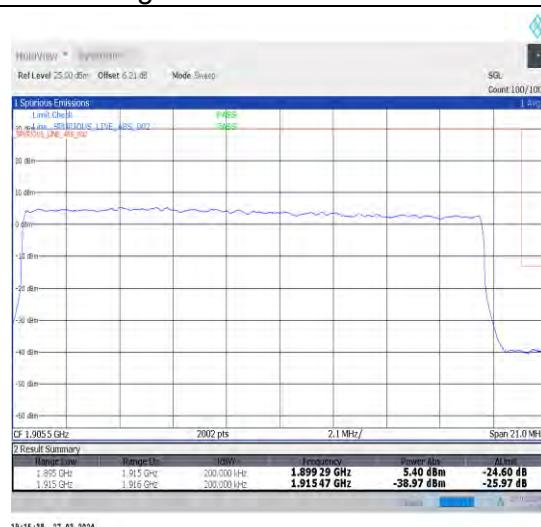
1-N25-15-20-H-3-DFT-PI2BPSK-Outer_Full-100@0-Ant1-1-seegraph-PASS-see graph
