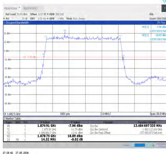
1-N25-15-15-M-2-DFT-PI2BPSK-Outer_Full-75@0-Ant1 -13.485-14.520-≤15-PASS
