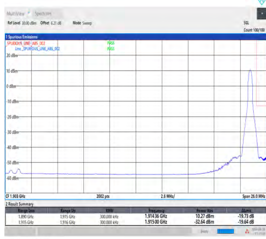
1-N25-15-25-H-5-CP-QPSK-Edge_1RB_Right-1@132-Ant1-1-seegraph-PASS-see graph
