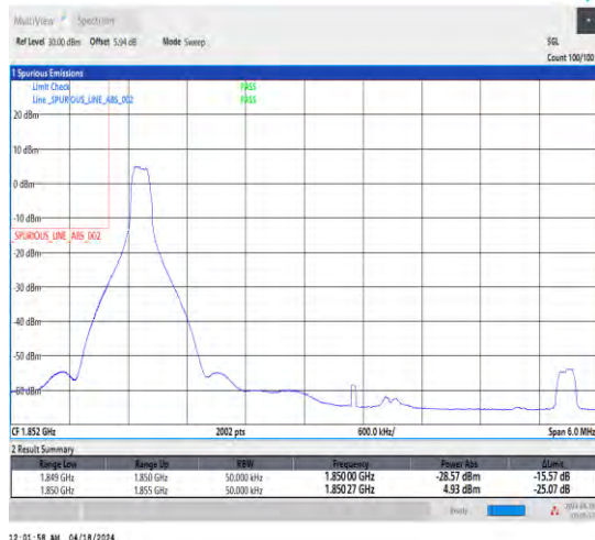
1-N25-15-5-L-1-DFT-PI2BPSK-Edge_1RB_Left-1@0-A nt1-1-seegraph-PASS-see graph
