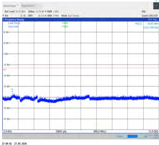
1-N25-15-40-H-1-DFT-PI2BPSK-Inner_1RB_Left-1 @1-3000-12000-Ant1-3551.70--35.85--13-PASS
