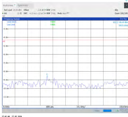
1-N25-15-40-L-1-DFT-PI2BPSK-Inner_1RB_Left-1 @1-0.009-0.15-Ant1-0.06--86.49--43-PASS
