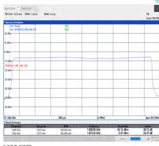
1-N25-15-25-L-3-DFT-PI2BPSK-Outer_Full-128@0-Ant1-1-seegraph-PASS-see graph
