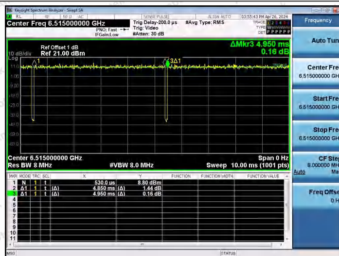
NTNV-11AX20SISO-Ant1-6515
