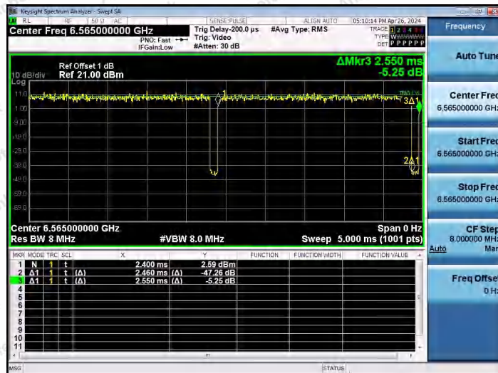
NTNV-11AX40SISO-Ant1-6565
