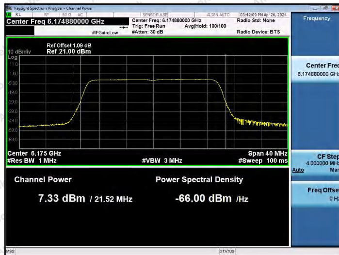
11AX20SISO-Ant1-6175-PASS
