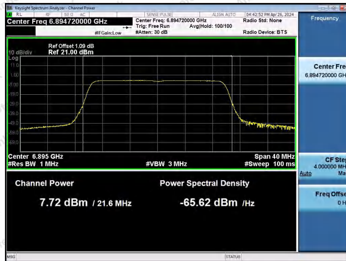
11AX20SISO-Ant1-6895-PASS
