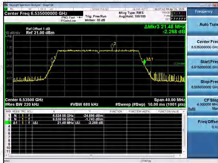
11AX20SISO-Ant1-6535
