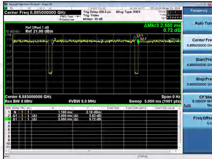
NTNV-11AX40SISO-Ant1-6885
