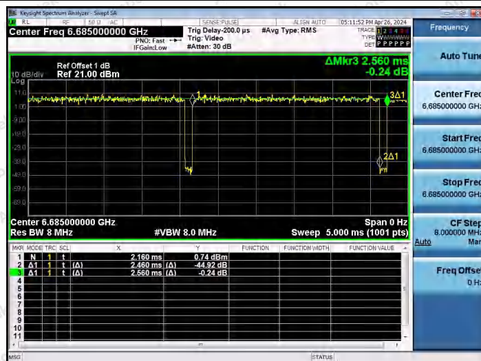
NTNV-11AX40SISO-Ant1-6685
