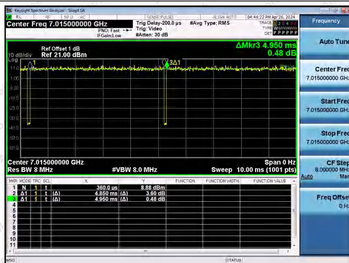
NTNV-11AX20SISO-Ant1-7015
