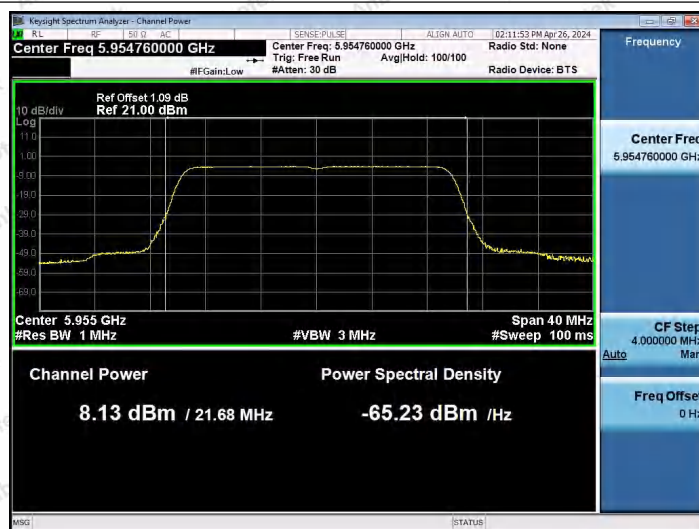
11AX20SISO-Ant1-5955-PASS
