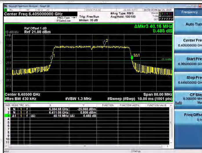
11AX40SISO-Ant1-6405
