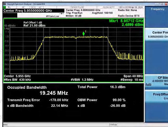
11AX20SISO-Ant1-5955-PASS
