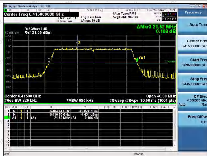
11AX20SISO-Ant1-6415
