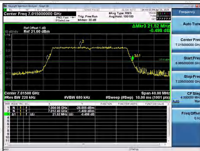
11AX20SISO-Ant1-7015
