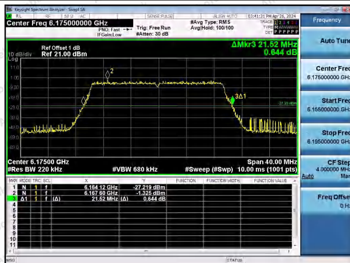
11AX20SISO-Ant1-6175
