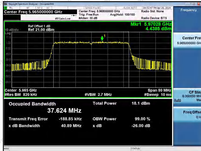
11AX40SISO-Ant1-5965-PASS
