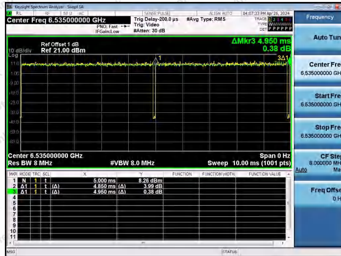
NTNV-11AX20SISO-Ant1-6535
