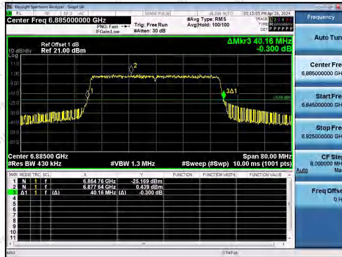
11AX40SISO-Ant1-6885
