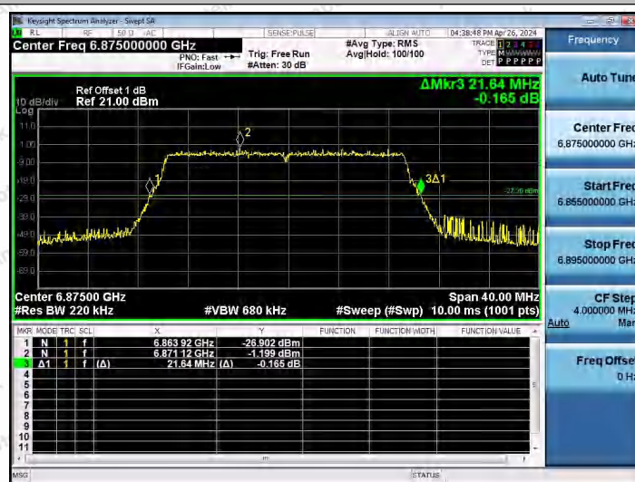
11AX20SISO-Ant1-6875
