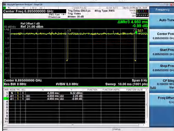
NTNV-11AX20SISO-Ant1-6895
