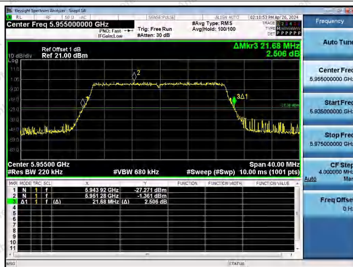
11AX20SISO-Ant1-5955
