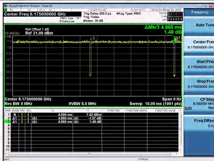
NTNV-11AX20SISO-Ant1-6175
