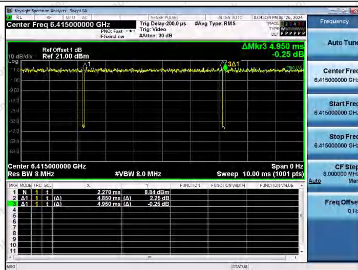
NTNV-11AX20SISO-Ant1-6415
