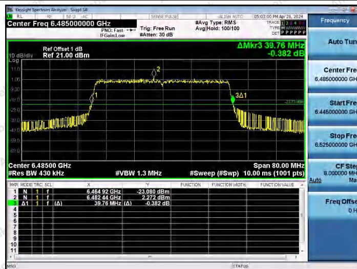
11AX40SISO-Ant1-6485
