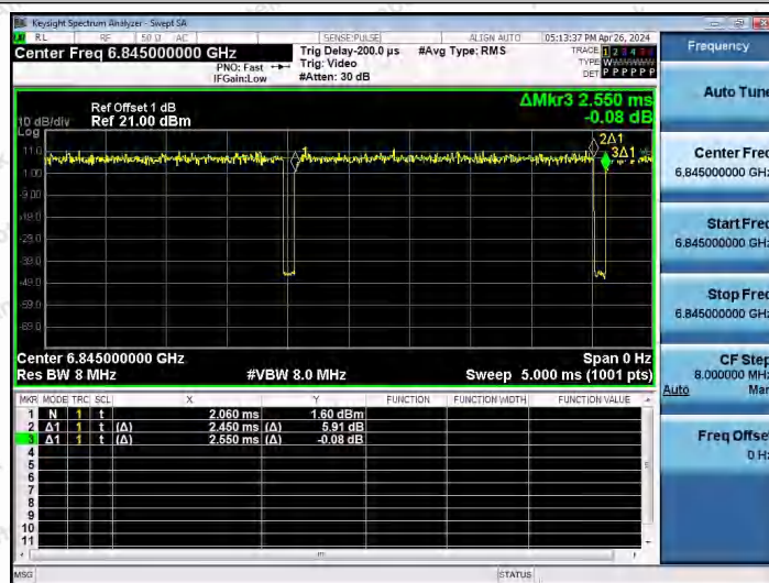
NTNV-11AX40SISO-Ant1-6845
