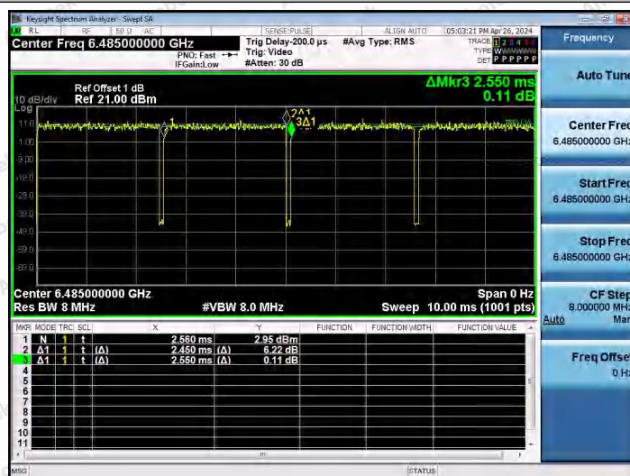
NTNV-11AX40SISO-Ant1-6485
