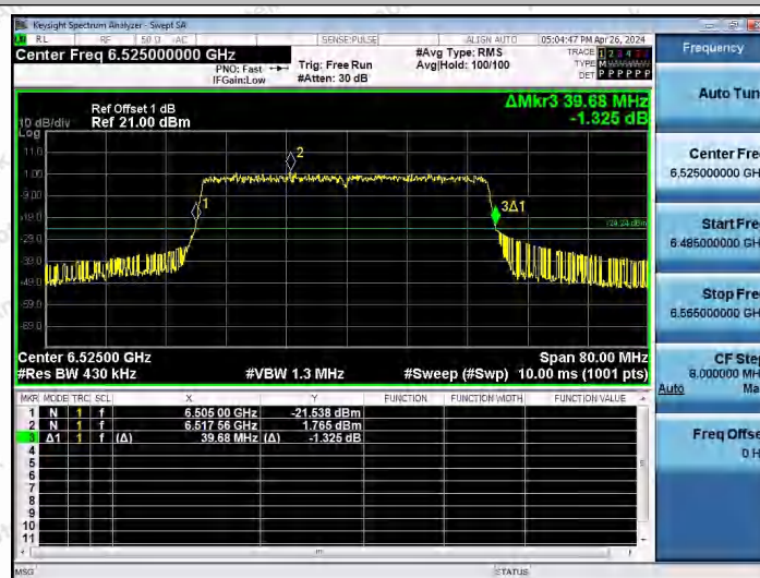
11AX40SISO-Ant1-6525
