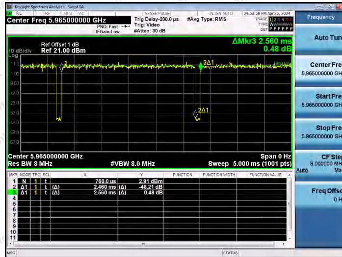
NTNV-11AX40SISO-Ant1-5965
