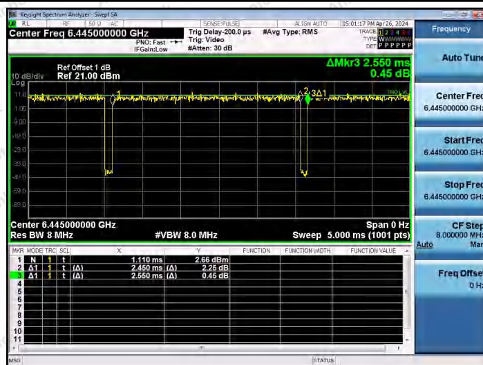
NTNV-11AX40SISO-Ant1-6445
