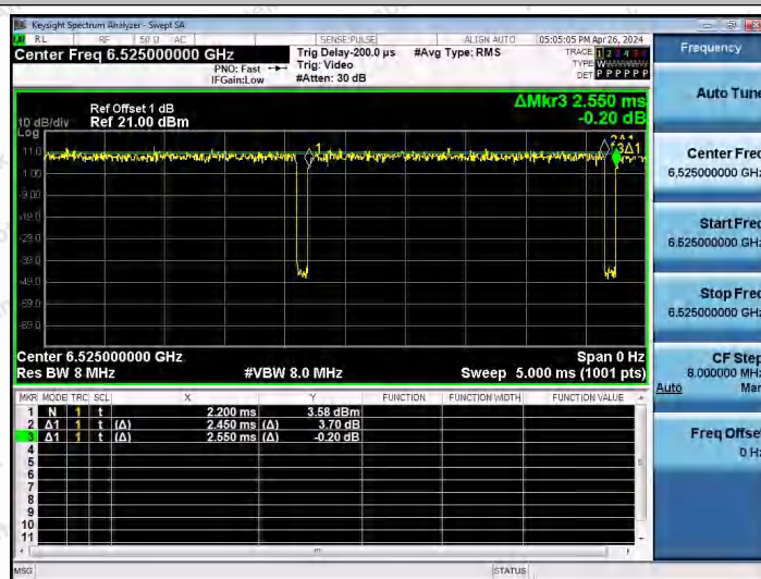
NTNV-11AX40SISO-Ant1-6525
