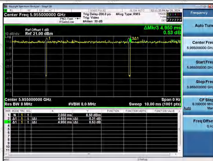
NTNV-11AX20SISO-Ant1-5955
