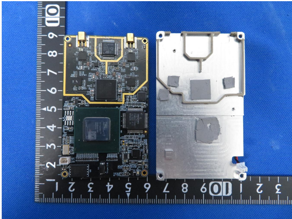
(1) EUT Photo (Model: WLN210-BM-a)
