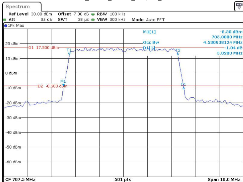
Band 12_5 MHz_Middle_16QAM_RB25#0
