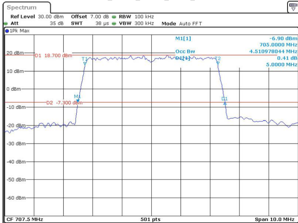
Band 12_5 MHz_Middle_QPSK_RB25#0
