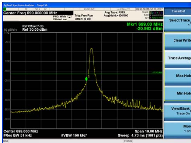
LTE Band 12 16QAM 5MHz CH-Low, 6RB
