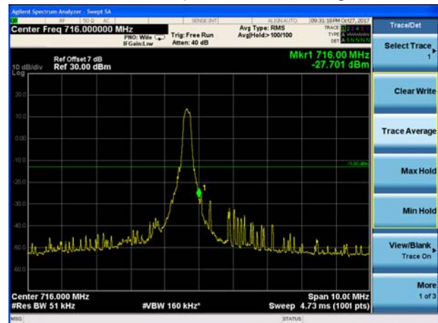
LTE Band 12 16QAM 5MHz CH-High, 6RB
