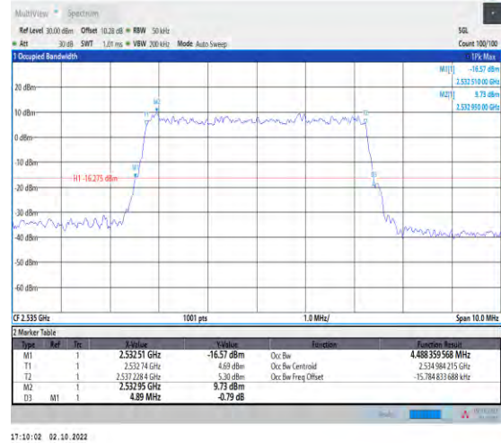
1-N7--15-5-M-5-DFT-256QAM-Outer_Full-25@0-Ant 1-4.488-4.890≤5-PASS
