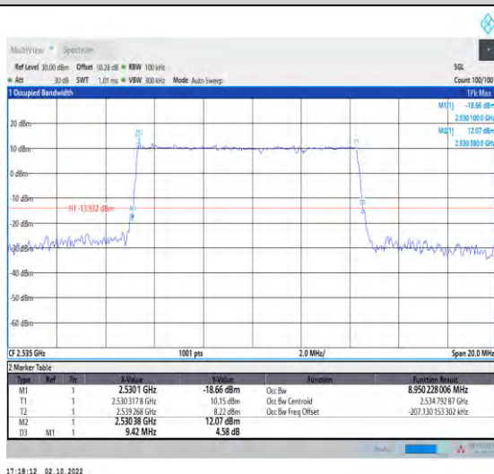
1-N7--15-10-M-3-DFT-16QAM-Outer_Full-50@0-Ant1-8.95-9.420-≤10-PASS
