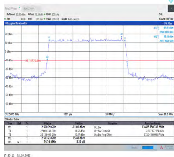
1-N7--15-15-L-2-DFT-PI2BPSK-Outer_Full-75@0-Ant1-13.426-14.160-≤15-PASS
