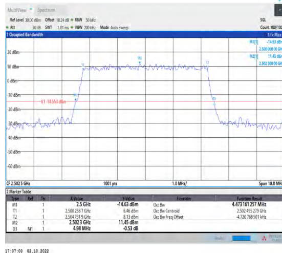
1-N7--15-5-L-4-DFT-64QAM-Outer_Full-25@0-Ant1- 4.473-4.980-≤5-PASS
