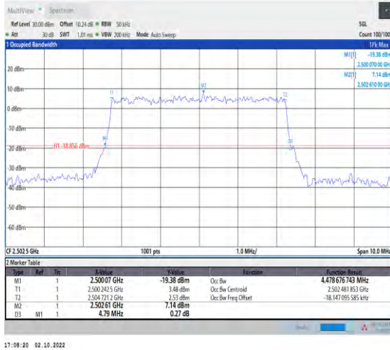
1-N7--15-5-L-9-CP-256QAM-Outer_Full-25@0-Ant1-4.479-4.790-≤5-PASS
