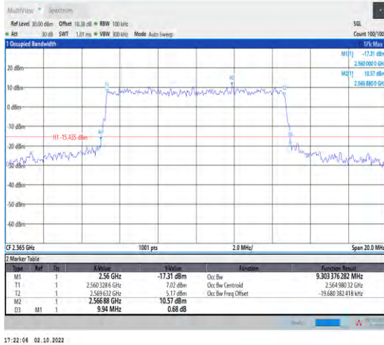
1-N7--15-10-H-8-CP-64QAM-Outer_Full-52@0-Ant1-9.303-9.940-≤10-PASS
