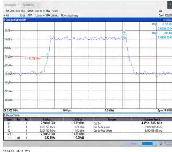
1-N7--15-5-L-2-DFT-PI2BPSK-Outer_Full-25@0-Ant 1-4.456-4.820-≤5-PASS
