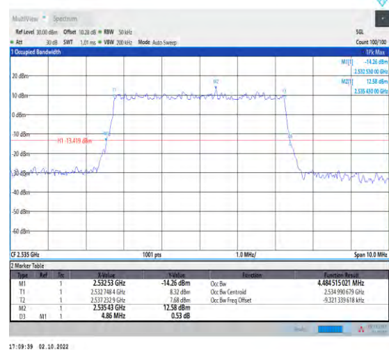
1-N7--15-5-M-3-DFT-16QAM-Outer_Full-25@0-Ant1-4.485-4.860-≤5-PASS
