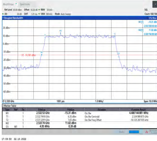
1-N7--15-5-M-4-DFT-64QAM-Outer_Full-25@0-Ant1 -4.48-4.950≤5-PASS
