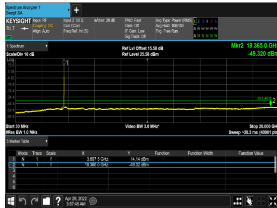
N48(10M)_DFT-s- OFDM_BPSK_Outer_Full_High_CH
