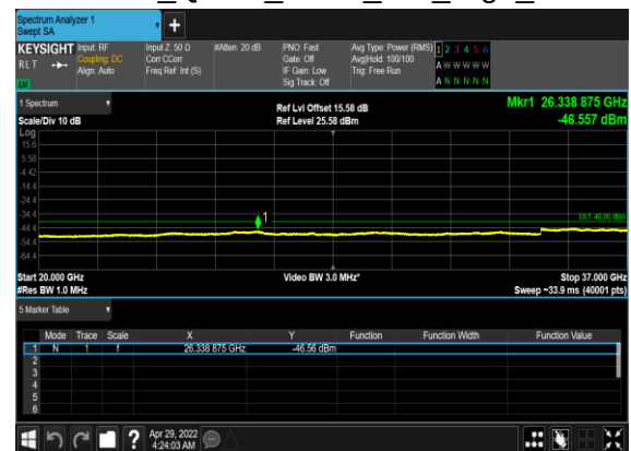
N48(20M)_DFT-s- OFDM_QPSK_Outer_Full_High_CH
