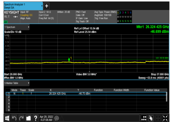
N48(40M)_DFT-s- OFDM_QPSK_Edge_1RB_Left_Low_CH
