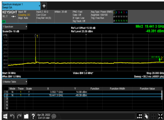
N48(10M)_DFT-s- OFDM_BPSK_Outer_Full_Low_CH
