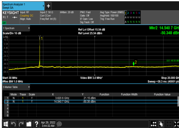
N48(10M)_DFT-s- OFDM_BPSK_Edge_1RB_Left_Mid_CH
