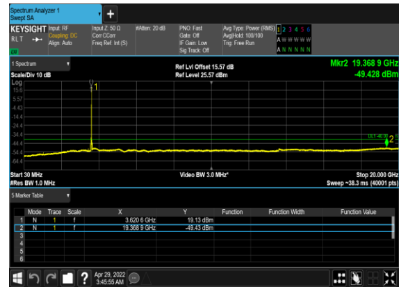
N48(10M)_DFT-s- OFDM_QPSK_Edge_1RB_Left_Mid_CH
