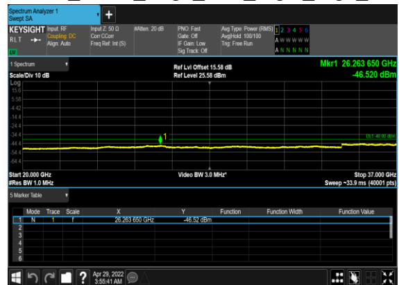
N48(10M)_DFT-s- OFDM_BPSK_Edge_1RB_Right_High_CH
