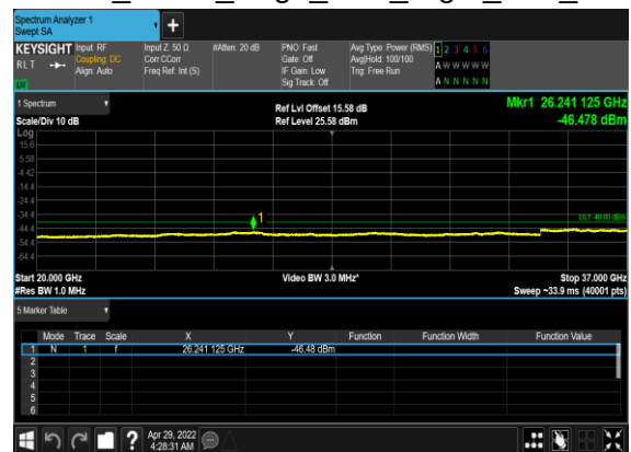
N48(40M)_DFT-s- OFDM_BPSK_Edge_1RB_Right_Low_CH
