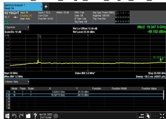
N48(10M)_DFT-s- OFDM_BPSK_Edge_1RB_Right_Mid_CH
