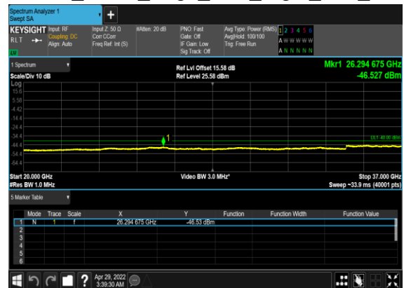
N48(10M)_DFT-s- OFDM_BPSK_Edge_1RB_Right_Low_CH
