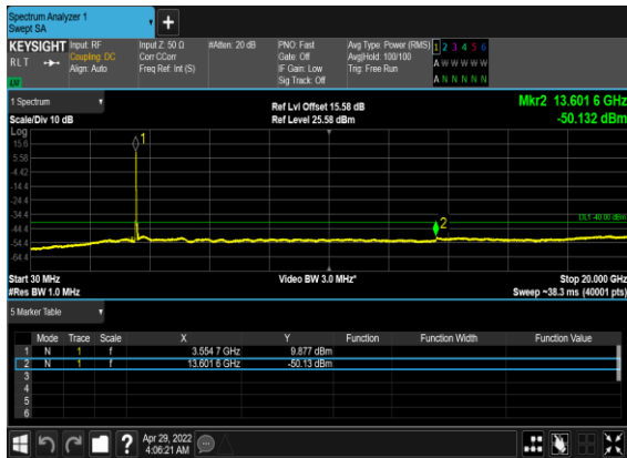
N48(20M)_DFT-s-OFDM_BPSK_Outer_Full_Low_CH
