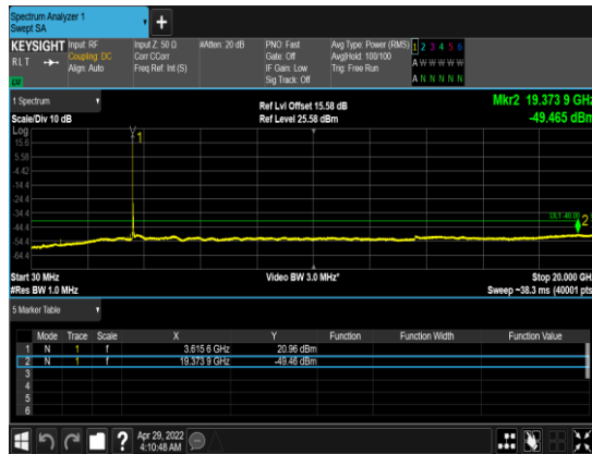
N48(20M)_DFT-s- OFDM_QPSK_Edge_1RB_Left_Mid_CH
