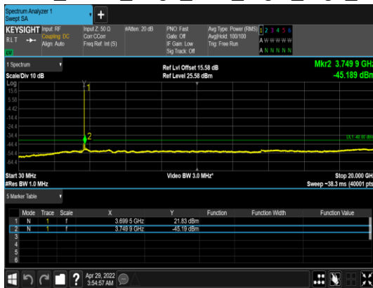
N48(10M)_DFT-s- OFDM_BPSK_Edge_1RB_Right_High_CH
