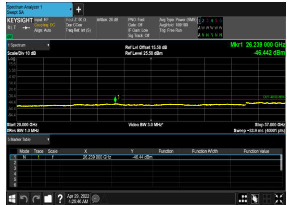
N48(40M)_DFT-s- OFDM_BPSK_Edge_1RB_Left_Low_CH
