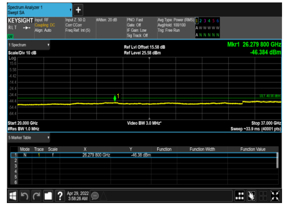
N48(10M)_DFT-s- OFDM_BPSK_Outer_Full_High_CH
