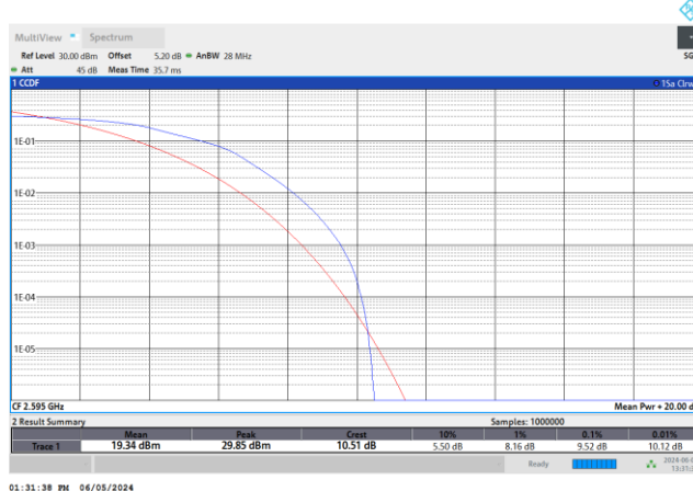
Band38-20MHz-QPSK-38000-100RB#0
