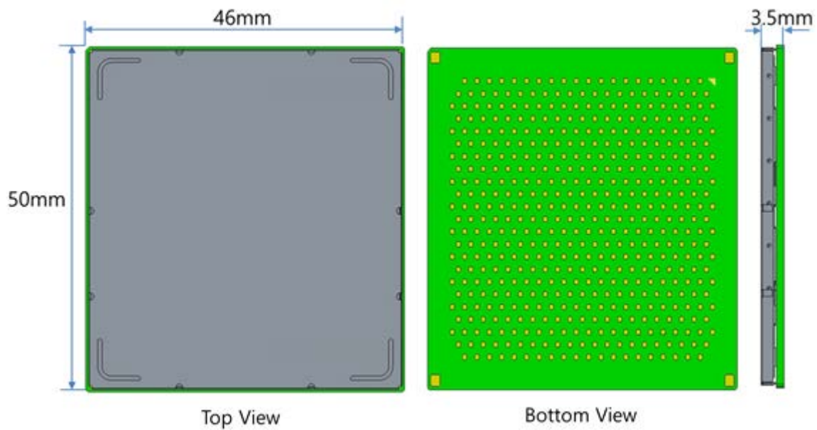
Mechanical Drawing
