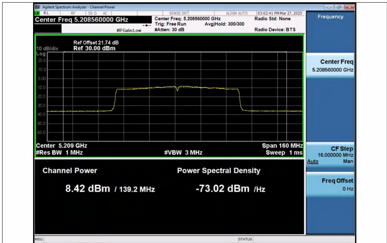
11AC80MIMO-Ant1-5210-PASS
