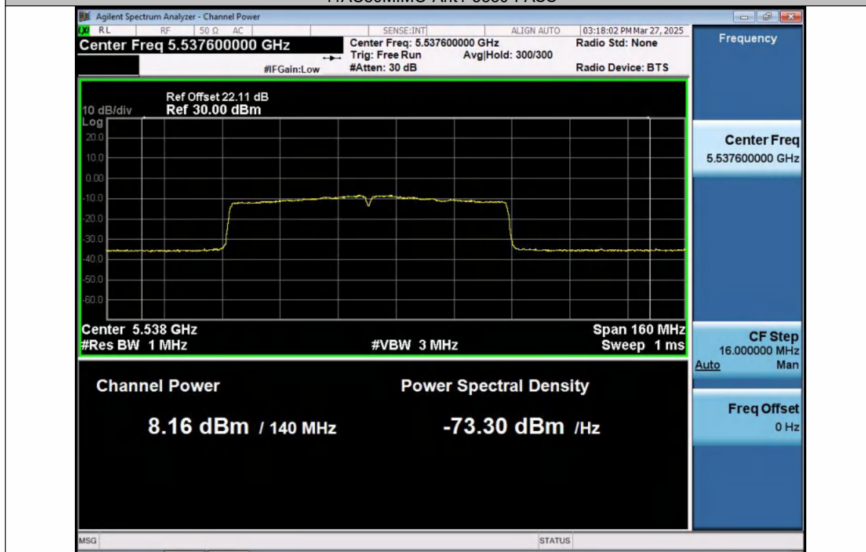
11AC80MIMO-Ant2-5530-PASS
