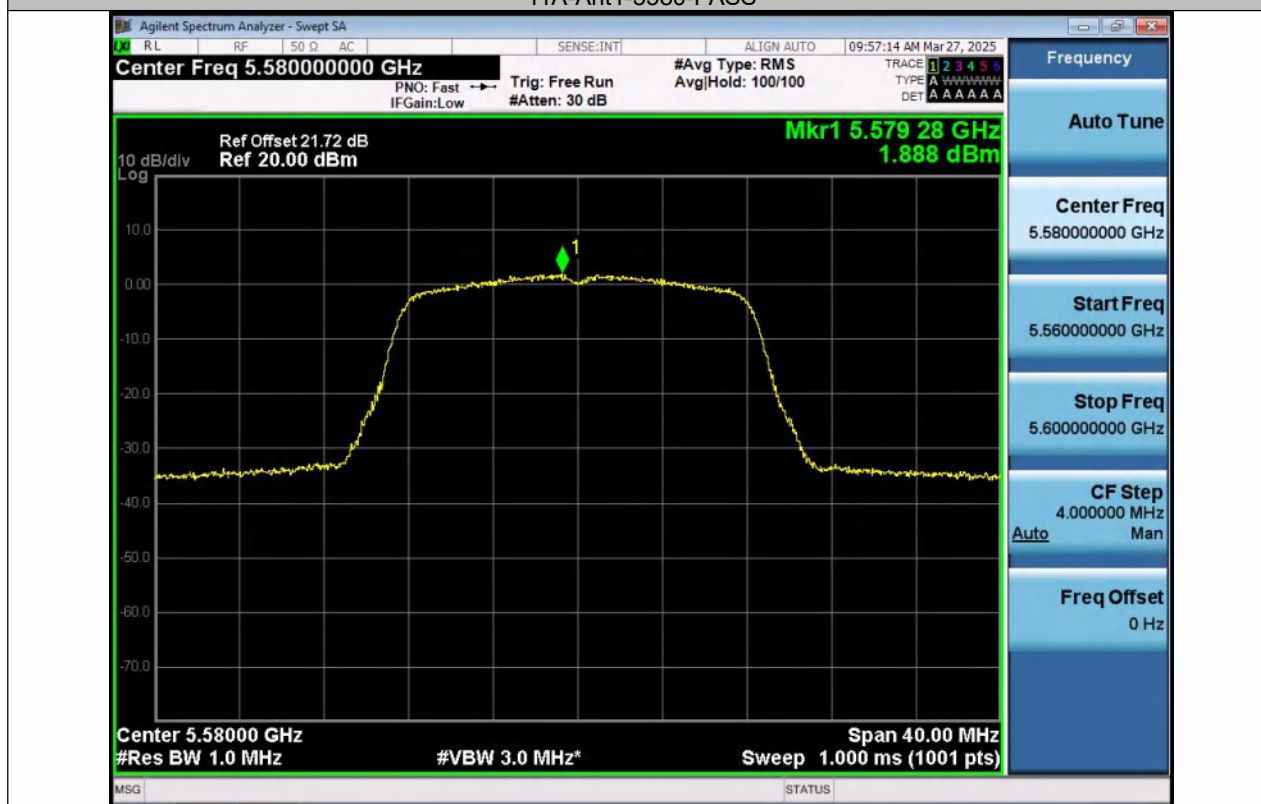
11A-Ant2-5580-PASS
