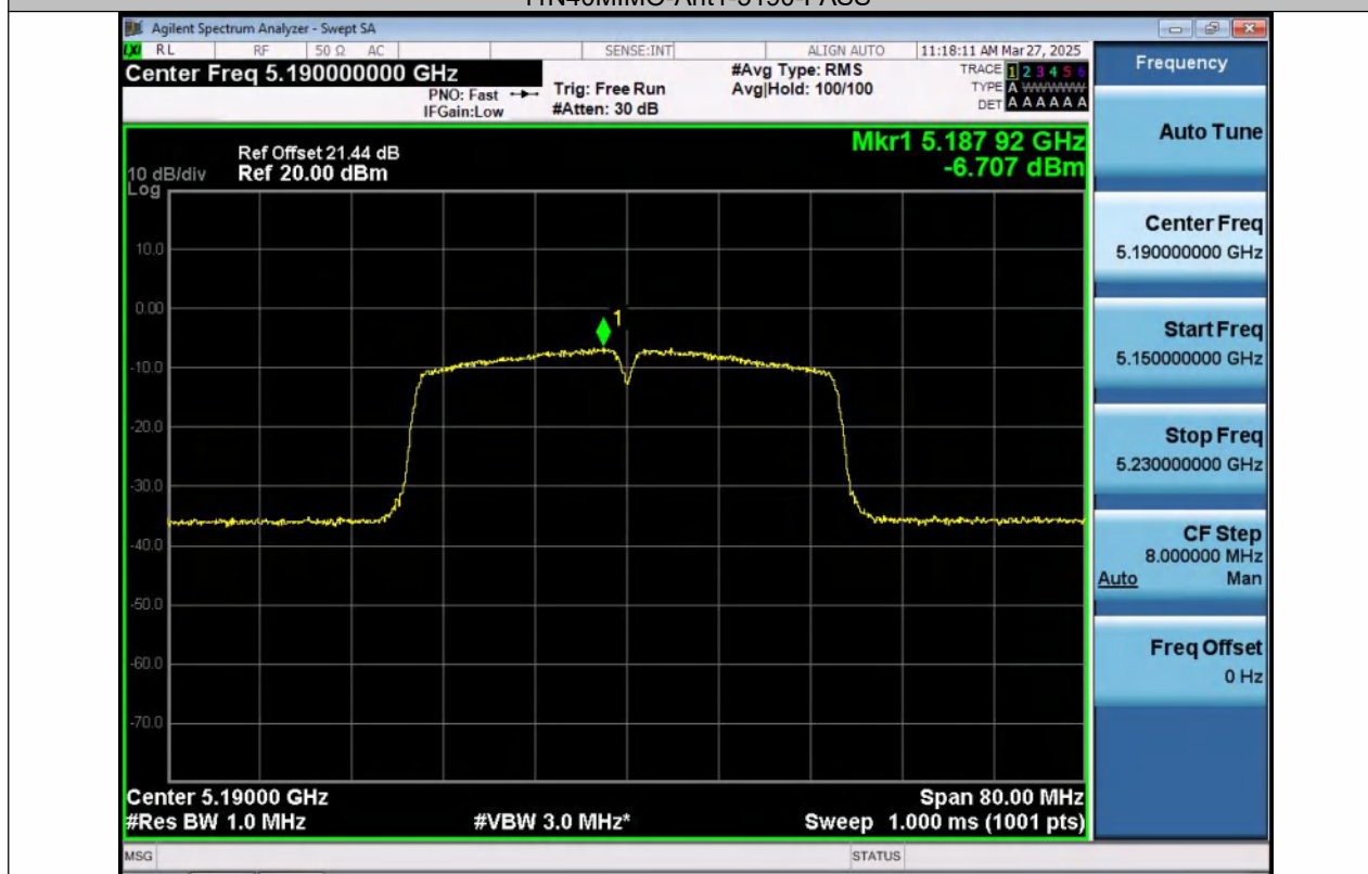
11N40MIMO-Ant2-5190-PASS
