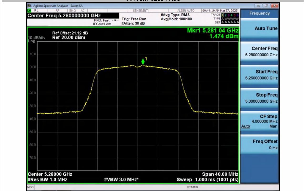
11A-Ant2-5280-PASS
