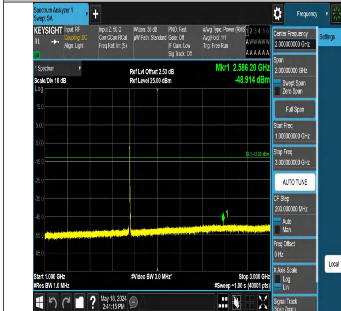
Band4_3MHz_QPSK_20385_1RB#14_1000~3000_1000~3000
