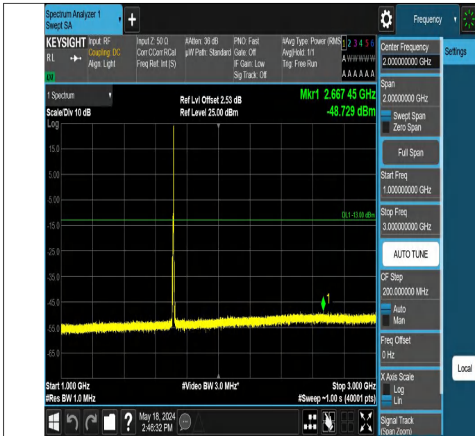
Band4_5MHz_QPSK_19975_1RB#24_1000~3000_1000~3000
