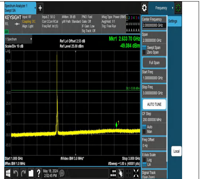
Band4_10MHz_QPSK_20000_1RB#0_1000~3000_1000~3000
