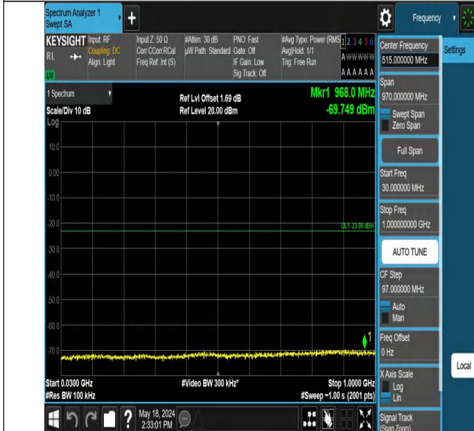
Band4_1.4MHz_QPSK_20393_1RB#0_30~1000_30~1000
