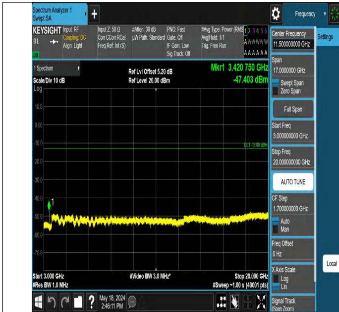
Band4_5MHz_QPSK_19975_1RB#0_3000~20000_3000~20000
