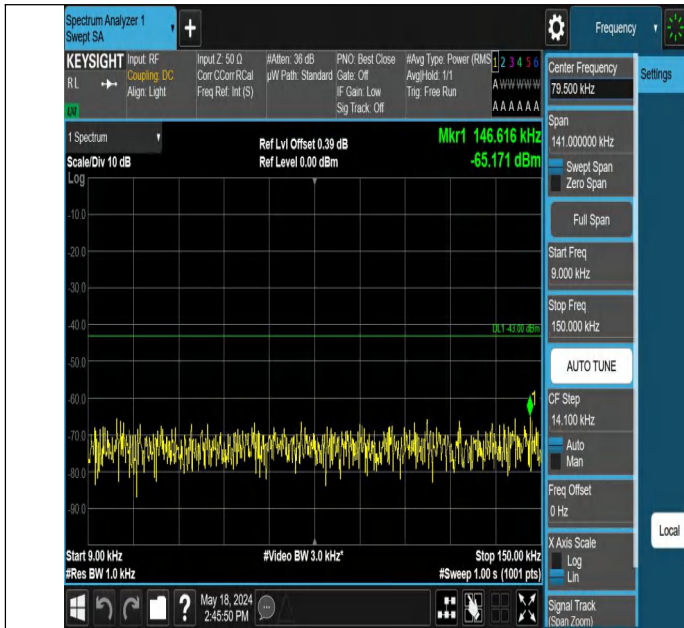
Band4_5MHz_QPSK_19975_1RB#0_0.009~0.15_0.009~0.15
