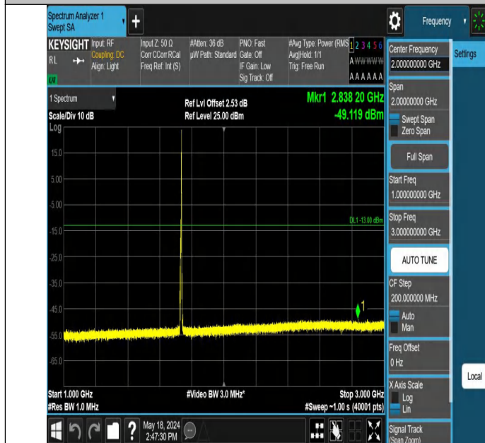
Band4_5MHz_QPSK_20175_1RB#24_1000~3000_1000~3000
