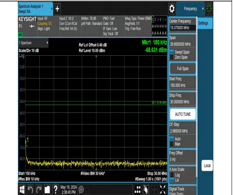
Band4_3MHz_QPSK_19965_1RB#0_0.15~30_0.15~30
