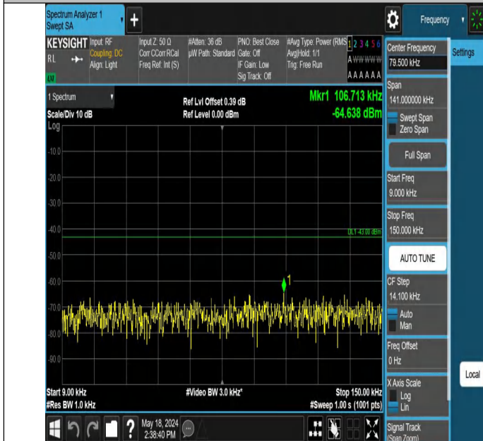
Band4_3MHz_QPSK_19965_1RB#0_0.009~0.15_0.009~0.15
