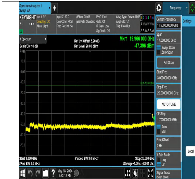
Band4_1.4MHz_QPSK_20393_1RB#0_3000~20000_3000~20000
