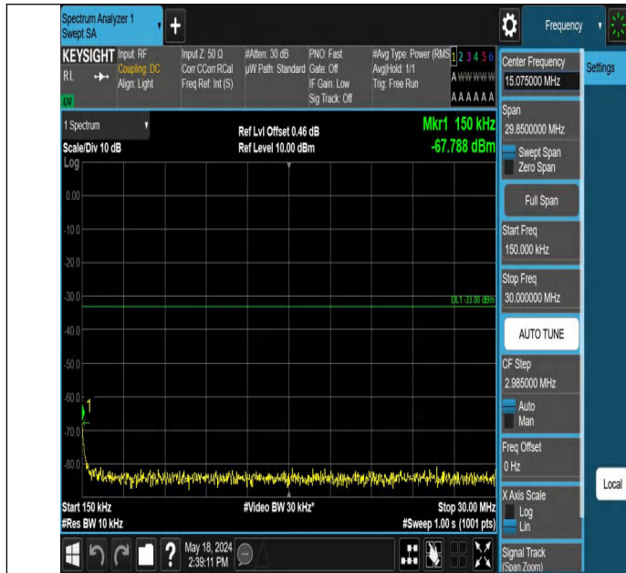
Band4_3MHz_QPSK_19965_1RB#14_0.15~30_0.15~30
