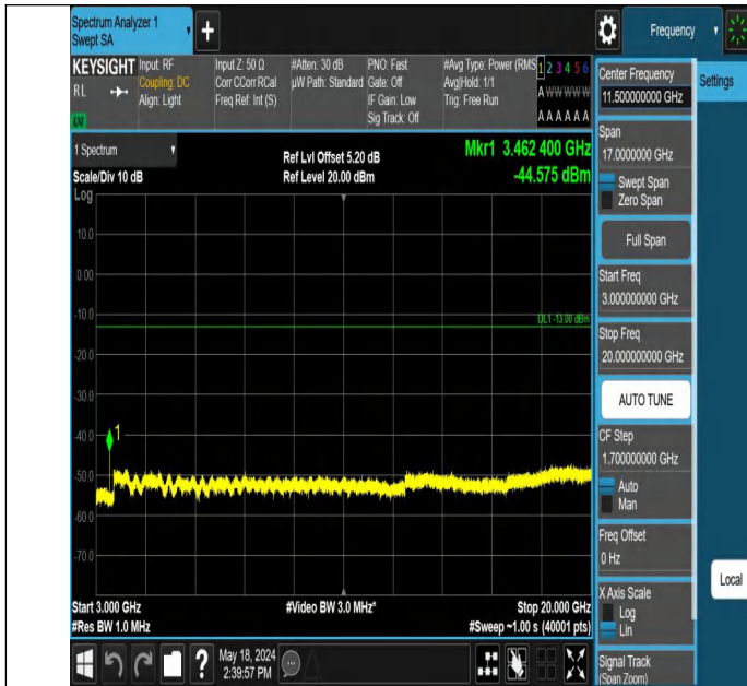
Band3_3MHz_QPSK_20175_1RB#0_3000~20000_3000~20000
