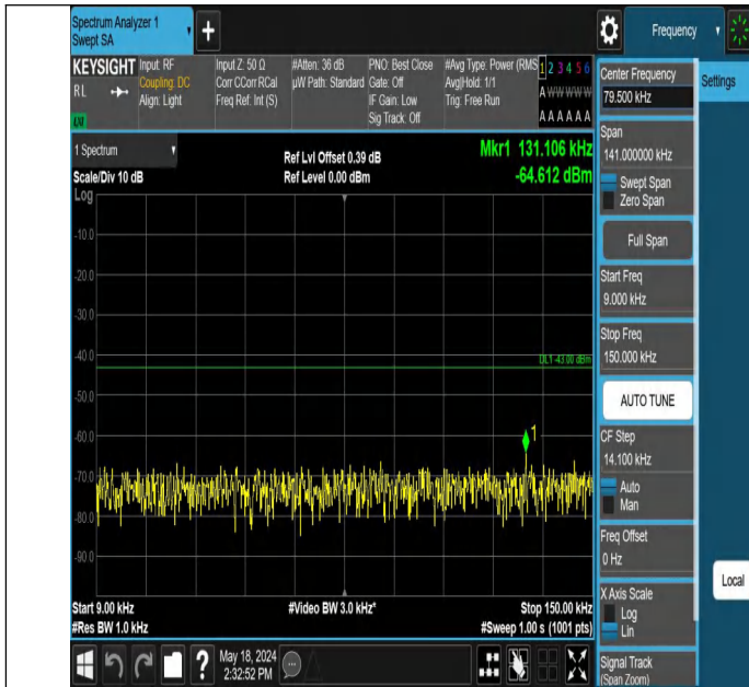
Band4_1.4MHz_QPSK_20393_1RB#0_0.009~0.15_0.009~0.15
