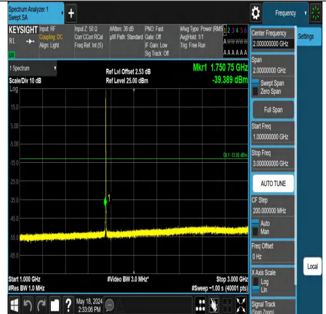
Band4_1.4MHz_QPSK_20393_1RB#0_1000~3000_1000~3000
