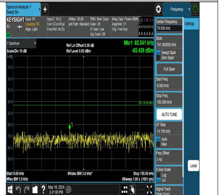
Band4_3MHz_QPSK_20385_1RB#14_0.009~0.15_0.009~0.15
