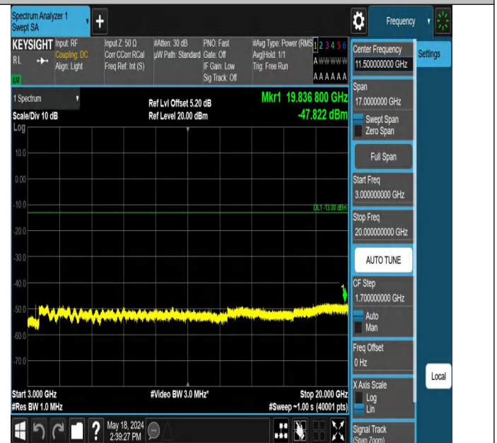
Band4_3MHz_QPSK_19965_1RB#14_3000~20000_3000~20000
