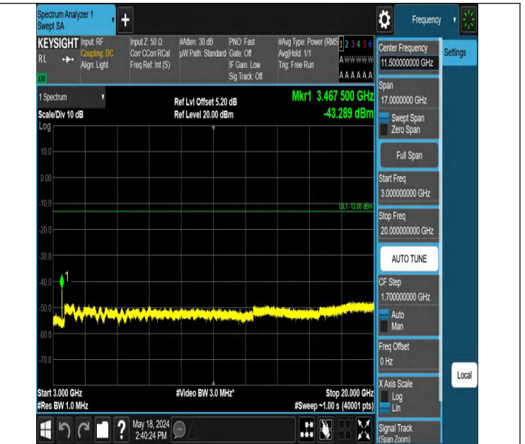
Band4_3MHz_QPSK_20175_1RB#14_3000~20000_3000~20000
