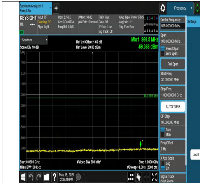
Band4_3MHz_QPSK_19965_1RB#0_30~1000_30~1000
