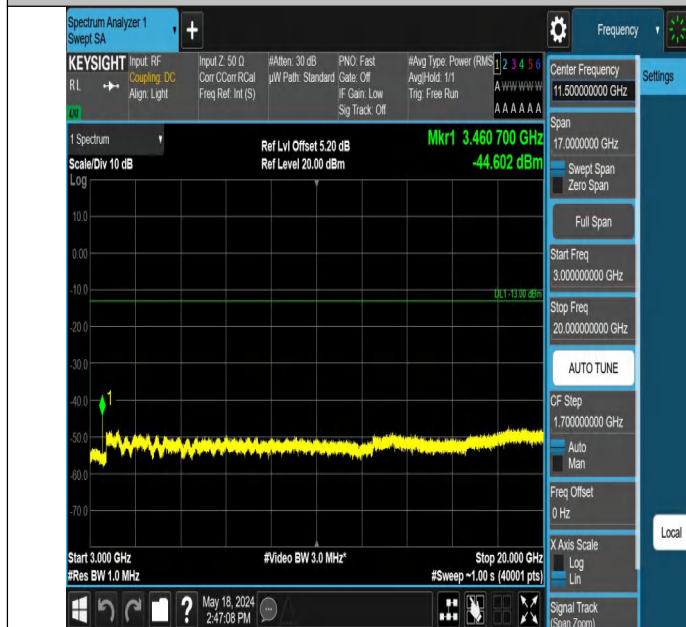
Band4_5MHz_QPSK_20175_1RB#0_3000~20000_3000~20000
