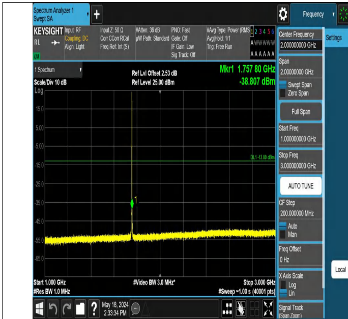
Band4_1.4MHz_QPSK_20393_1RB#5_1000~3000_1000~3000
