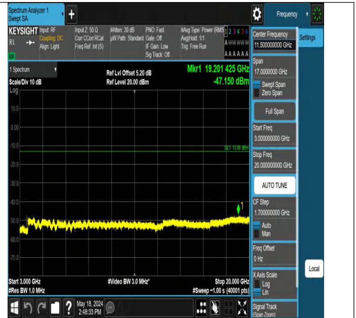
Band4_5MHz_QPSK_20375_1RB#24_3000~20000_3000~20000
