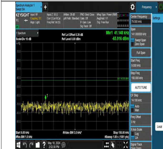
Band4_10MHz_QPSK_20000_1RB#0_0.009~0.15_0.009~0.15
