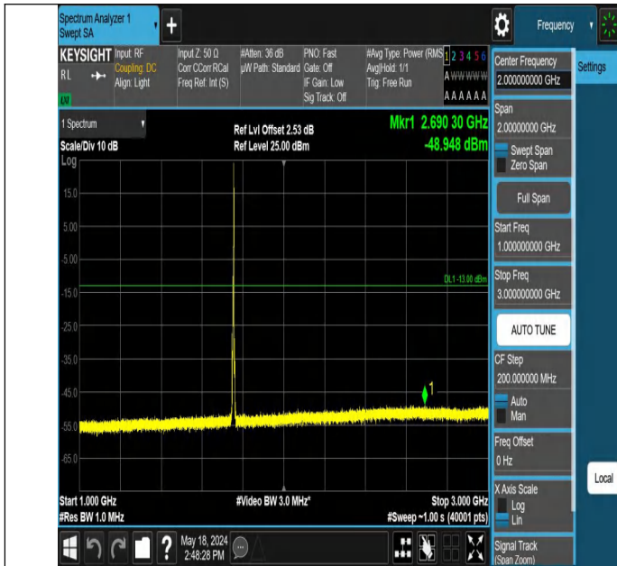
Band4_5MHz_QPSK_20375_1RB#24_1000~3000_1000~3000
