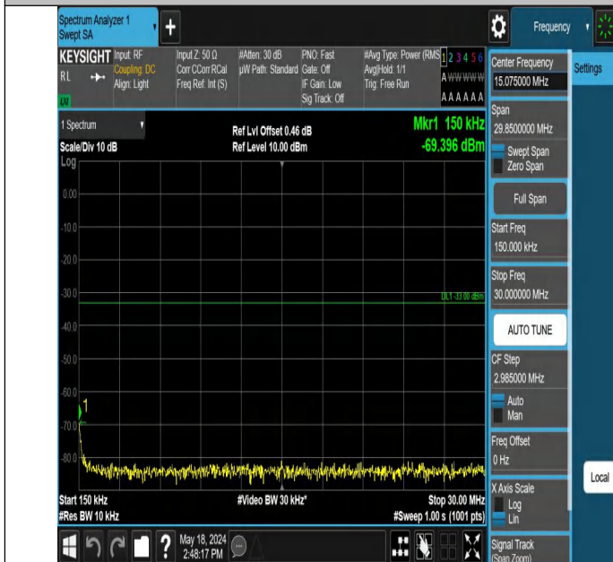
Band4_5MHz_QPSK_20375_1RB#24_0.15~30_0.15~30
