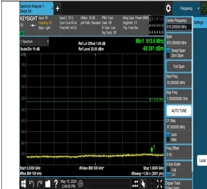
Band4_5MHz_QPSK_19975_1RB#0_30~1000_30~1000
