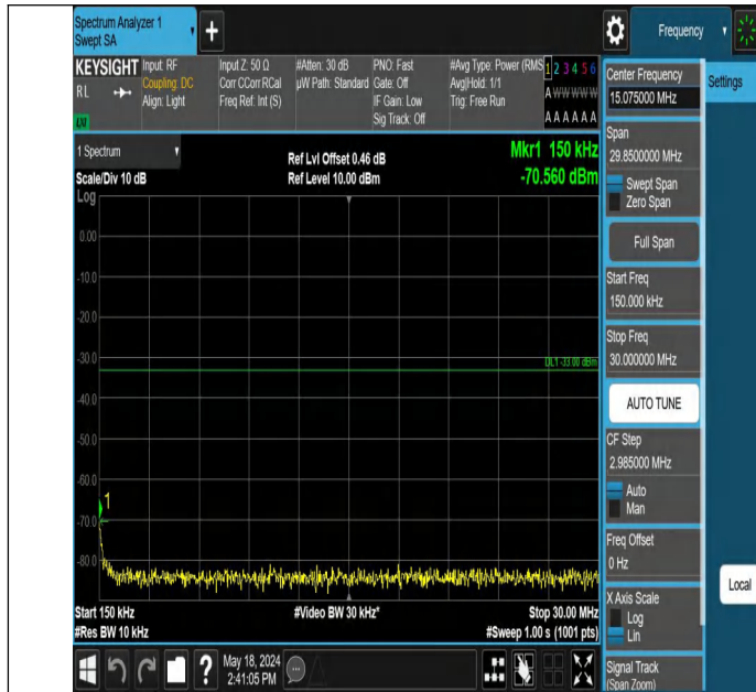
Band4_3MHz_QPSK_20385_1RB#14_0.15~30_0.15~30
