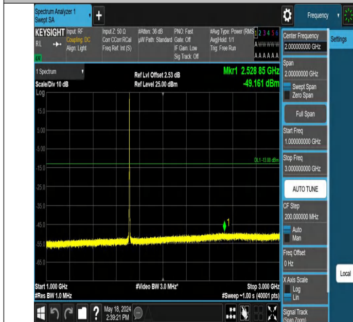
Band4_3MHz_QPSK_19965_1RB#14_1000~3000_1000~3000
