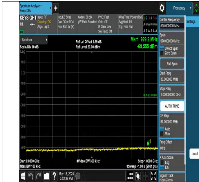
Band4_10MHz_QPSK_20000_1RB#0_30~1000_30~1000
