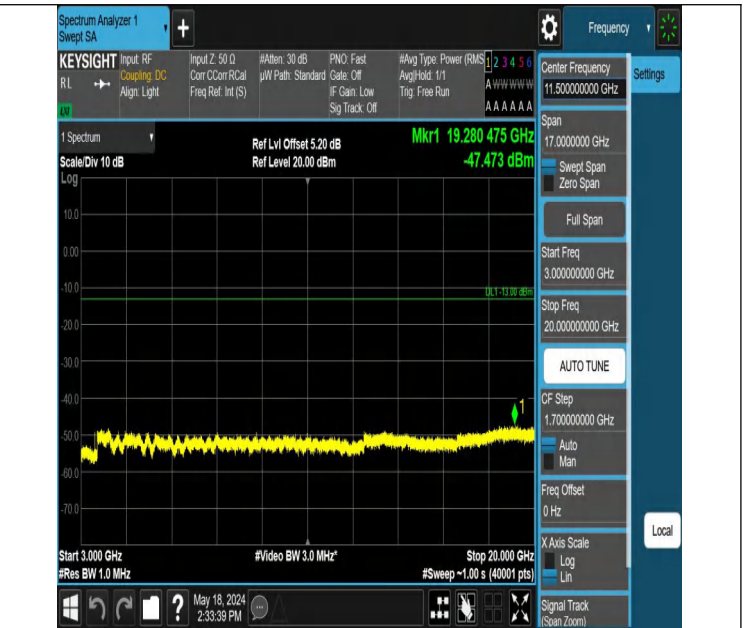
Band4_1.4MHz_QPSK_20393_1RB#5_3000~20000_3000~20000
