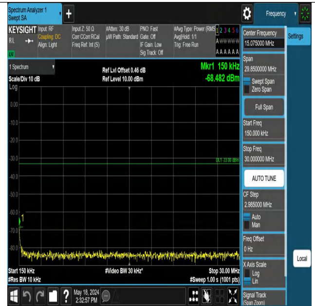
Band4_1.4MHz_QPSK_20393_1RB#0_0.15~30_0.15~30
