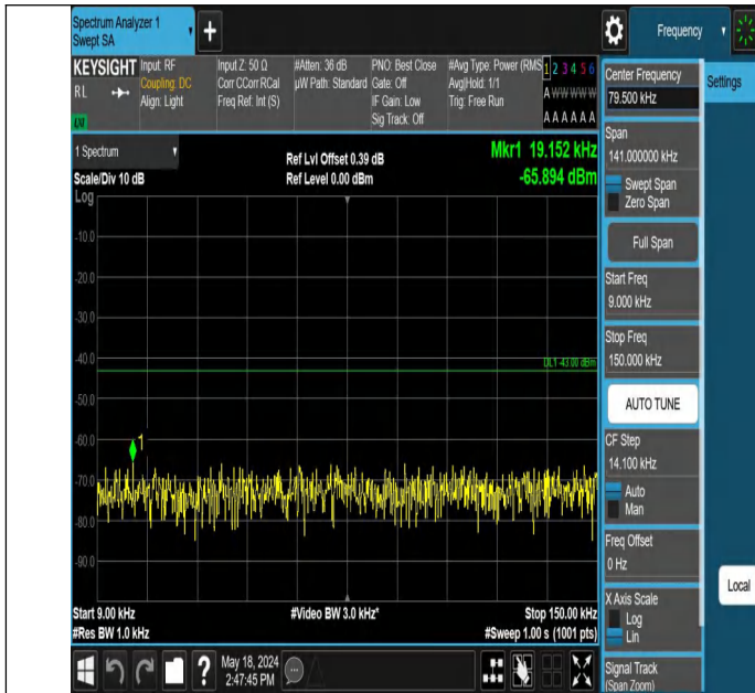
Band4_5MHz_QPSK_20375_1RB#0_0.009~0.15_0.009~0.15
