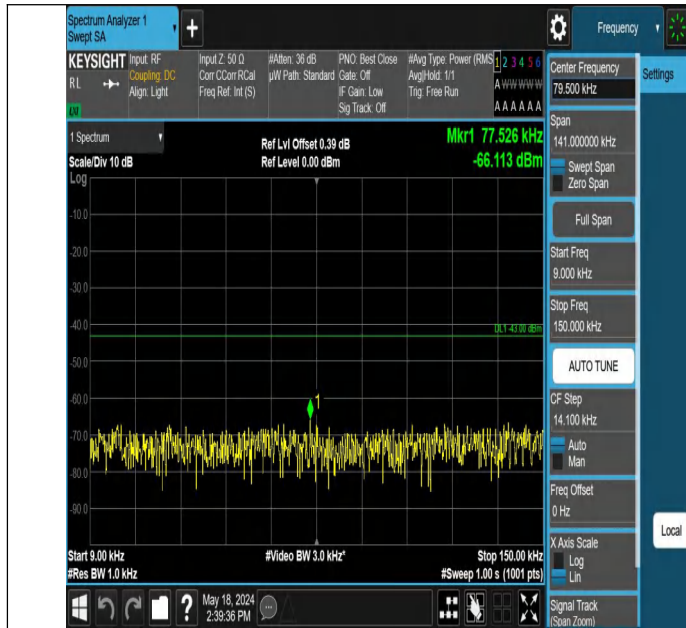
Band4_3MHz_QPSK_20175_1RB#0_0.009~0.15_0.009~0.15
