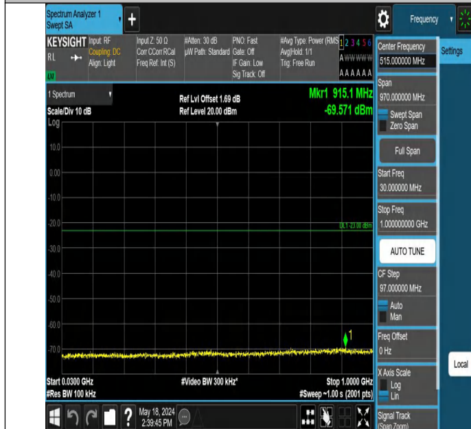
Band4_3MHz_QPSK_20175_1RB#0_30~1000_30~1000
