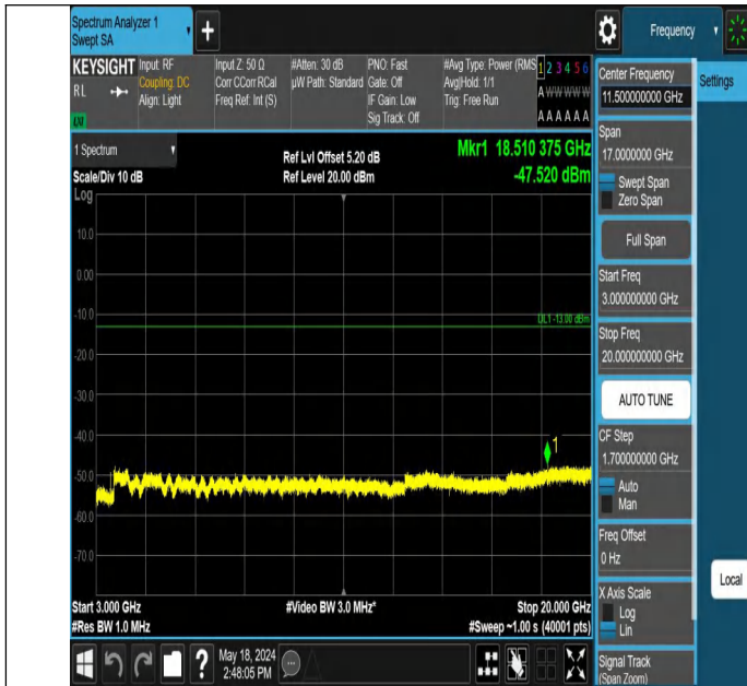
Band4_5MHz_QPSK_20375_1RB#0_3000~20000_3000~20000
