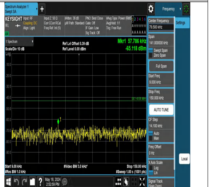
Band4_10MHz_QPSK_20000_1RB#49_0.009~0.15_0.009~0.15
