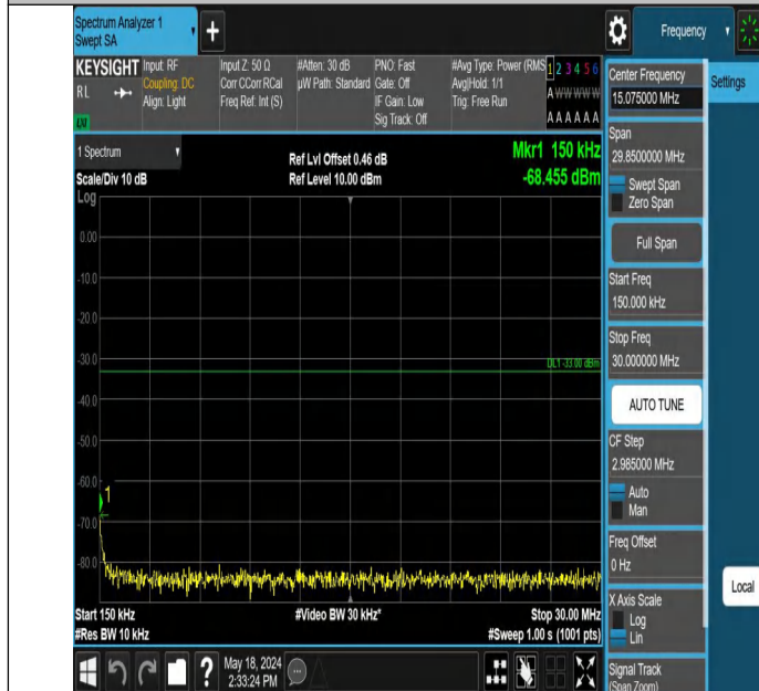
Band4_1.4MHz_QPSK_20393_1RB#5_0.15~30_0.15~30
