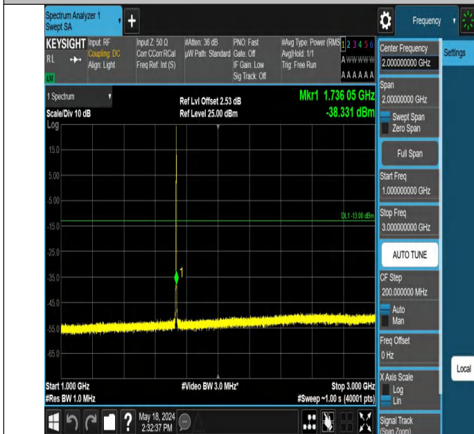
Band4_1.4MHz_QPSK_20175_1RB#5_1000~3000_1000~3000
