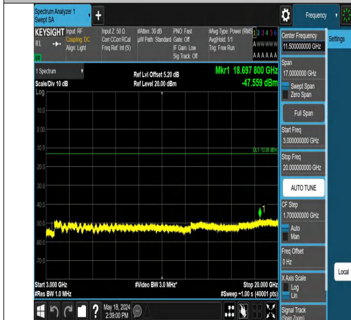
Band4_3MHz_QPSK_19965_1RB#0_3000~20000_3000~20000
