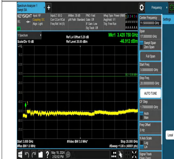
Band4_10MHz_QPSK_20000_1RB#0_3000~20000_3000~20000
