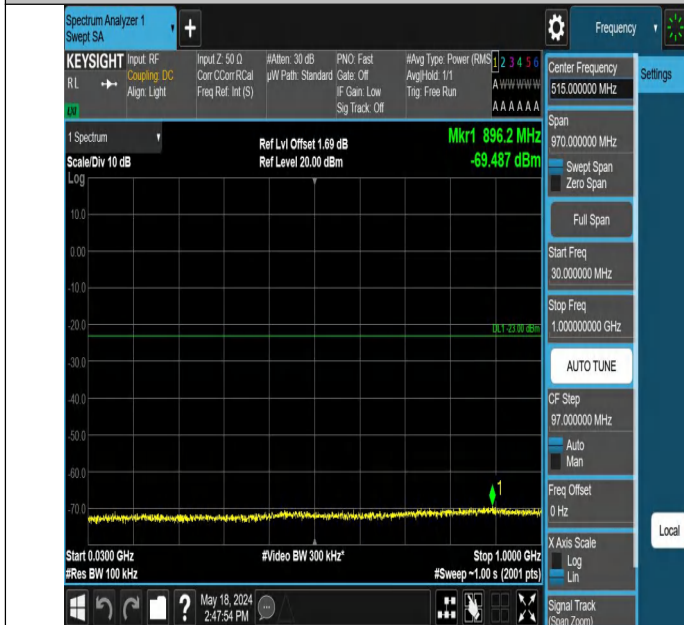
Band4_5MHz_QPSK_20375_1RB#0_30~1000_30~1000
