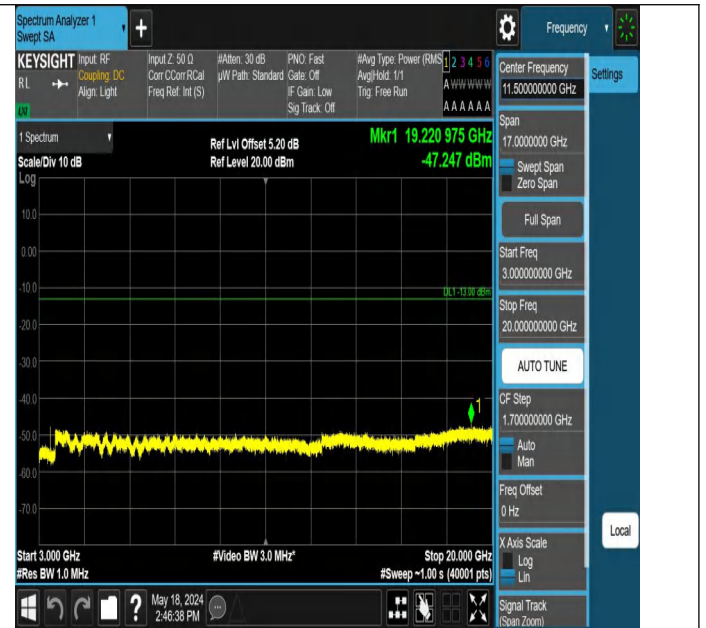
Band4_5MHz_QPSK_19975_1RB#24_3000~20000_3000~20000
