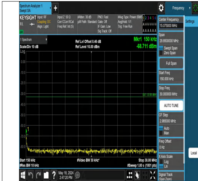
Band4_5MHz_QPSK_20175_1RB#24_0.15~30_0.15~30
