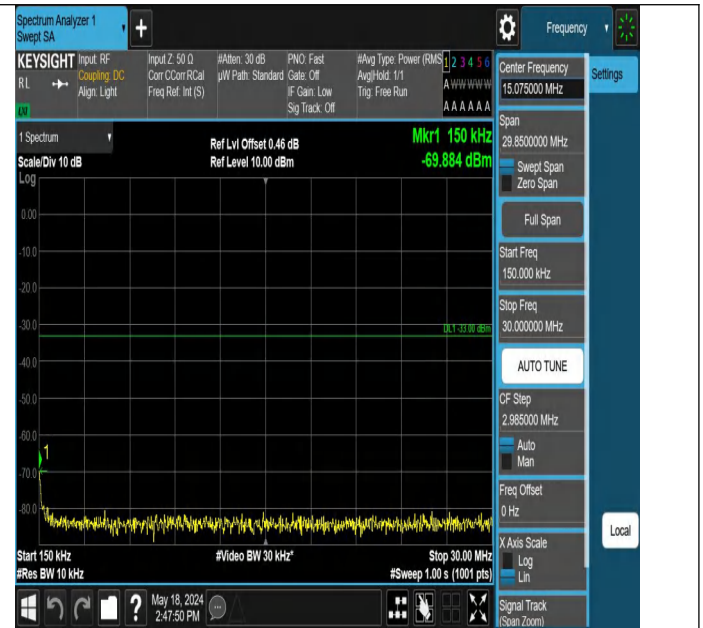
Band4_5MHz_QPSK_20375_1RB#0_0.15~30_0.15~30
