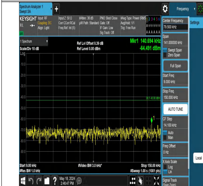
Band4_5MHz_QPSK_20175_1RB#0_0.009~0.15_0.009~0.15
