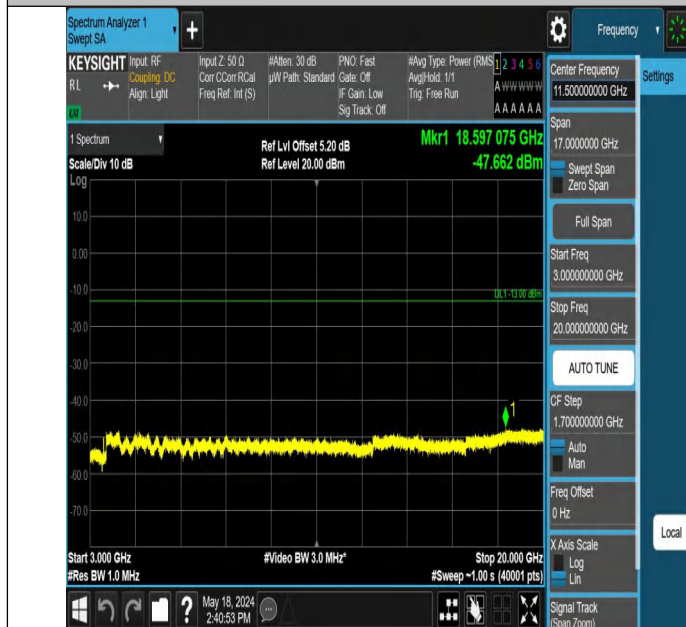
Band4_3MHz_QPSK_20385_1RB#0_3000~20000_3000~20000
