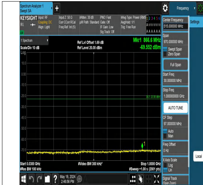
Band4_5MHz_QPSK_20175_1RB#0_30~1000_30~1000
