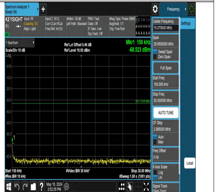
Band4_10MHz_QPSK_20000_1RB#0_0.15~30_0.15~30
