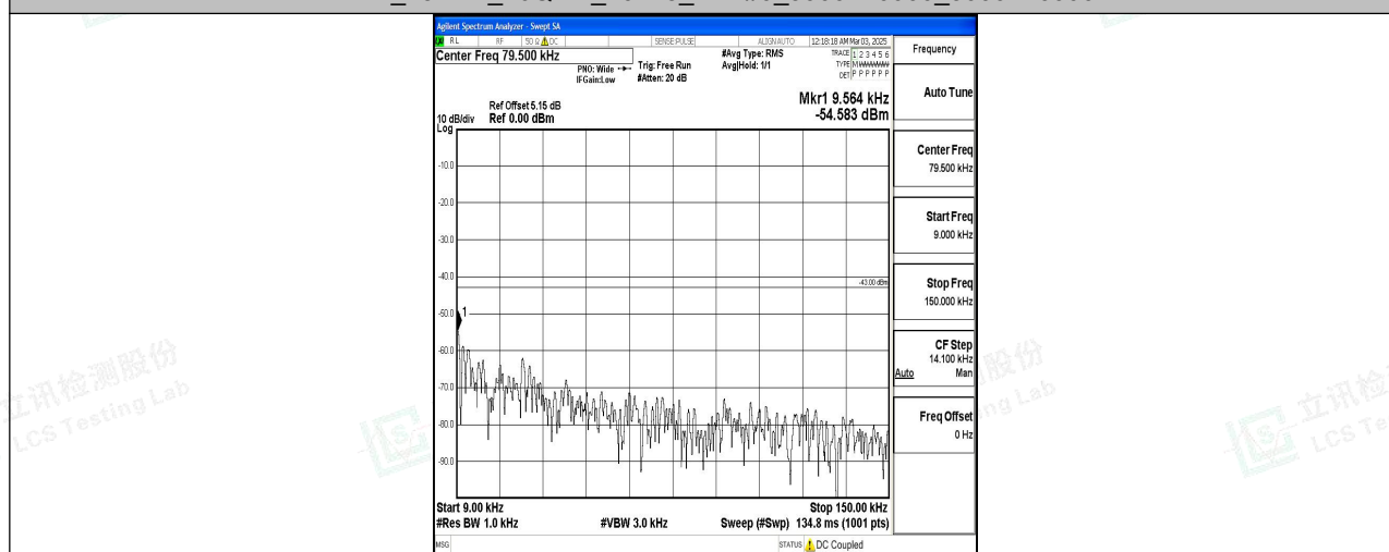
Band4_15MHz_QPSK_20325_1RB#0_0.009~0.15_0.009~0.15
