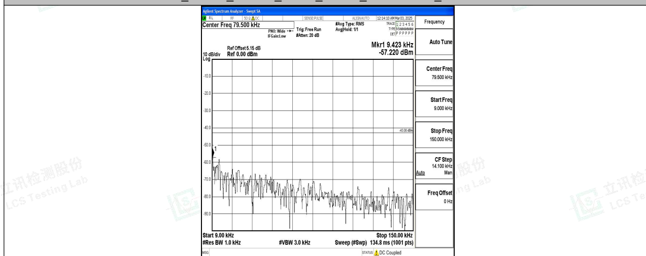
Band4_10MHz_QPSK_20350_1RB#0_0.009~0.15_0.009~0.15
