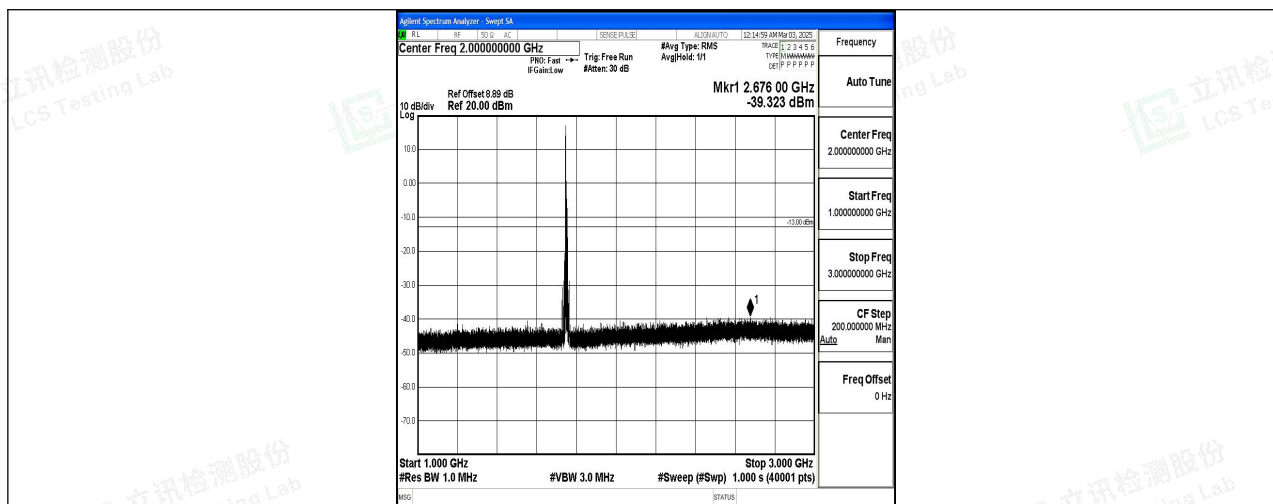
Band4_10MHz_16QAM_20350_1RB#0_1000~3000_1000~3000
