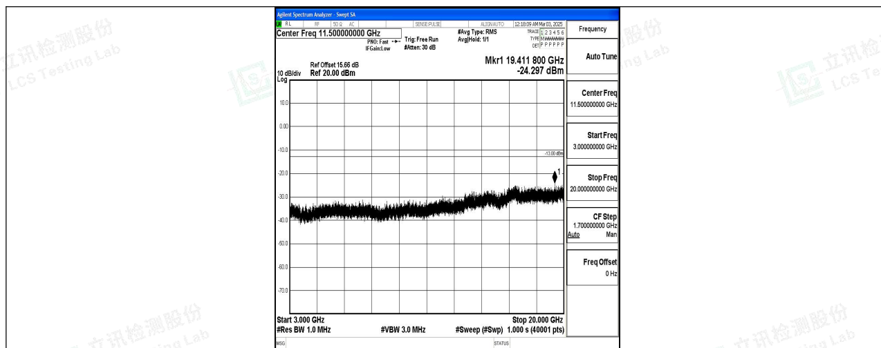
Band4_15MHz_16QAM_20175_1RB#0_3000~20000_3000~20000
