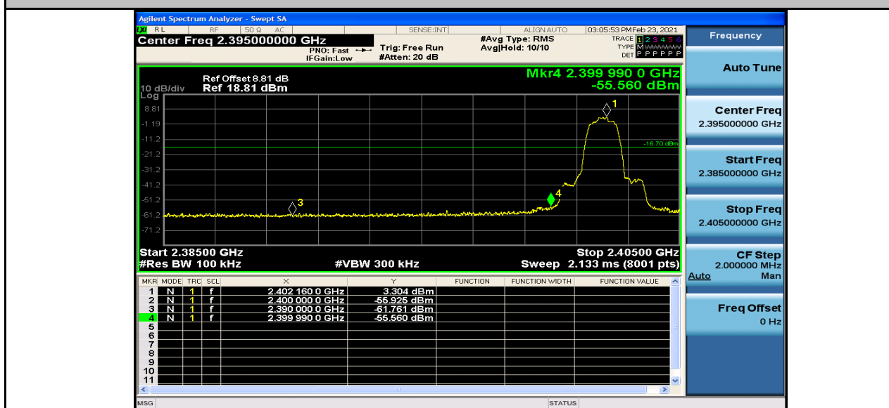
Band-edge for RF Conducted Emissions_2DH5_2480_Hopping On
