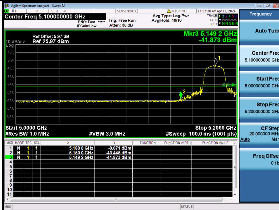
Bandedge_HVNT_ANT1_802_11a_5180
