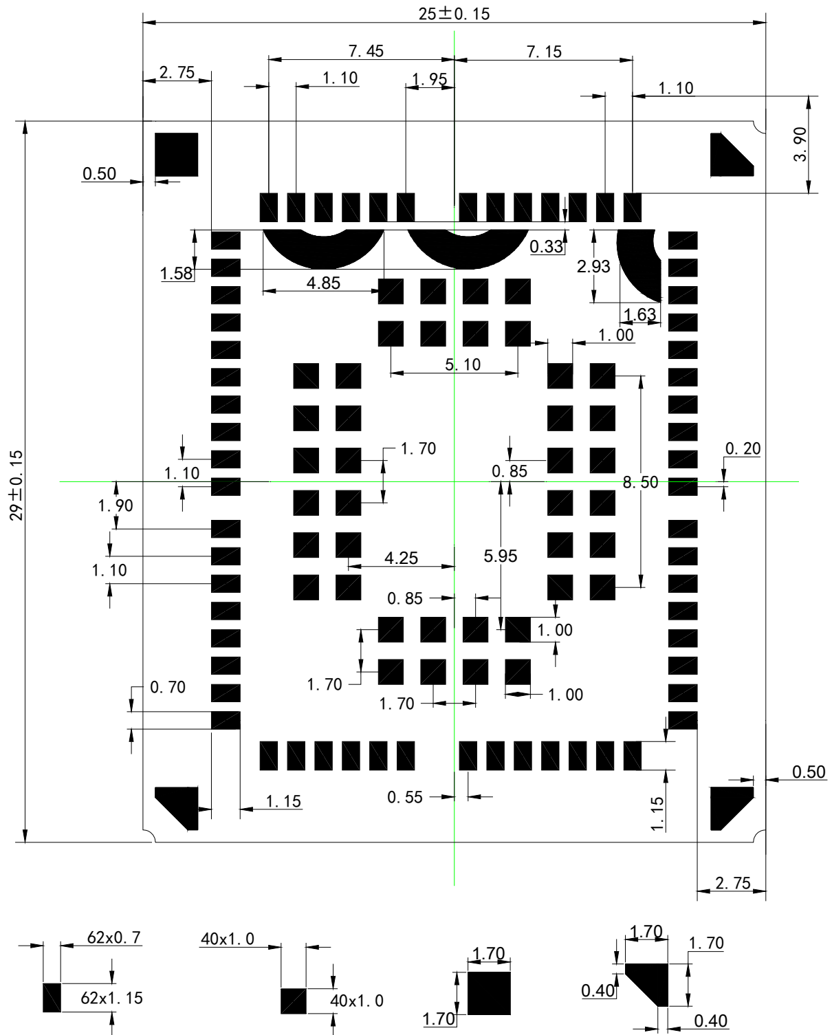
Figure 43: EG91-EX Module Bottom Dimensions (Top View)
