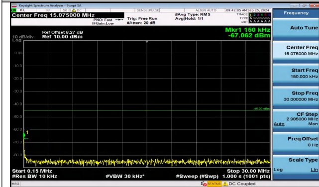
Band38_5MHz_16QAM_38000_1RB#0_0.15~30_0.15~30
