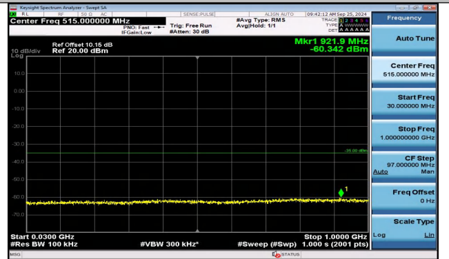
Band38_5MHz_16QAM_38000_1RB#0_30~1000_30~100 0
