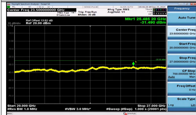
Band38_5MHz_QPSK_38225_1RB#0_20000~27000_20000~27000
