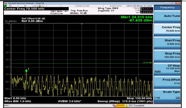
Band38_5MHz_16QAM_38000_1RB#0_0.009~0.15_0.009 ~0.15
