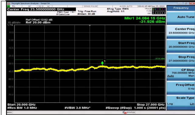
Band38_5MHz_QPSK_38000_1RB#0_20000~27000_200 00~27000
