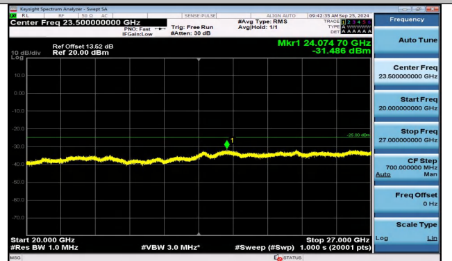
Band38_5MHz_16QAM_38000_1RB#0_20000~27000_20 000~27000
