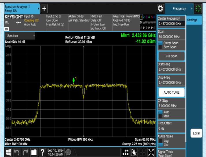
11N40MIMO-Ant2-2437-0~Reference-PASS
