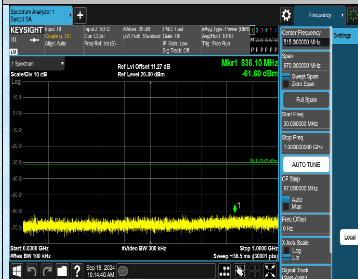
11N40MIMO-Ant2-2437-30~1000-PASS
