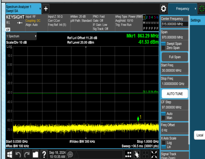
11N40MIMO-Ant2-2422-30~1000-PASS
