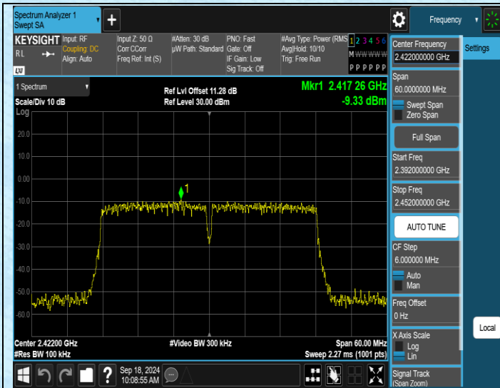
11N40MIMO-Ant1-2422-0~Reference-PASS
