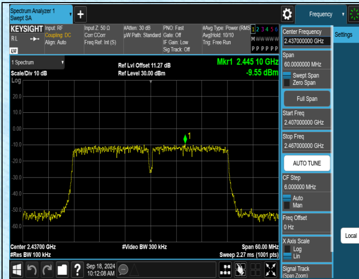
11N40MIMO-Ant1-2437-0~Reference-PASS
