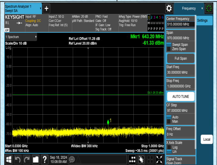
11N40MIMO-Ant1-2422-30~1000-PASS
