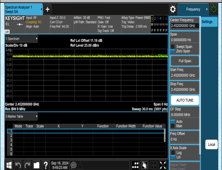
NTNV-11N40SISO-Ant2-2452
