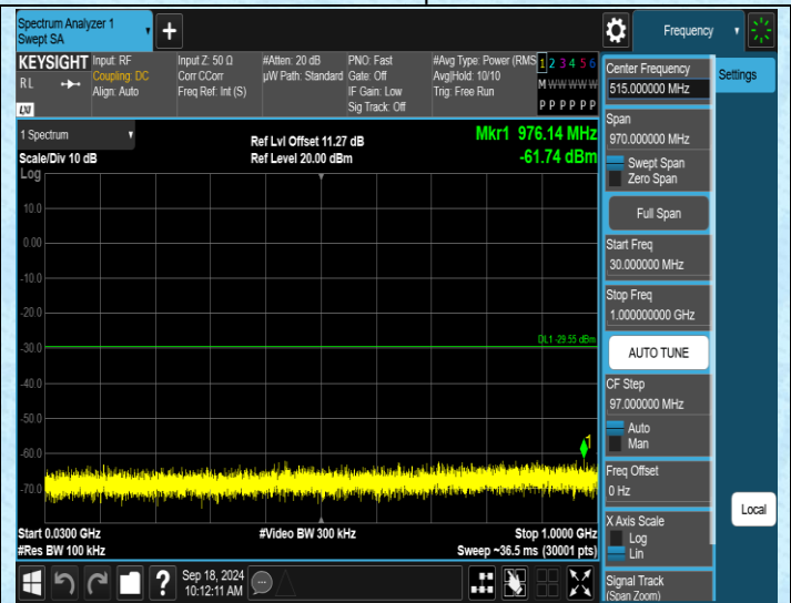
11N40MIMO-Ant1-2437-30~1000-PASS
