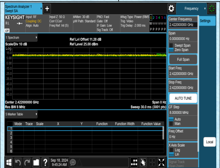
NTNV-11N40SISO-Ant2-2422
