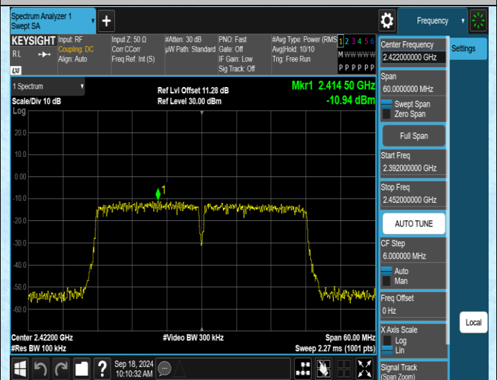
11N40MIMO-Ant2-2422-0~Reference-PASS
