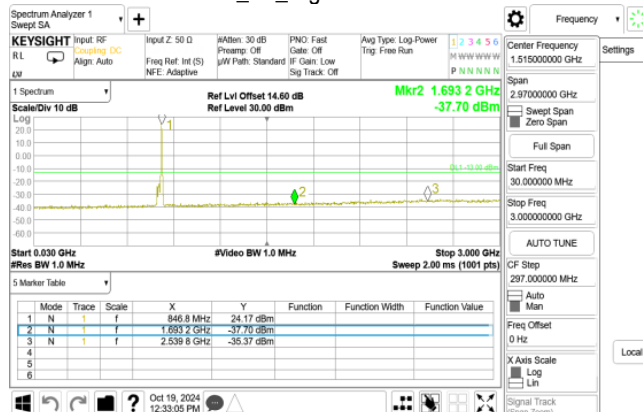
HSDPA_B5_HighCH4233-846.6
