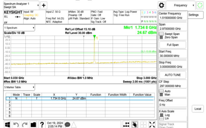
WCDMA_B4_MidCH1413-1732.6
