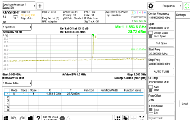
WCDMA_B2_LowCH9262-1852.4
