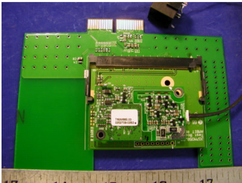
Set up – Board View
