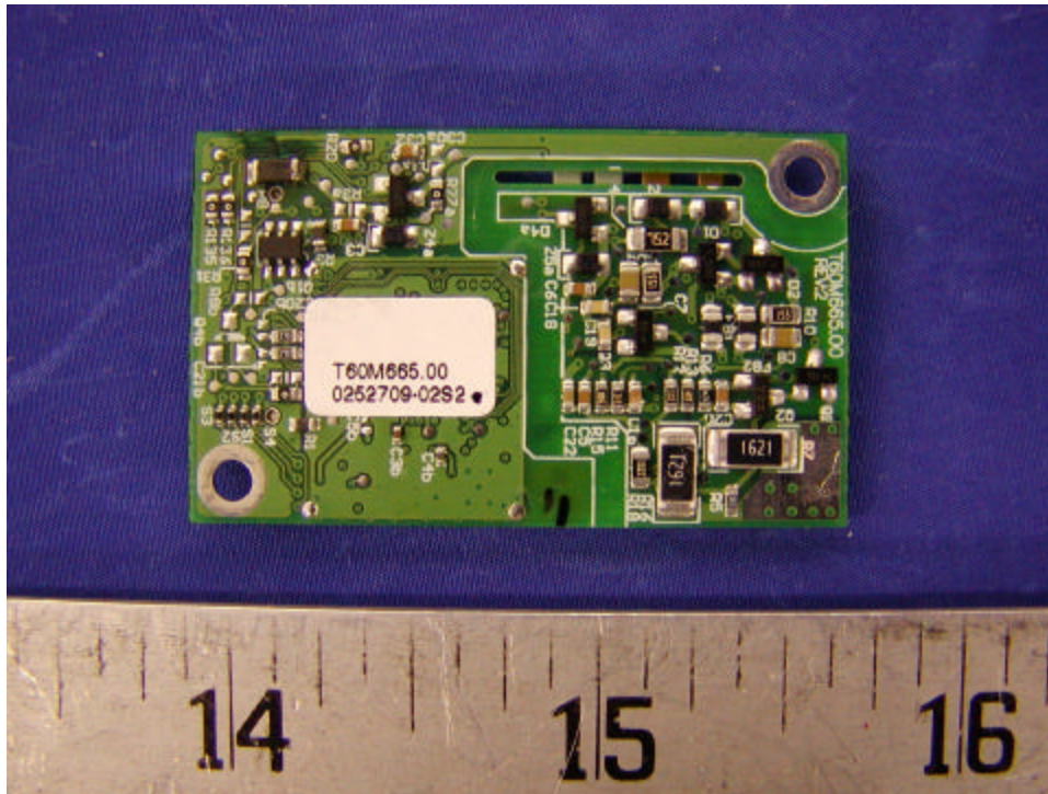
EUT – Side B View
