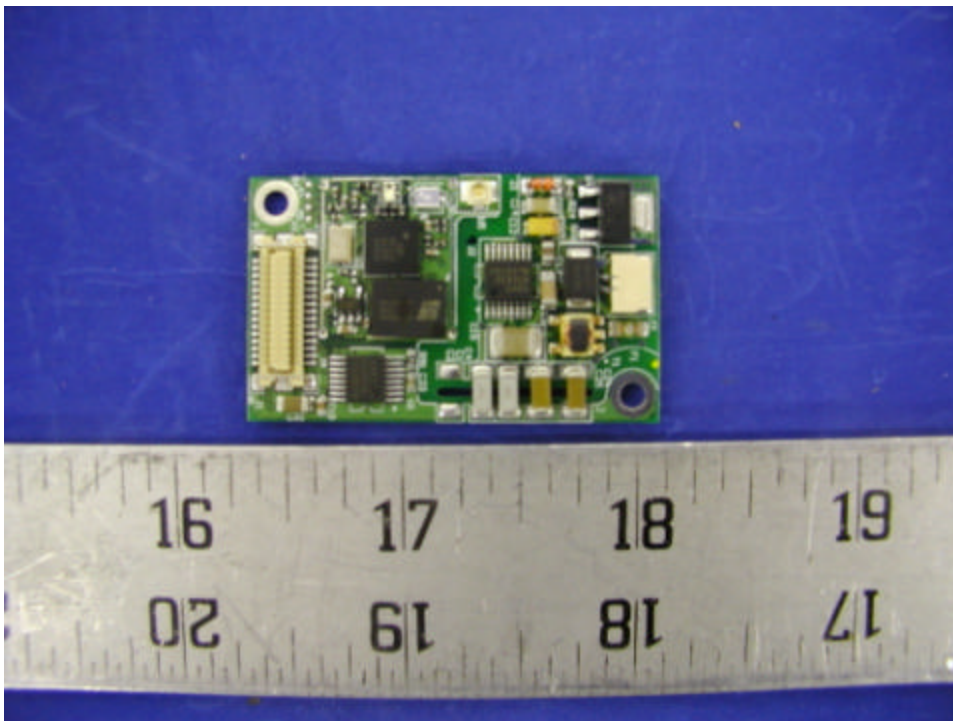
EUT – Side A View, Shield off
