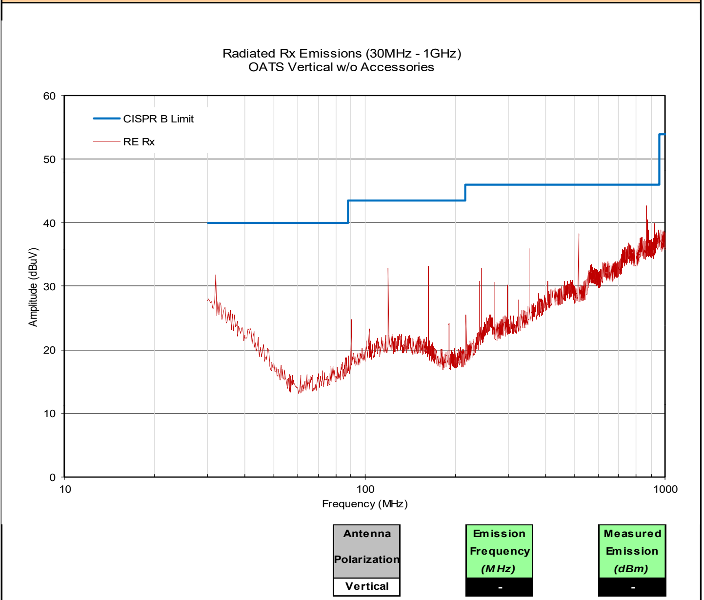
Plot 11.4 – Radiated Spurious Emissions OATS, 30 - 1000MHz, without Accessories, Vertical
