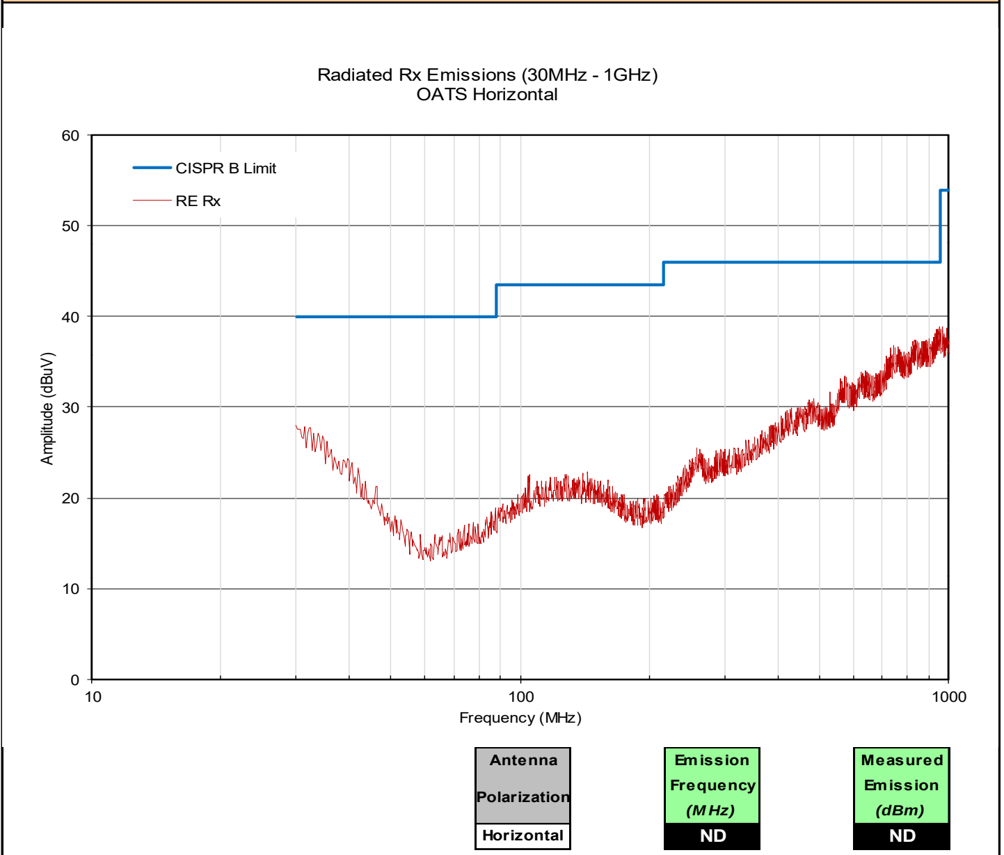
Plot 12.3– Radiated Spurious Emissions OATS, 30 - 1000MHz, Horizontal
