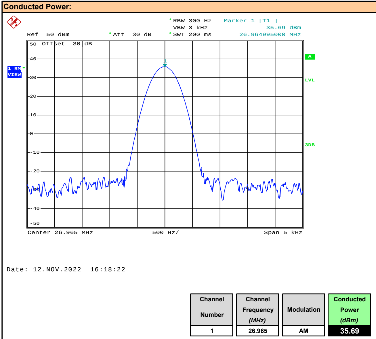
Plot 7.1 – Conducted Output Power, Channel 1, AM
