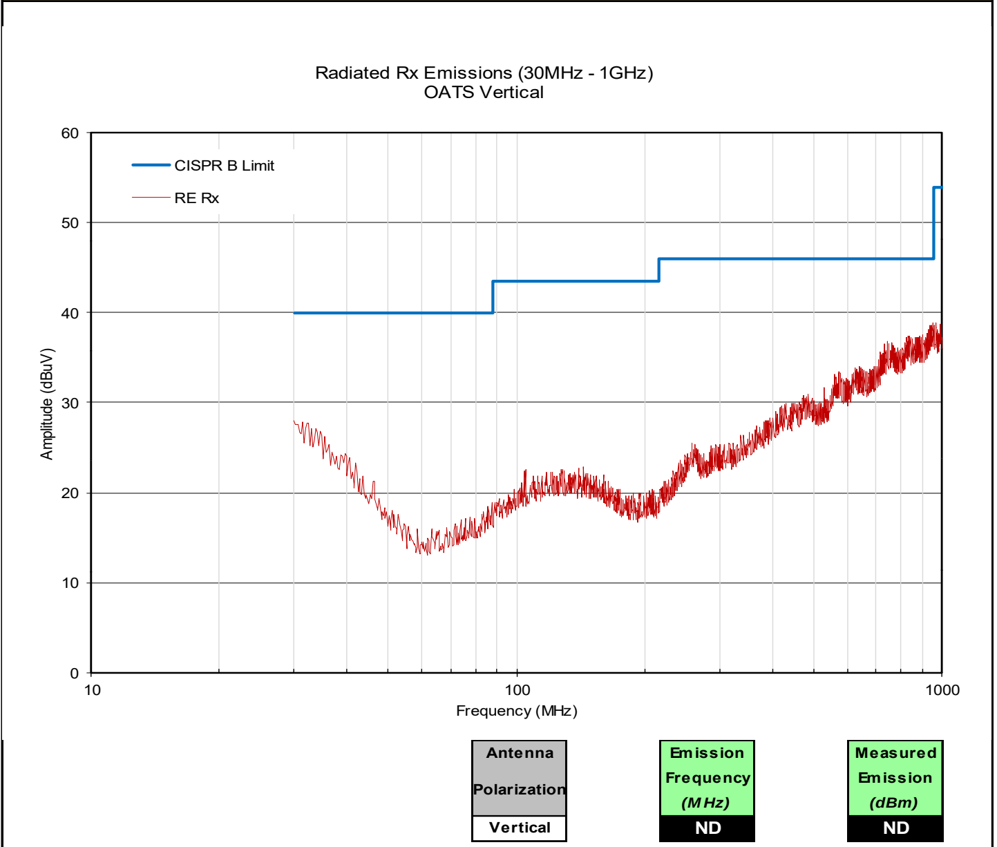
Plot 12.4– Radiated Spurious Emissions OATS, 30 - 1000MHz, Vertical
