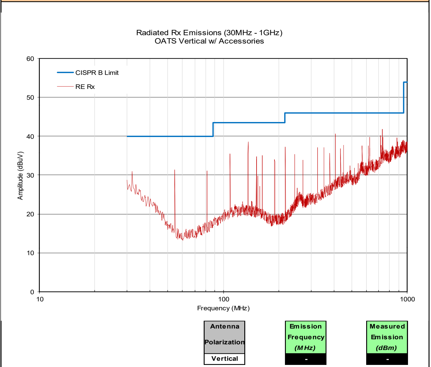
Plot 11.8 – Radiated Spurious Emissions OATS, 30 - 1000MHz, with Accessories, Vertical
