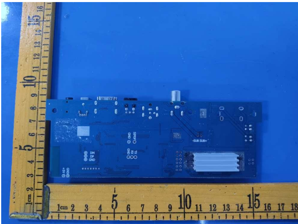
Internal view of unit (Model:D21)
