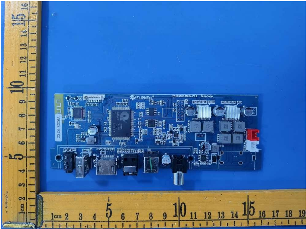
Internal view of unit (Model:D21)
