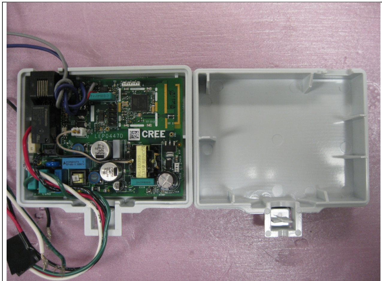
Top Side of Relay Board In Enclosure (CIF-10V-CWC-SNSR)
