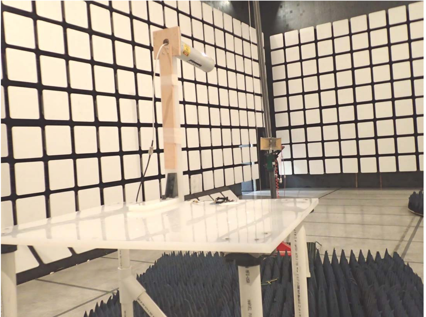
Radiated Emissions @ 3 m, Orthogonal Position 2 EUT with 15.0 dBi Yagi Antenna
