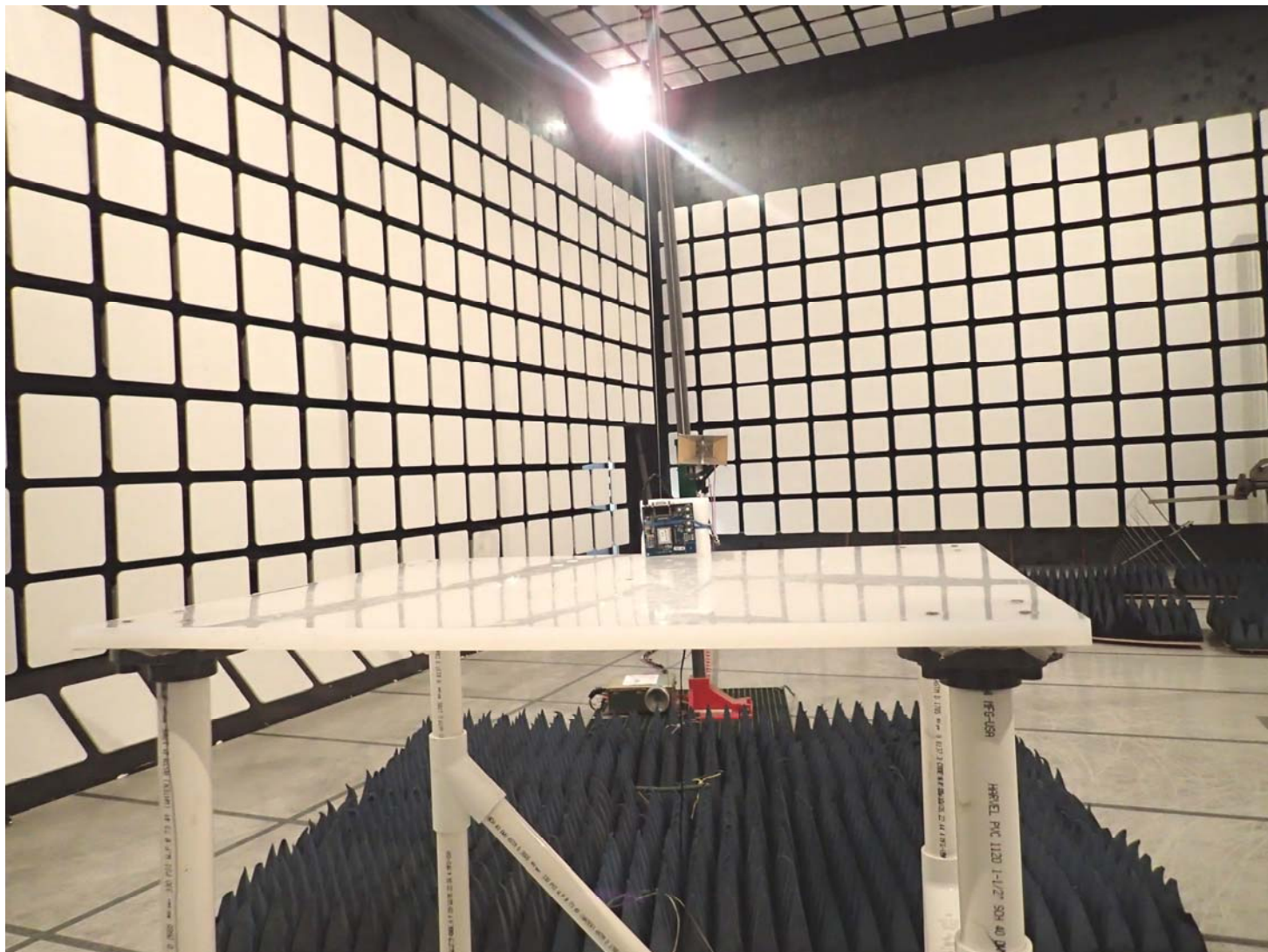
Radiated Emissions @ 3 m, Orthogonal Position 1 EUT with 1.5 dBi Integrated Wire Antenna
