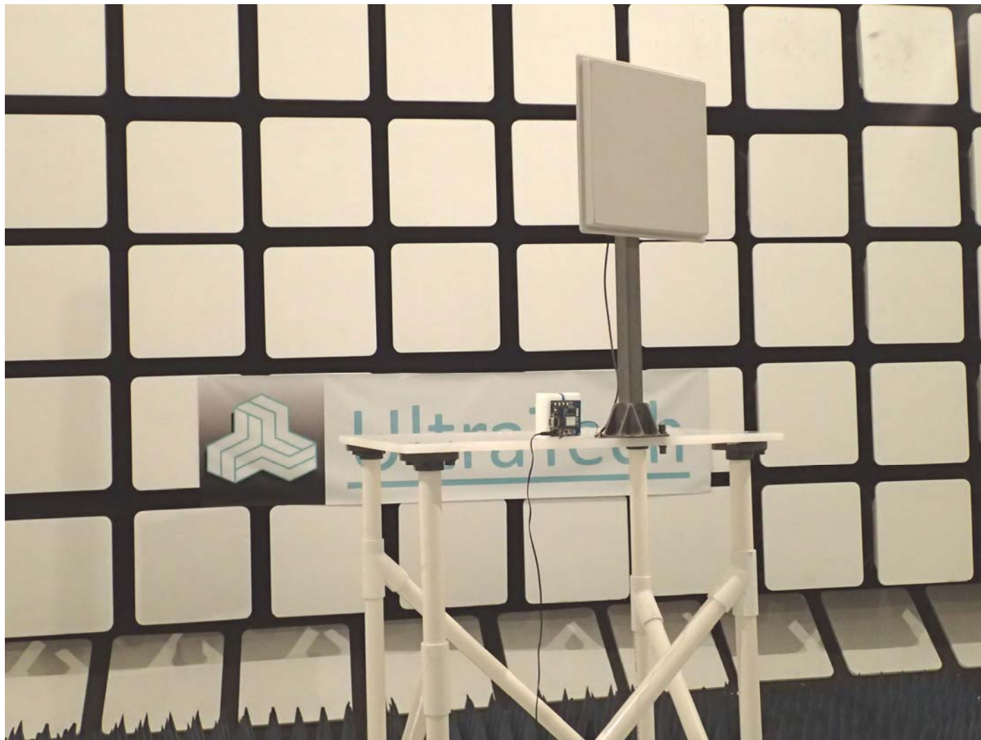
Radiated Emissions @ 3 m, Orthogonal Position 1 EUT with 19.0 dBi Flat Panel Antenna
