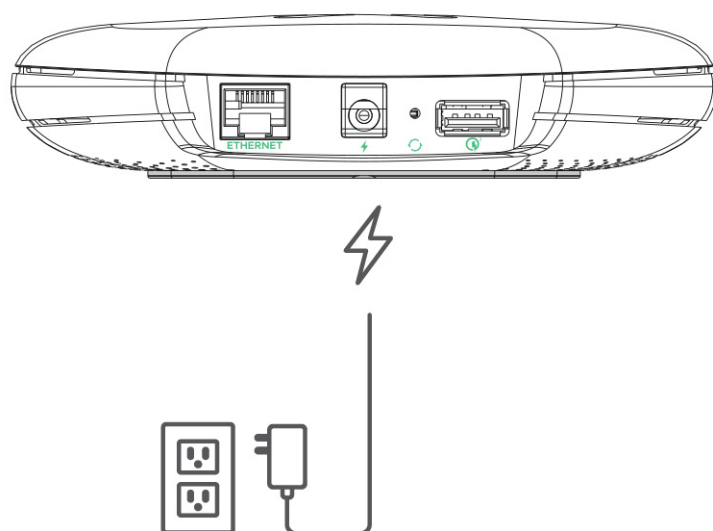
Figure 3 WSR30 Back Panel
