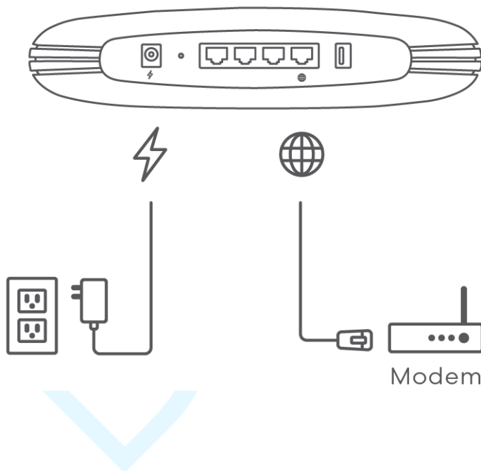
Figure 1 WSQ60/WSQ50 Rear Panel
