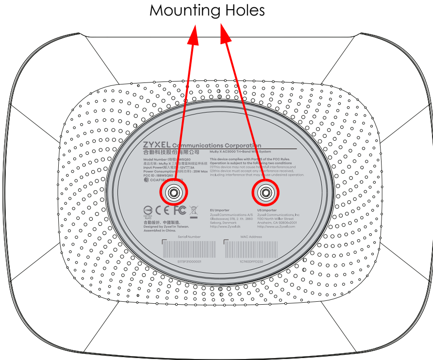
Figure 4 WSQ50 Mounting Holes
