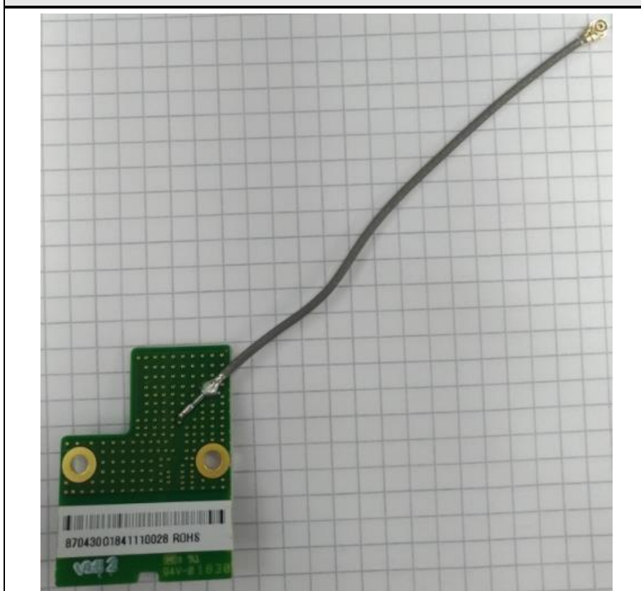
BT LR antenna board bottom
