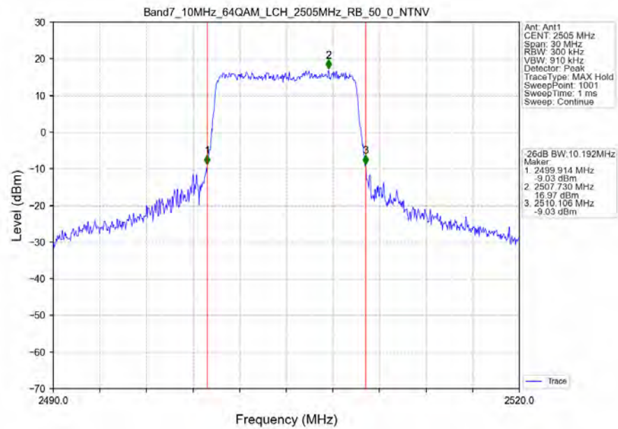
Band7_10MHz_64QAM_LCH_2505MHz_RB_50_0_NTNV
