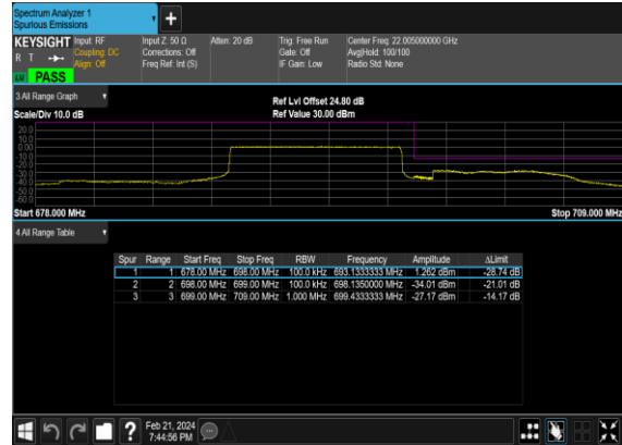
N71(10M)_DFT-s- OFDM_QPSK_Outer_Full_High_CH
