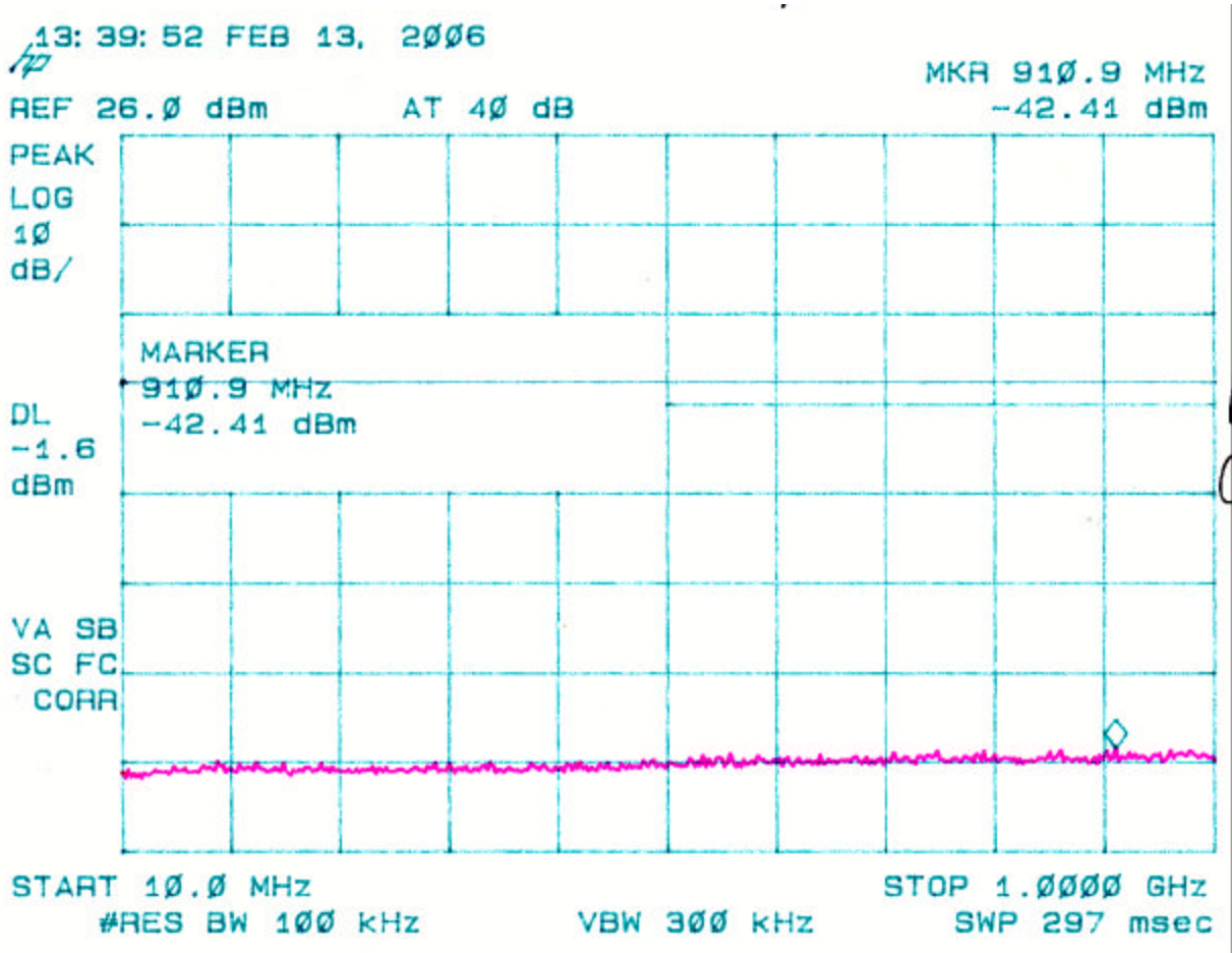
Figure 4i Antenna Conducted Spurious Emissions 15.247(c) High
