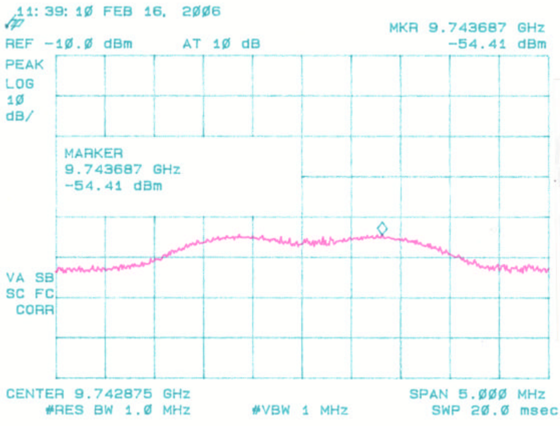
Figure 4b - 4 Peak Radiated Spurious Emission 15.247(c) Mid – Parabolic Dish
