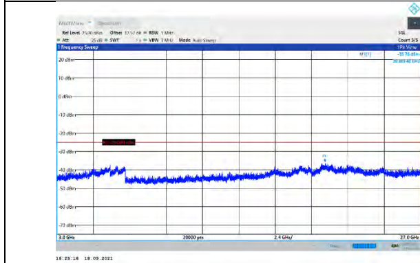
CA_38C-20MHz-20MHz-16QAM-16QAM-37952-38150-1RB#0-0RB#0-3000~27000MHz
