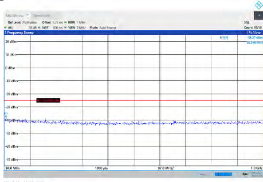
CA_7C-20MHz-20MHz-QPSK-QPSK-20850-21048-1RB#99-1RB#0-30~1000MHz
