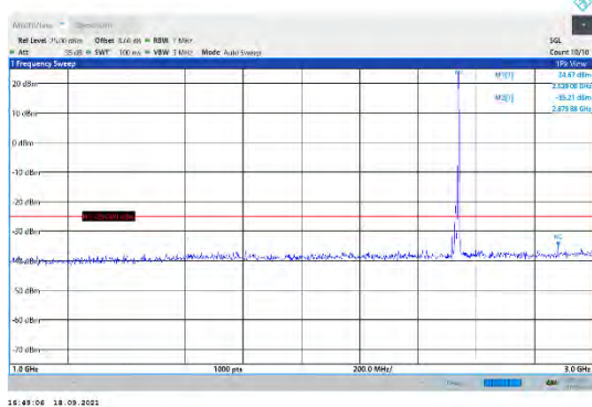
CA_7C-20MHz-20MHz-16QAM-16QAM-20850-21048-0RB#0-1RB#99-1000~3000MHz
