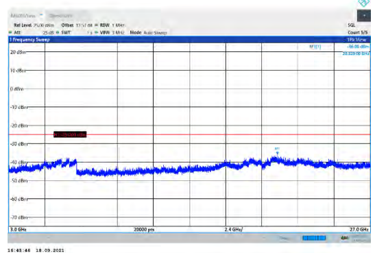
CA_7C-20MHz-20MHz-16QAM-16QAM-20850-21048-1RB#0-0RB#0-3000~27000MHz
