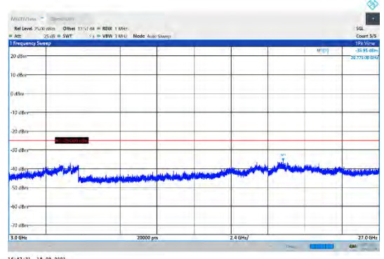
CA_7C-20MHz-20MHz-16QAM-16QAM-20850-21048-1RB#99-1RB#0-3000~27000MHz
